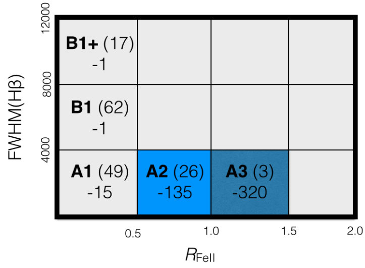
Figure 6: Average shift of [\text{OIII}]\lambda 5007 (negative is blueshift) for spectral types in the optical plane of E1. Numbers in parentheses indicate sources in each bin, with the dataset available to us in late 2001.
