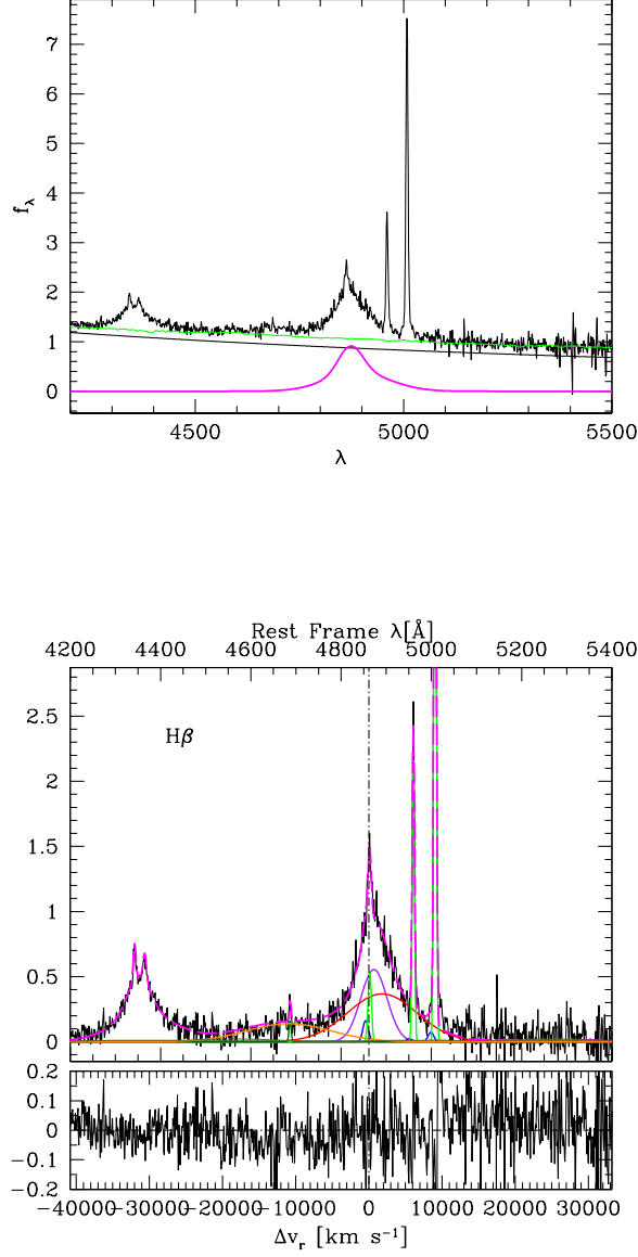
Figure 3: Top: continuum placement for source SDSS J034106.75+004609.9. The black line traces the featureless continuum; the green line traces the total continuum that includes a contribution from the host galaxy (whose presence is made manifest by the Mg Ib band visible in the spectrum). There is no significant FeII emission. The magenta line traces the cleaned H\beta broad profile. Bottom: H\beta profile analysis. The excess on the blue side of H\beta can be explained by significant HeII \lambda 4686 VBC emission. H\beta and H\gamma are consistently fit with the same BC and VBC parameters (the BC and VBC (red) decomposition is shown for H\beta only).
