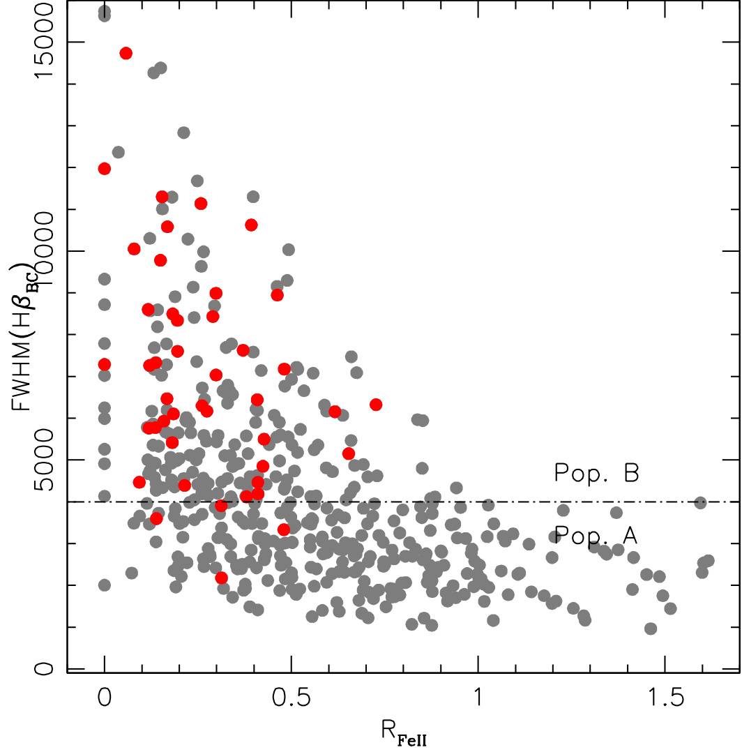
Figure 4: The 4DE1 optical plane involving the width of \text{H}\beta and the strength of optical FeII. Horizontal line marks the boundary between population A (lower) and B (upper) sources. Source occupation is shown for the 470 brightest SDSS-DR5 quasars ( z < 0.75 ) with highest s/n SDSS spectra Zamfir et al. (2008). Grey and red dots represent RQ and lobe dominated LD RL quasars. The latter show a strong preference for the Population B zone.
