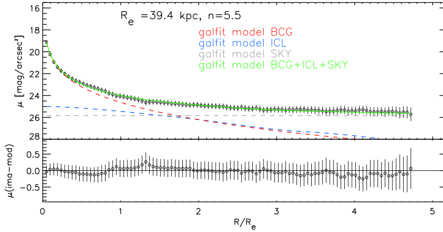
Figure A1. galfit fit (green solid line) of the BCG surface brightness profile in the F814W filter. The dashed lines highlight the best matching radial profiles for the sky background (grey line), the ICL (blue line) and the central galaxy (red line).
