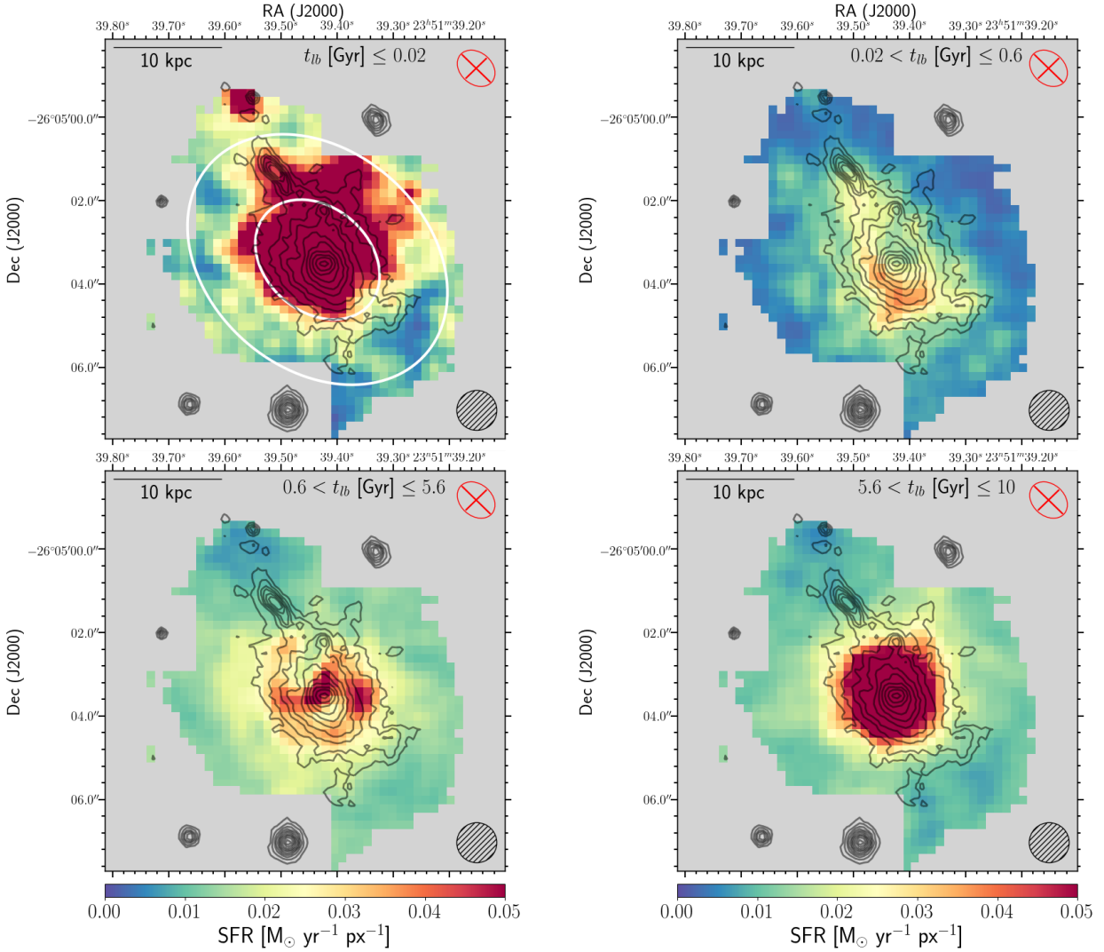
Figure 3. SINOPSIS SFR density maps of the Abell 2667 BCG in the look-back time ( t_{lb} ) intervals t_{lb}[\text{Gyr}] \leq 0.02 (top left), 0.02 < t_{lb}[\text{Gyr}] \leq 0.6 (top right), 0.6 < t_{lb}[\text{Gyr}] \leq 5.6 (bottom left) and 5.6 < t_{lb}[\text{Gyr}] \leq 10 (bottom right), respectively. In the top left-hand side panel, the two white ellipses show the spatial extent of the regions we define as nuclear and outskirt in Fig. 4. Contours and symbols are defined as in Fig. 2.
