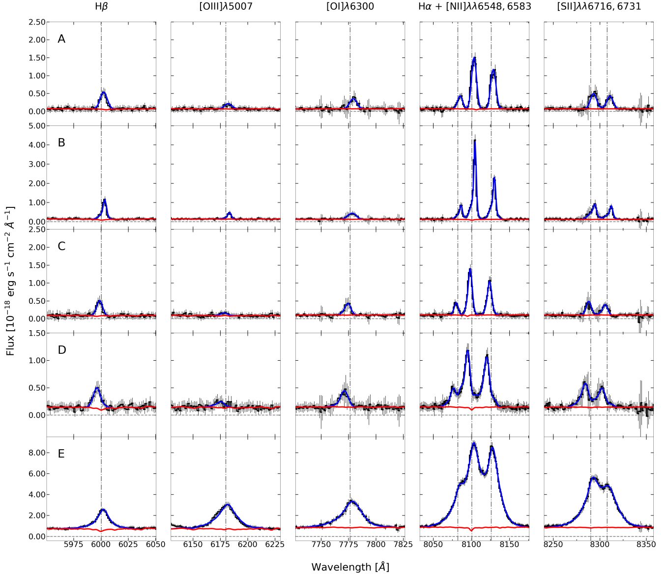
Figure 5. MUSE representative spectra and 3\text{-}\sigma errors of the sky regions A, B, C, D, and E, presented in Sec. 3.3.1, Fig. 7. The red solid line corresponds to the SINOPSIS model of the stellar continuum while the blue solid line shows the fit of the spectra emission lines as obtained by our Python code (see Sec. 3.3). The vertical dash-dotted lines are indicative of the expected wavelength of each line, according to the BCG redshift.
