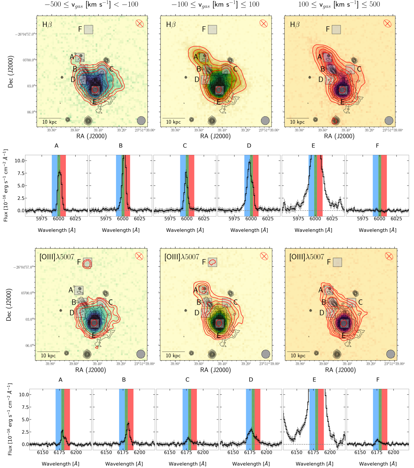
Figure 7. H \beta (top panels) and [OIII] \lambda 5007 (bottom panels) emission in Abell 2667 BCG with contours and symbols as defined in Fig. 2.. The images show the emission line integrated flux within three different velocity channels: from -500 to -100 \text{ km s}^{-1} (blue), from -100 to 100 \text{ km s}^{-1} (green) and from 100 to 500 \text{ km s}^{-1} (red). In each panel, the red solid lines are indicative of the 85.0, 90.0, 93.0, 95.5, 99.7 percentiles of the emission lines flux, respectively. For both H \beta and [OIII] \lambda 5007, we report cutouts of the integrated spectra of six peculiar small ( 1'' \times 1'' ) sky regions, labelled with capital letters, and chosen to be representative of very different areas of the galaxy. In each cutout, the shaded areas indicate the different velocity ranges we adopted.
