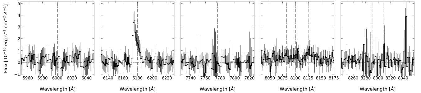
Figure C1. Integrated spectrum of the Ly \alpha -emitter candidate at z \sim 4.08 (F region, see Fig. 7). We present wavelength cutouts of the MUSE observed spectrum (grey solid line) and its 3\text{-}\sigma error, integrated over a 1.2'' \times 1.2'' region centred at RA(J2000.0)= 23^h 51^m 39.507^s , Dec(J2000.0)= -26^\circ 04' 56.81'' . In the cutouts, the vertical dash-dotted lines indicate the expected wavelength of H \beta , [OIII] \lambda 5007 , [OI] \lambda 6300 , H \alpha + [NII] and the [SII] doublet at the BCG redshift. The only line we detect falls in the [OIII] \lambda 5007 cutout. However, the absence of the weaker component of the [OIII] doublet and of the other lines, together with the highly asymmetric shape of the emission, suggests that the detection corresponds to a different line, possibly a Ly \alpha .
