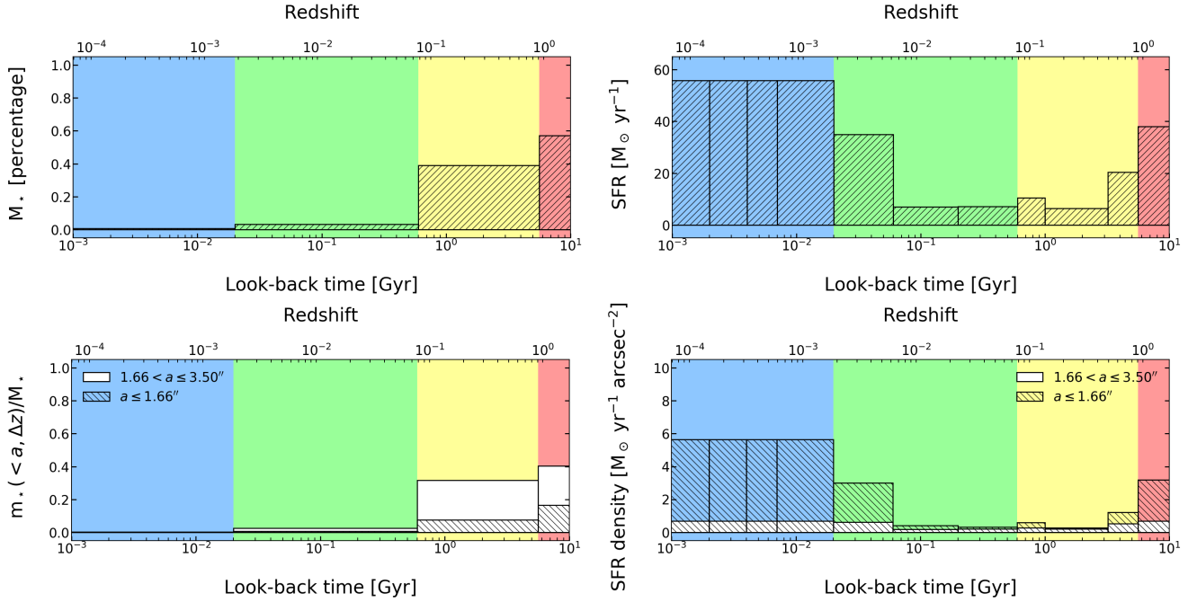
Figure 4. Top panels: SINOPSIS spatially integrated mass building ( left panel ) and star formation history ( right panel ) of the Abell 2667 BCG. The colour-shaded areas of the diagrams represent the four main age bins within which SINOPSIS calculates the galaxy percentage of mass built and SFR (see Fig. 3). In the right panel, the histogram shows the SFH computed in the highest temporal resolution mode (11 SSPs age intervals). Both the percentage of mass built and the SFR of each time-bin have been obtained integrating all the maps values within an elliptical region centred at the galaxy coordinates, with axis ratio b/a = 0.76 , position angle PA = 48.89^\circ (for the parameters see Sec. 3.1) and semi-major axis a = 3.5'' . Bottom panels: Percentage of the stellar mass built ( left panel ) and SFR density ( right panel ) at different epochs for the nuclear ( hatched histogram ) and external regions ( white histogram ) of the BCG. For the nuclear region we have integrated SINOPSIS spatially-resolved values within an elliptical aperture centred at the galaxy coordinates, with b/a , PA as before, but a = 1.66'' . For the outskirts, we have resorted to an elliptical annulus with central coordinates, b/a and PA as before, but with 1.66'' < a \leq 3.55'' . The two different areas are marked with the two white ellipses in the top left-hand side panel of Fig. 3.
