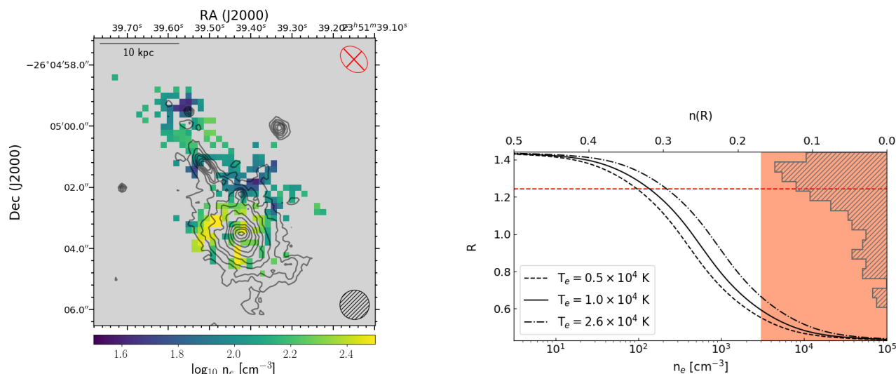
Figure 9. Left panel: Electron density ( n_e ) map for Abell 2667 BCG as retrieved from Eq. 2 for an electron temperature T_e = 1.0 \times 10^4 K, with contours and symbols as defined in Fig. 2. Right panel: Electron density ( n_e ) curve (Proxauf et al. 2014) as a function of the intensity ratio R = [\text{SII}]\lambda 6716/[\text{SII}]\lambda 6731 for T_e = 0.5 \times 10^4 K (black dashed line), T_e = 1.0 \times 10^4 K (black solid line) and T_e = 2.6 \times 10^4 K (black dash-dotted line). The red area of the diagram highlights the electron density values above the [SII] doublet critical density (i.e. n_e \sim 3 \times 10^3 \text{ cm}^{-3} ). We present the distribution of the retrieved R values as well as the median value of the distribution R \sim 1.21 (red dashed line).
