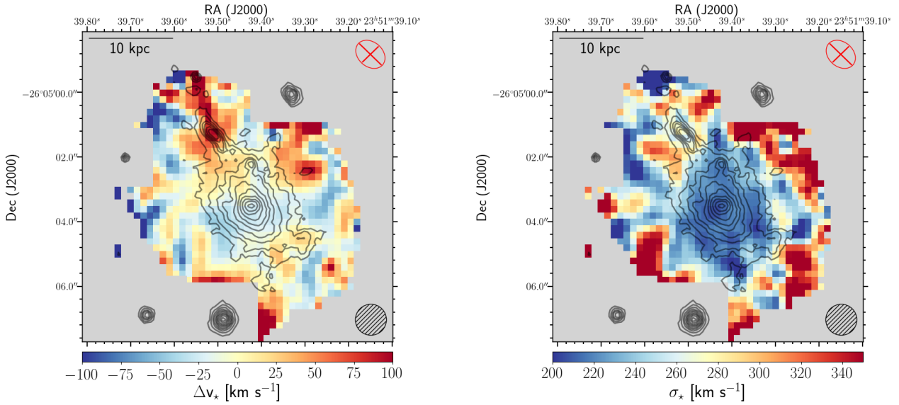
Figure 2. pPXF maps for the stellar velocity ( left panel ) and velocity dispersion ( right panel ) along the observer's line-of-sight, with the Hubble Space Telescope F450W WFC2 contours superimposed ( grey solid lines ). In both maps, the spaxels with a \text{SNR} < 3 are coloured in grey. The hatched black circle on the bottom right-hand side shows the beam size of the average V-band observed seeing of \sim 0.96'' (FWHM) while the red ellipse on the top indicates the galaxy orientation in the sky-plane. The ratio between the ellipse's axis corresponds to the b/a value retrieved by the two dimensional surface brightness model of the galaxy by galfitm .
