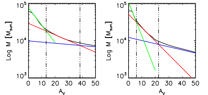
Figure 7. Expanded view of the low extinction range of the CMDs in Figure 5, highlighting the breaks and the best linear fits to the data for W3 Main/(OH) (left), and AFGL 333 (right).
