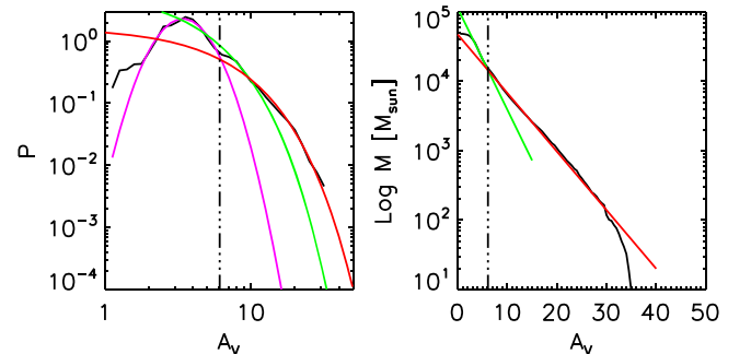
b W3 NW field
