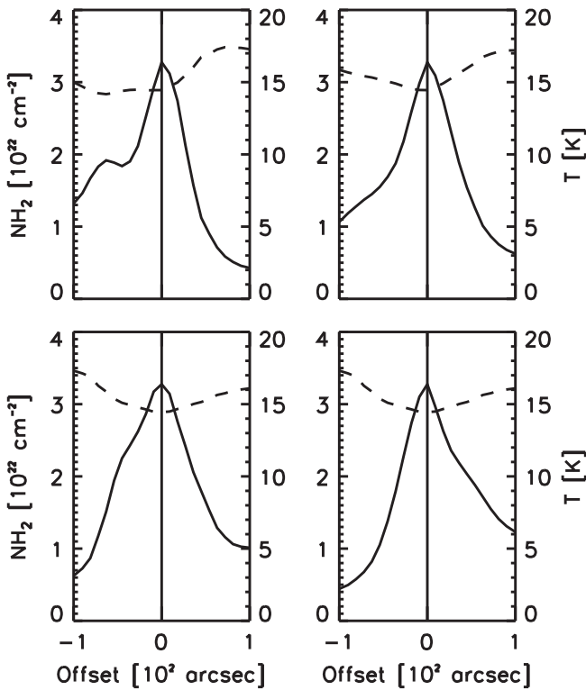
Figure 8. Profiles 200'' ( \sim 2 pc) long through the column density peak of the Trilobite centered on position R.A./decl.: 2^{\text{h}}21^{\text{m}}5^{\text{s}}.3 , +61^{\circ}27'29''.1 . Both temperature (dashed line; right scale) and column density (solid line; left scale) are shown for different orientations of the profile: in the west–east direction (top-left); NW–SE (top-right); north–south (bottom-left); NE–SW (bottom-right). Black vertical line marks the coordinate center (solid line).
