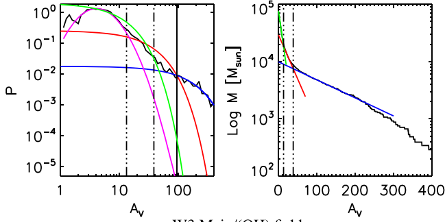
a W3 Main/(OH) field
