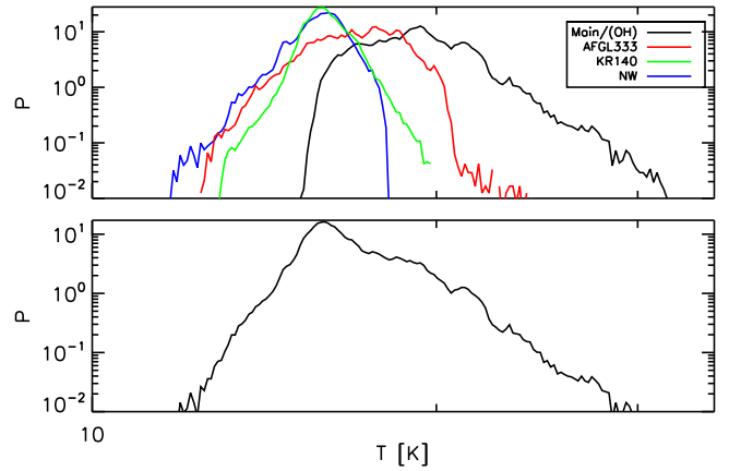
Figure 4. Like Figure 2, but for the logarithmized PDF of dust temperature. Top: for each field in W3. Bottom: global PDF of the W3 GMC.
