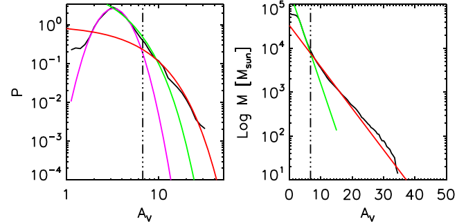
a KR 140 field
