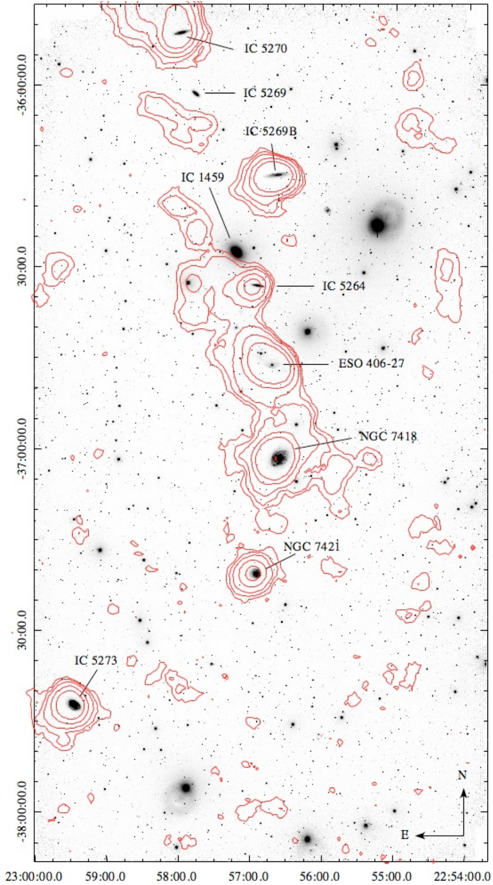
Fig. 1. OmegaCAM at VST mosaic in g band of the IC 1459 group with the HI map from the KAT-7 observations (red contours). The image size is about 1^\circ \times 2^\circ , and the HI contour levels are 5.5, 10, 20, 50, and 100 \times 10^{18} \text{ cm}^{-2} (as shown by Oosterloo et al. 2018). The right ascension and declination (J2000) are given in the horizontal and vertical axis of the field of view, respectively. North is at the top and east is to the left.
