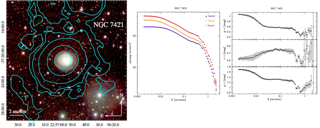
Fig. B.7. Same as Fig. B.1 but for NGC 7421. The HI contour levels are 0.25, 0.5, 1.5, 5 , and 10 \times 10^{19} \text{ cm}^{-2} .
