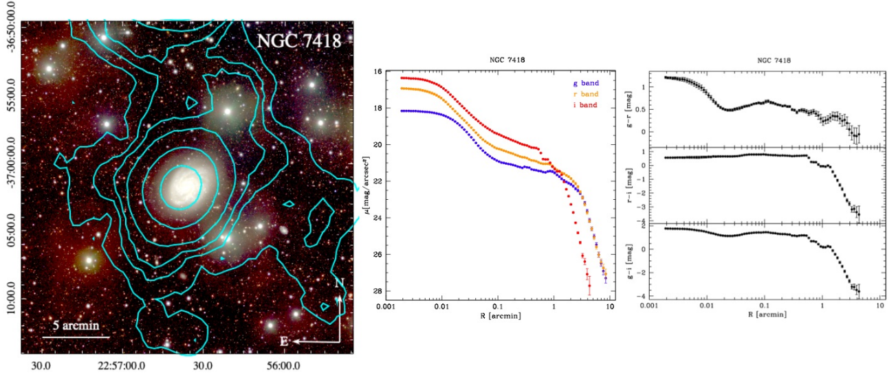
Fig. B.6. Same as Fig. B.1 but for NGC 7418. The HI contour levels are 0.5, 1.5, 2.5, 5, 15 , and 35 \times 10^{19} \text{ cm}^{-2} .
