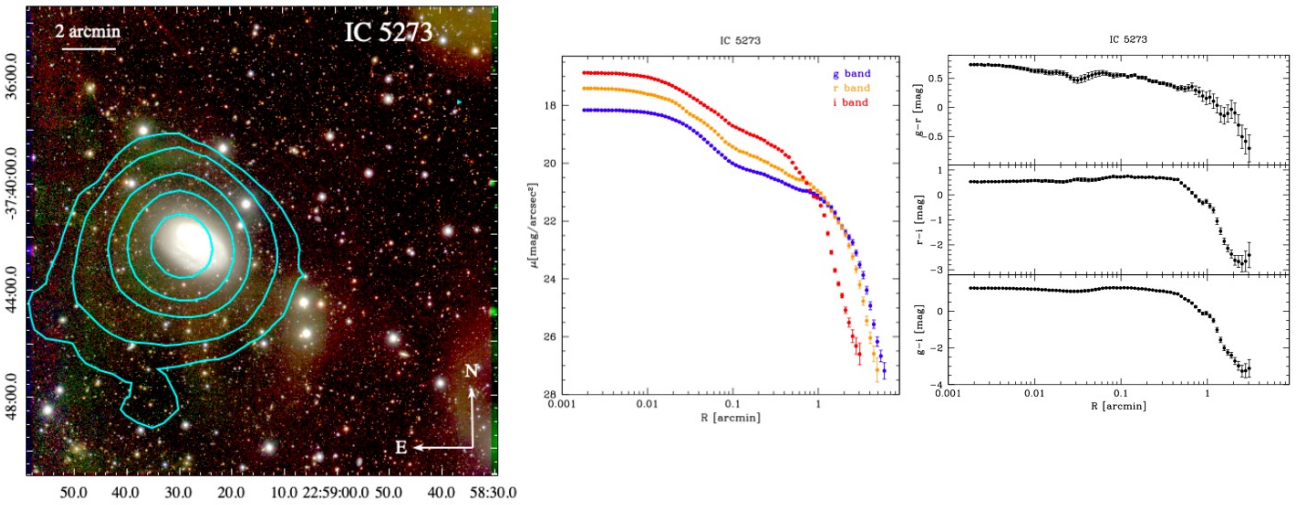
Fig. B.8. Same as Fig. B.1 but for IC 5273. The HI contour levels are 1, 2.5, 7.5, 12.5 , and 20 \times 10^{19} \text{ cm}^{-2} .
