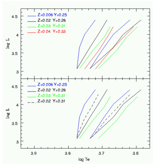
Fig. 5. The CC IS at varying the metallicity and the Helium content.
