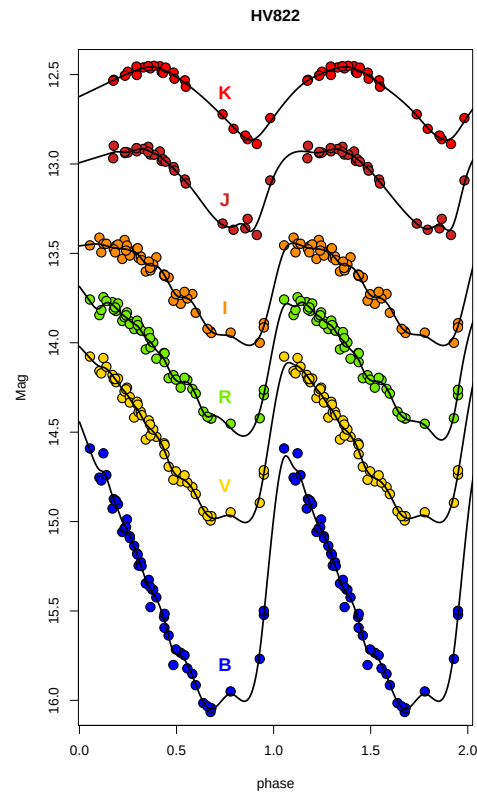
Fig. 4. A typical CC light curve in the BVR IJHK bands (data from Storm et al. 2004).
