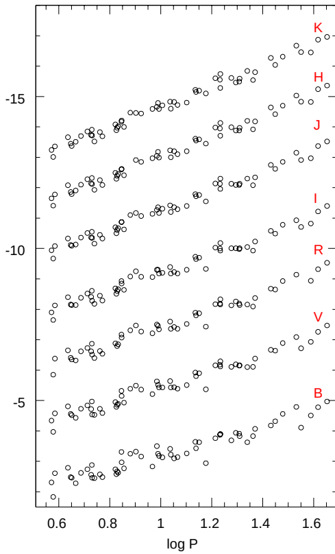
Fig. 3. PL relations obtained adopting the BVR IJHK data for Galactic CCs by Fouqué et al. (2007) (see text for details).
