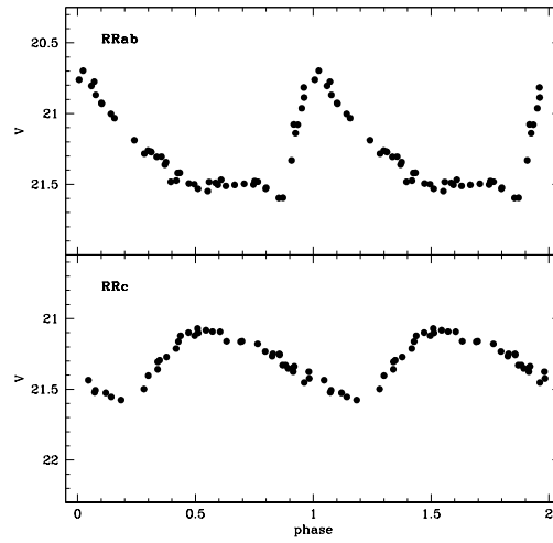
Fig. 9. The typical light curves of a RRab and of a RRc are plotted in the top and in the bottom panel, respectively.
