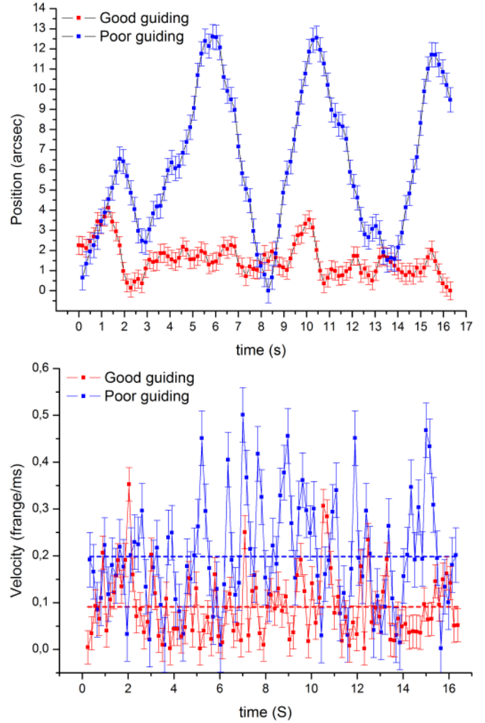
Fig. 7. Position (top) and its derivative (velocity at bottom) of the guiding focal image projected on an axis perpendicular to the fringes of the short baseline. The red and blue curves correspond to periods with small and large amplitude oscillations obtained on \alpha And (data selected among the recorded images between 22h57 and 23h00) and \gamma And (data selected in the first minute of the recorded images between 02h52 and 02h57). The unit of the vertical position axis is one arcsecond (1 pixel = 0.133'' on the guiding camera). The error bars are the median seeing at the moment of the observation. The error bars of the bottom graph are the standard deviation ( \sigma ) of the velocity points. The mean velocities are 0.2 and 0.1 fringe/ms for guiding with large and small oscillations, respectively. One pixel of the guiding camera equals 6 fringes for the 5 m baseline. It is expressed in fringe/ms, but for guiding with small amplitude oscillations, the fringes move probably less than 0.1 fringe/ms because this value is affected by the atmospheric tip-tilt.
