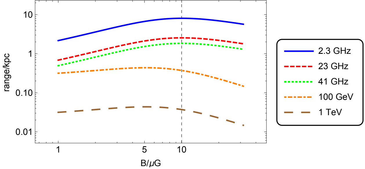
Fig. 10.— Ranges of cosmic-ray electrons downstream of the shock that emit synchrotron radiation into the specified characteristic frequency or with energies 100 GeV and 1 TeV (dominating IC emission) as a function of downstream region magnetic field. The range is determined by the condition that t_{\text{transport}} = t_c with both synchrotron and IC losses accounted for. Here the downstream gas velocity is assumed to be a fixed 112 km/s ( \sim 1/4 v_w ) and the cosmic rays are taken to stream at the Alfvén speed in the specified field and for a density of \rho = 1.4 n_H m_p where we adopt n_H = 3 \times 10^{-3} \text{ cm}^{-3} . Note that Haze electrons reach a maximum \sim 3 kpc downstream from the shock and 2.3 GHz electrons can reach a maximum \sim 10 kpc; electrons IC emitting 1-100 GeV \gamma -rays are concentrated close to the shock. The vertical line shows the \sim 10 \mu\text{G} field where the range of the radio and microwave-emitting electrons is approximately maximised. The total vertical extent of the Bubbles is \sim 8 kpc with the shocks forming at heights \sim 1 kpc; note that 2.3-GHz-emitting electrons can reach the edges of the Bubbles whereas microwave-emitting electrons do not; from this analysis the vertical extent of the microwave should be \sim R_{\text{sh}} + \text{range}[23 \text{ GHz}] \sim 3 kpc; this is consistent with observations that show a drop-off in the intensity of the microwave emission at \sim 35^\circ corresponding to the distance of 2.7 kpc for the near-surface of the Bubbles at 5 kpc distance.
