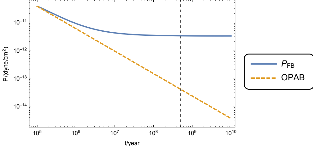
Fig. 6.— Pressure interior to the contact discontinuity (solid blue); this asymptotes to the assumed atmospheric pressure 3.2 \times 10^{-12} \text{ dyn cm}^{-2} . Parameters as for Figure 4. The vertical line indicates when the bubble has attained a volume equivalent to the observed Fermi Bubbles (cf. Figure 4). The dashed orange curve is for an over-pressured, adiabatic bubble.
