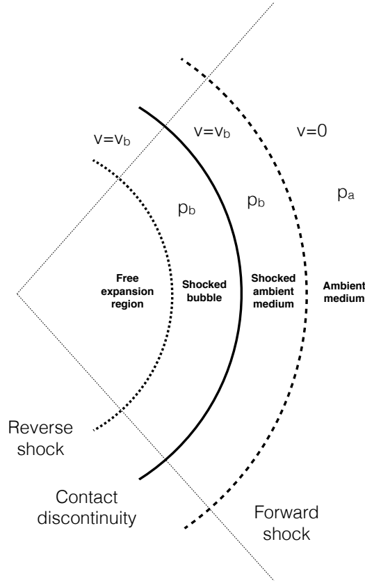
Fig. 3.— Illustration of the key features of a bubble.
