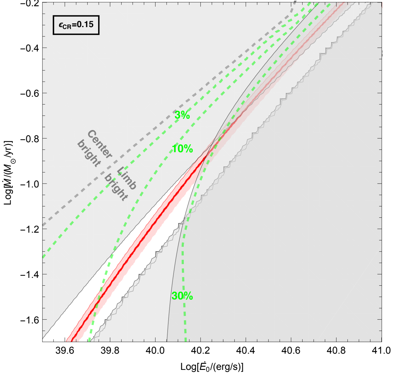
Fig. 9.— Predicted hadronic and IC \gamma -ray luminosity within the allowed parameter space for the case that P_{\text{halo}} = 2 \text{ eV cm}^{-3} , \epsilon_{\text{CR}} = 0.15 and T_{\text{shell}} = 3.5 \times 10^6 \text{ K} . Regions that are masked out in gray do not obey all the physical or observational constraints as in Figure 8. The pink/red band is the locus of parameter space points for which the predicted hadronic luminosity is close to that observed (central value of 4.4 \times 10^{37} \text{ erg/s} over 100 \text{ MeV} < E_\gamma < 500 \text{ GeV} with 1\text{-}\sigma statistical+systematic errors shown as the pink regions: Fermi-LAT Collaboration 2014). The green dashed curves report the total 100 MeV-500 GeV inverse Compton (IC) luminosity as a proportion (3%,10%, or 30% as labeled) of 4.4 \times 10^{37} \text{ erg/s} . The IC curves assume that, of the 15% of the mechanical energy at each shock that goes into freshly-accelerated cosmic rays, 10% goes into primary electrons, L_e = 0.1 L_{\text{CR}} = 0.1 \times 0.15 \times \dot{E} . The gray, dashed curve shows where the naive flat surface brightness condition (eq. 6-13) is exactly satisfied.
