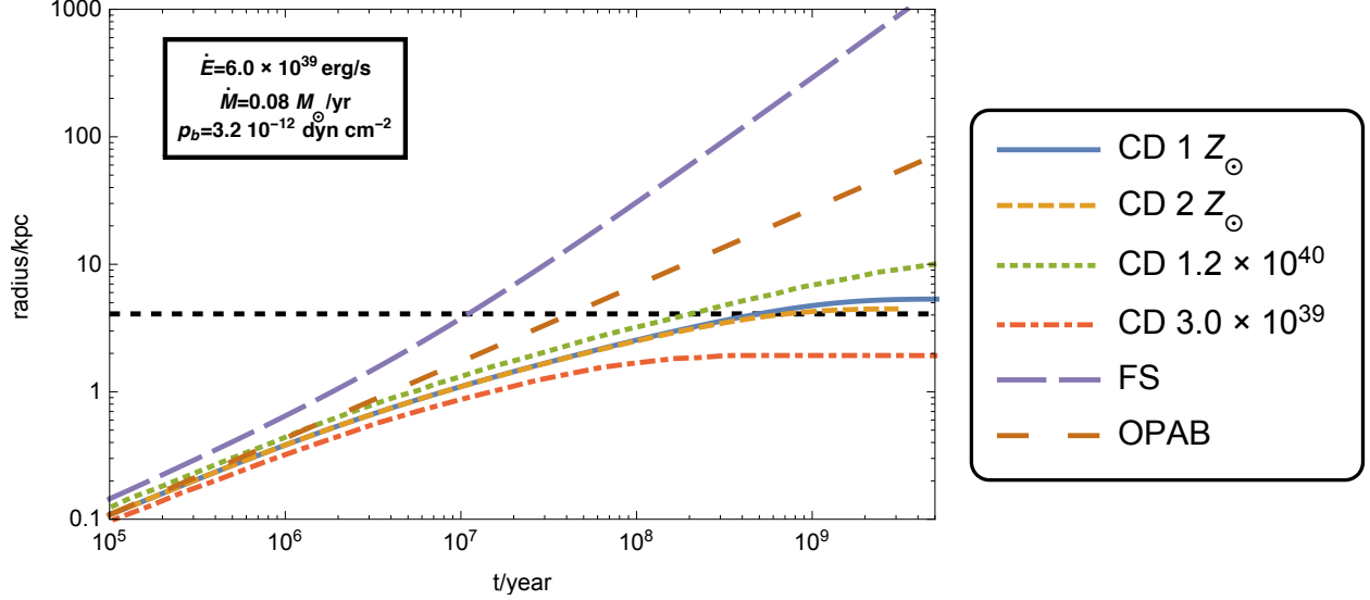
Fig. 4.— Radius of the bubble contact discontinuity (CD) and forward shock (FS) vs. time for \dot{E} = 6 \times 10^{39} erg/s and solar metallicity (unless otherwise marked) and \dot{M} = 0.08 M_{\odot}/\text{yr} (fixed); the atmosphere has pressure 2.0 \text{ eV cm}^{-3} \simeq 3.2 \times 10^{-12} \text{ dyn cm}^{-2} . Contact discontinuity (CD) curves are: i) solid blue for \dot{E} = 6.0 \times 10^{39} erg/s; ii) dashed orange for \dot{E} = 6.0 \times 10^{39} erg/s and cooling with twice solar metallicity ( Z = 2Z_{\odot} ); iii) dotted green for \dot{E} = 1.2 \times 10^{40} erg/s; and iv) dot-dashed orange for \dot{E} = 3.0 \times 10^{39} erg/s. The long dashed violet curve is for the forward shock. The brown long-dashed curve shows the analytical result for the expansion of an over-pressured, adiabatic bubble (OPAB; see Appendix); this very substantially over-estimates the bubble radius for t \gtrsim \text{few} \times 10^7 yr. The horizontal black dashed line represents the equivalent spherical radius of 4.1 kpc corresponding to the total volume of the Fermi Bubbles; for the fiducial model the bubble has attained this size by \sim 5 \times 10^8 yr.
