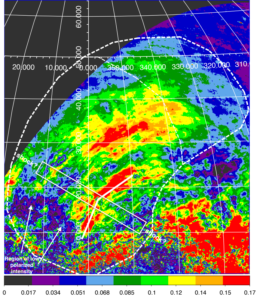
Fig. 13.— Inflexion in the GC Spur in the northern bubble traced in white. colors show 2.3 GHz polarisation data from S-PASS (Carretti et al. 2013) in Galactic coordinates with east to the left and the edge of the black triangle to upper left corresponding to the instrumental horizon. The color bar units are Jy/beam (convolved beam is approximately 10' ). The outer dashed contour delimits the northern S-PASS polarized radio lobe (Carretti et al. 2013); the northern Fermi Bubble (Su et al. 2010) edge is contiguous except in the north west where it runs inside the boundary of the radio lobe as shown by the thinner dashed line. The large, inclined rectangle indicates the position of a faint depolarisation feature, running from north-east (top left) to south-west (bottom right) through the inflexion point, that might be attributed to a magnetic field aligned with the surface of the giant reverse shock. A region of low polarized intensity at 2.3 GHz in the lower south east is indicated; this region is also evident at 23 GHz.
