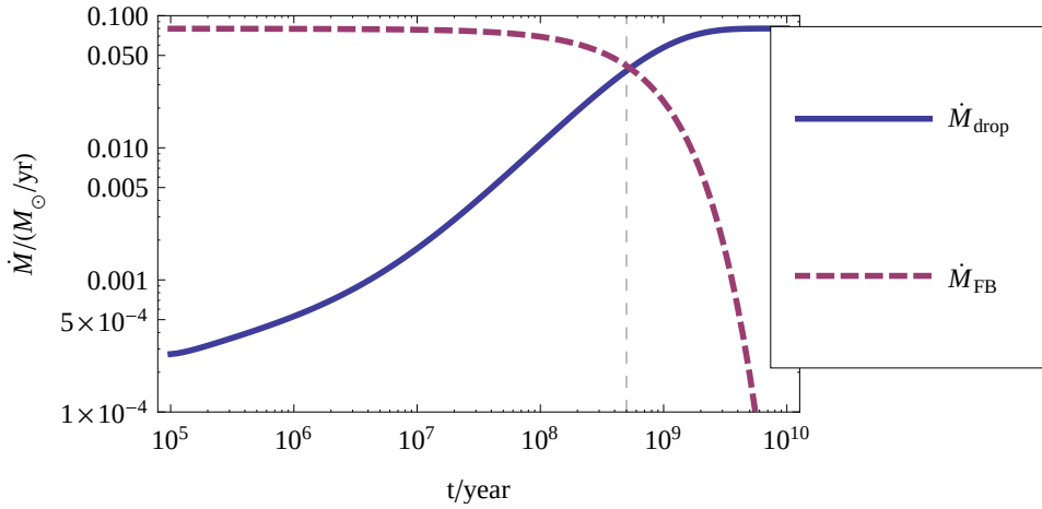
Fig. 7.— Mass drop out (solid blue) and mass growth of Bubbles (dashed purple). Parameters as for Figure 4. The vertical line indicates when the bubble has attained a volume equivalent to the observed Fermi Bubbles (cf. Figure 4). At times \gtrsim Gyr mass drop out by itself saturates the injection rate of freshly-heated plasma.
