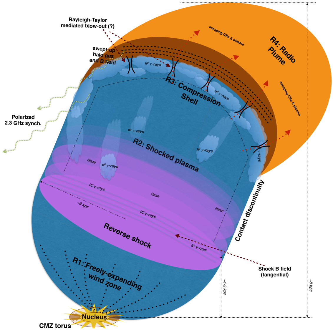
Fig. 1.— Schematic showing the main features of the north bubble according to our model.
