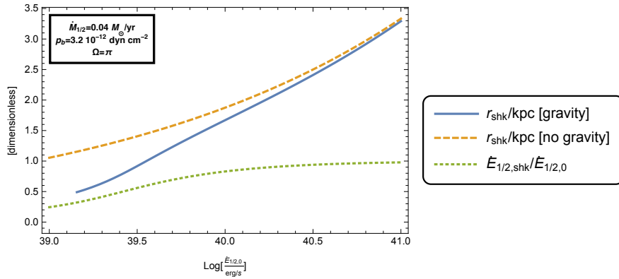
Fig. 2.— Distance to the shock and relative mechanical power at the shock as a function of mechanical power injected at the nucleus into one hemisphere, \dot{E}_{1/2,0} . The downstream thermal pressure in the bubble is 2\text{ eV cm}^{-3} \simeq 3.2 \times 10^{-12}\text{ dyn cm}^{-2} , the mass flux into the flow is 0.04\text{ }M_{\odot}/\text{yr} and we adopt \Omega \simeq \pi (Lacki 2014), corresponding to an expansion cone angle \sim 120^\circ .
