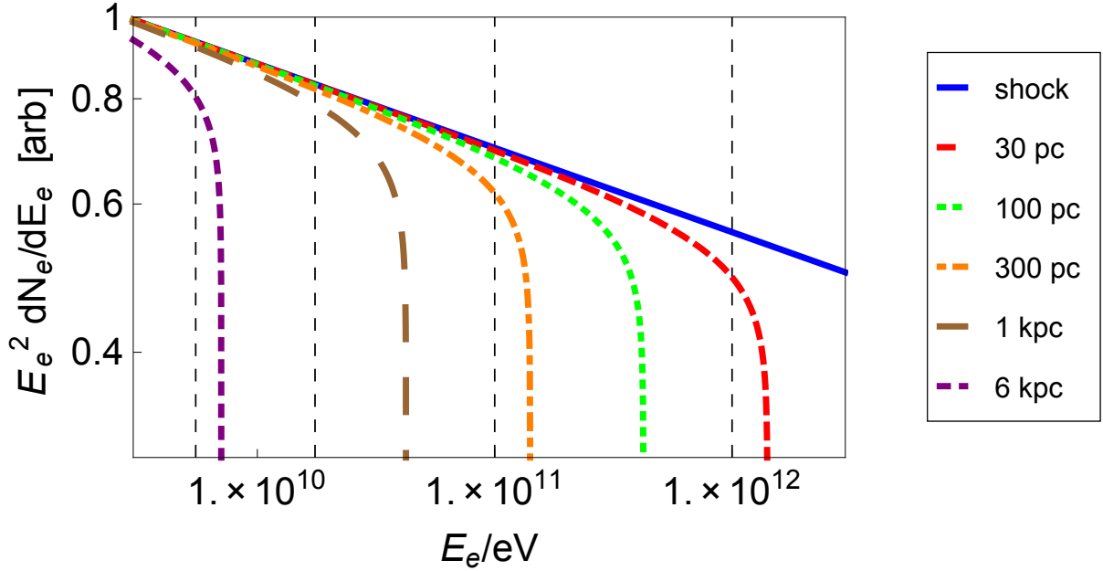
Fig. 11.— Spectra of cosmic-ray electrons at various distances downstream of a shock. The electrons are injected at the shock with an assumed distribution dN_e/dE_e \propto E_e^{-2.1} and are conveyed downstream at a total speed given by the downstream flow speed (112 km/s) + streaming at the Alfvén speed (240 km/s). At the same time, they suffer synchrotron (with B = 7\mu\text{G} ) and IC losses ( U_{ISRF} = 1.5 \text{ eV cm}^{-3} ); the position-dependent spectrum evolves according to Eq. 6-15. From left to right, the vertical dashed lines indicate the primary electron energy corresponding to i) synchrotron emission at 2.3 GHz; ii) synchrotron emission at 23 GHz; iii) 100 GeV IC emission off starlight; and iv) 10 GeV IC emission off the CMB. Note that, for these (realistic) parameters, IC emission is concentrated within < \text{kpc} of the shock; in contrast 23-GHz emitting electrons extend \sim 2 \text{ kpc} , and 2.3-GHz emitting electrons can reach the full extent of the Bubbles. Note there is a one-to-one correspondence between distance from shock and time since acceleration (electron ‘age’) with the implication that, provided the emission is resolved, nowhere does the spectrum steepen by the canonical -1 due to the synchrotron + IC losses, rather it maintains its hard injection spectral index up to some distance/time-dependent energy above which it is cut-off.
