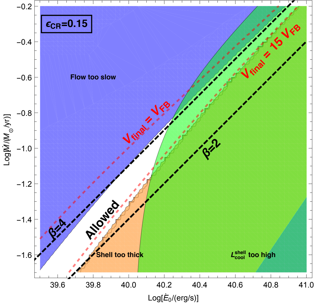
Fig. 8.— Explored \{\dot{E}_0, \dot{M}\} parameter space and excluded regions for the case that P_{\text{halo}}^{\text{FB}} = 2 \text{ eV cm}^{-3} , \epsilon_{\text{CR}} = 0.15 and T_{\text{shell}} = 3.5 \times 10^6 \text{ K} . White space shows the allowed region. The region masked out in green predicts a bolometric cooling luminosity ( > 10^{40} \text{ erg/s} ) from the compression shell (R3) that is too high to be compatible with X-ray constraints from ROSAT (Snowden et al. 1997; Almy et al. 2000). The region masked out in orange predicts a compression shell that is too thick ( > 1.4 \text{ kpc} ). The region masked out in blue predicts that the flow from the interior region into the shell is too slow, i.e., the transport time from R2 to R3 is longer than the plasma cooling time in R2 so the plasma cools before it reaches the shell at variance with the assumptions of the model. The thick black dashed curves delineate the star-formation-driven mass efflux vs. mechanical energy input into the giant outflows for mass loading rates of \beta = 2 and 4 , scaling the results of Strickland & Heckman (2009). The dashed red lines trace the locus of \dot{E}_0/\dot{M} points that generate asymptotic volumes of, respectively, V_{\text{FB}} and 15 \times V_{\text{FB}} obtained from eq. 4-1.
