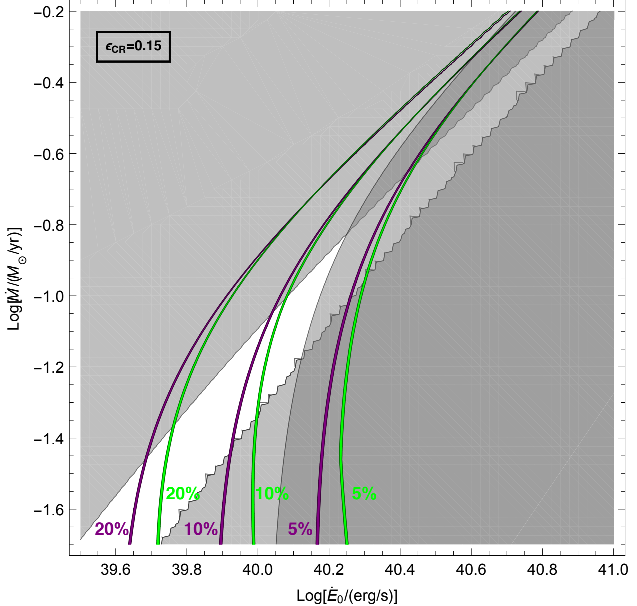
Fig. 12.— Predicted synchrotron emission for P_{\text{halo}} = 2 \text{ eV cm}^{-3} , \epsilon_{\text{CR}} = 0.15 and T_{\text{shell}} = 3.5 \times 10^6 \text{ K} . Regions masked out in gray do not obey all the physical constraints as described in Figure 8. Purple curves refer to the microwave Haze and green curves to the giant, 2.3 GHz radio lobes. The curves are labelled according to where the modelled 2.3 GHz and 23 GHz intensity matches that observed for the nominated percentage of total cosmic-ray power going into freshly accelerated electrons, viz. L_e = \{5\%, 10\%, 20\%\} \times L_{\text{CR}} where L_{\text{CR}} \equiv \epsilon_{\text{CR}} \dot{E} with \dot{E} the mechanical power arriving at the shocks. The curves account for both primary and secondary electron synchrotron; here, secondary synchrotron accounts for 5-20% of the total 2.3 GHz intensity over the favored parameter space. The purple curve for emission over the Haze region assumes a volume-filling magnetic field of 7 \mu\text{G} and an interstellar radiation field calculated at 3 kpc above the plane ( U_{\text{ISRF}} = 1.7 \text{ eV cm}^{-3} ; Porter et al. 2008); we adopt reference values for the Haze intensity at 23 GHz of 1200 \text{ Jy/sr} (Su et al. 2010) and 18.5 \text{ kJy/sr} for the total intensity at 2.3 GHz (Carretti et al. 2013).
