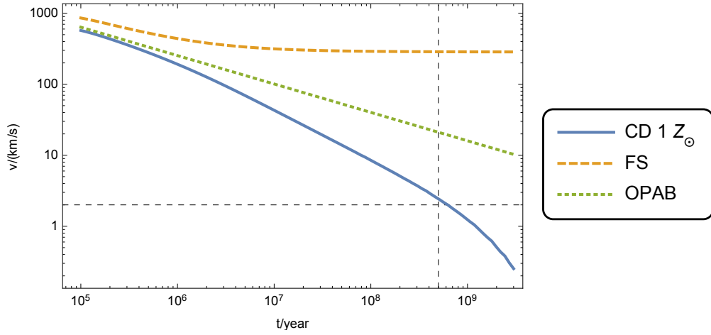
Fig. 5.— Velocity of the bubble contact discontinuity (CD) and forward shock (FS) versus time for cooling with Z = Z_{\odot} . Parameters as for Figure 4. The dotted (green) curve shows the analytical result for the expansion of the contact discontinuity of an over-pressured, adiabatic bubble (OPAB). The expansion velocity of the forward shock asymptotes to the sound speed as it degenerates into a sound wave. For the chosen parameters, at the age ( \sim 5 \times 10^8 yr indicated by the vertical line) where the bubble has attained a volume equivalent to the observed Fermi Bubbles (cf. Figure 4), its contact discontinuity is expanding at 2-3 km/s.
