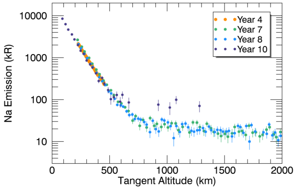
Figure 9. Altitude profiles of sodium emission observed above Mercury's subsolar point by the MESSENGER MASCS UVVS instrument. These were taken over several Mercury years (as indicated by the legend), but all were taken near the same true anomaly angle, between 65°-70° in this example. Although the sodium exosphere varies temporally, this figure highlights the seasonal repeatability of MASCS observations.
