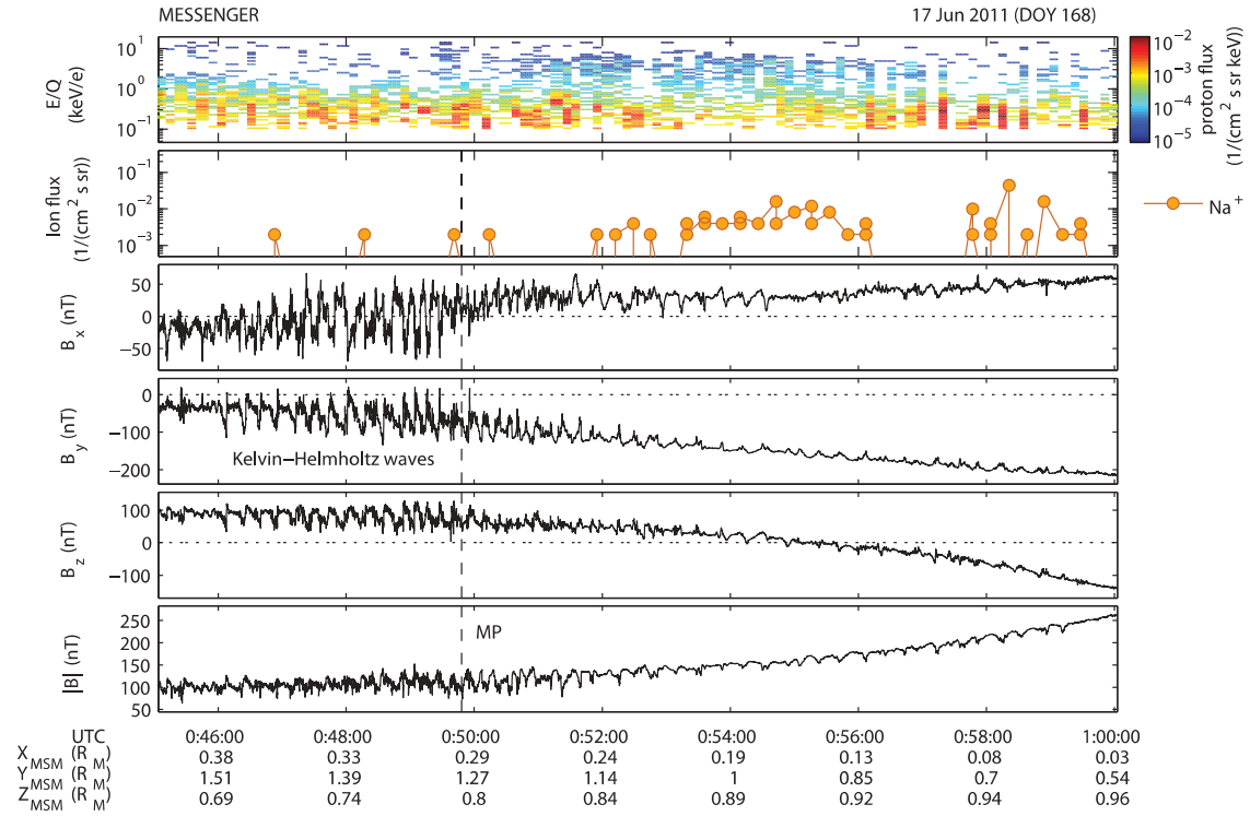
Figure 7. KH observations on 17 June 2011. The first and second panels show the FIPS spectrogram of E/Q for the measured proton flux and the sodium ion count rate, respectively. The third–fifth panels are the magnetic field components and the sixth panel is magnetic field strength. Adapted from Sundberg et al. [2012].
