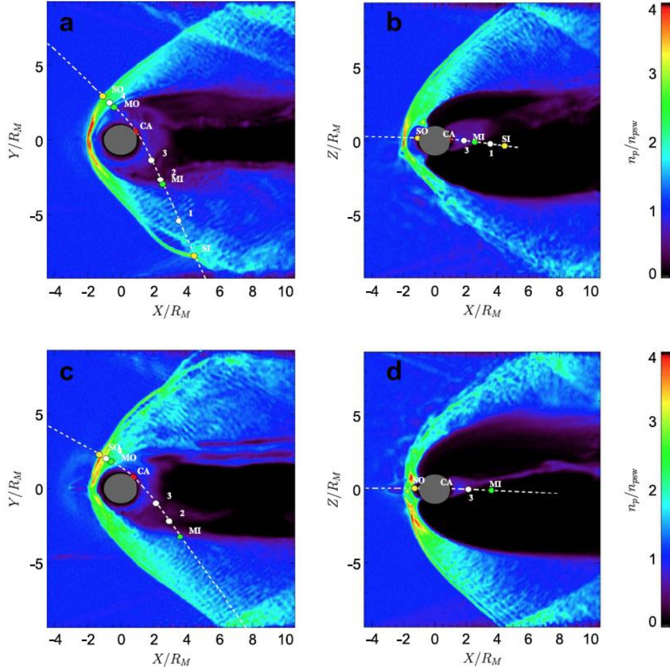
Figure 18: Simulated magnetospheric configuration from the global hybrid model of Travenick et al. (2010). Panels (a) and (b) show the simulated solar wind proton density in the equatorial and noon-midnight meridional planes, respectively, under northward IMF conditions. Panels (c) and (d) are the same but for southward IMF. Colors in each panel represent the density of solar wind protons normalized to the upstream value. MESSENGER trajectories of the M1 and M2 flybys are superimposed as white dashed lines.
