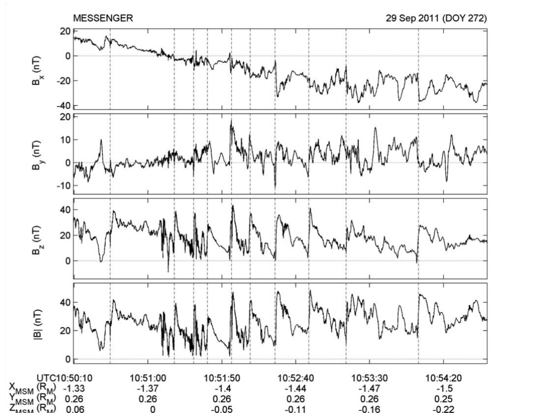
Figure 15. A series of dipolarizations of the magnetic field in the plasma sheet observed by MESSENGER and analyzed by Sundberg et al. [2012]. These brief, several second-long events are marked by vertical dashed line. Each has sudden, strong transitions from the magnetic field being highly stretched to a more dipolar configuration with a greatly enhanced B_z component.
