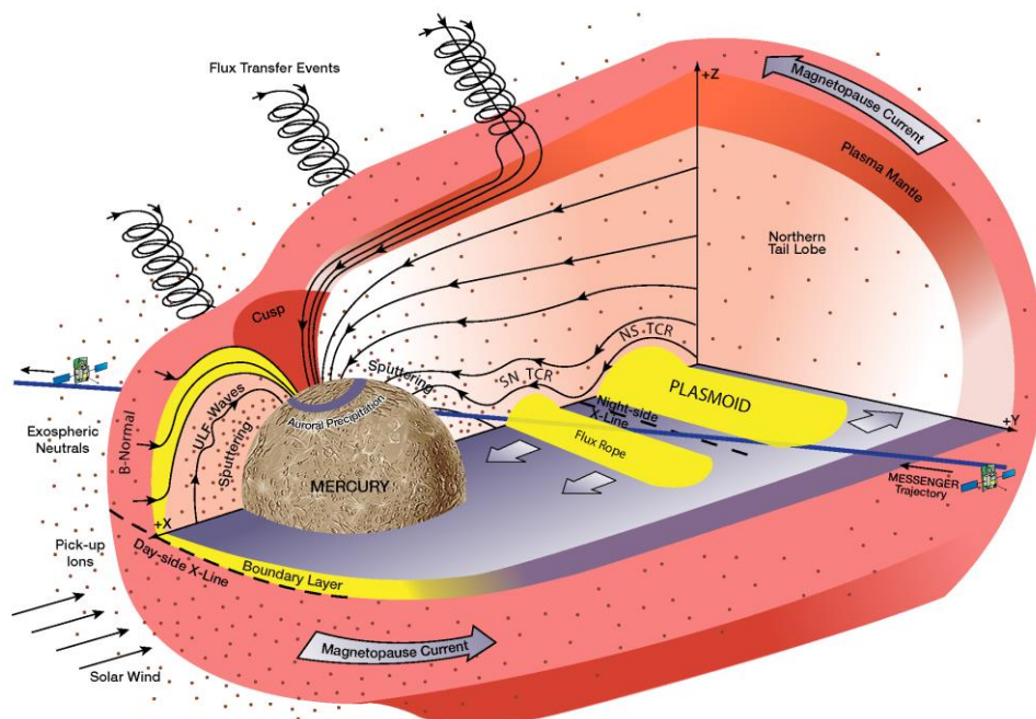
Figure 1. Schematic of Mercury's Dungey cycle. This large-scale magnetospheric convection, responsible for the circulation of plasma and magnetic flux, is driven by steady and impulsive reconnection. Note the strong magnetic field normal to the dayside magnetopause, the large FTEs, and the reconnection line in the near-tail region. Figure from Slavin et al. [2009].
