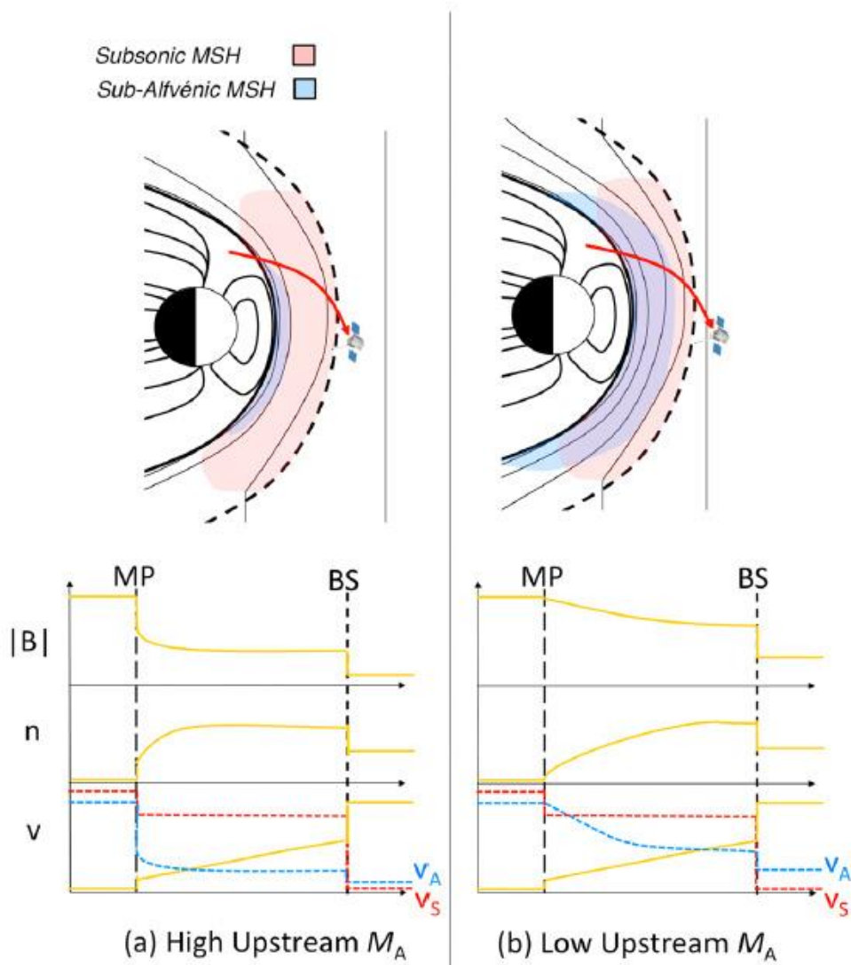
Figure 2. Illustration of a spacecraft pass through the subsolar magnetosheath (MSH) for (a) high solar wind Mach number ( M_A ) and (b) low solar wind M_A . The MSH plasma is subsonic equatorward of the approximately \pm 45^\circ latitude. With decreasing M_A , a larger fraction of the subsolar magnetosheath is sub-Alfvénic, as indicated by the blue shaded region. In addition, a thicker region of magnetic flux pileup is evident by an increase in |B| and a decrease in plasma density, n . The Alfvén speed ( V_A ) and sound speed ( V_S ) are also shown for both cases. Adapted from Gershman et al., 2013.
