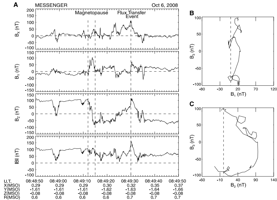
Figure 5. (A) Magnetic field observations of the inner current sheet and MP boundary observed as MESSENGER exited the dawn-side magnetosphere. (B) Magnetic field measurements across the MP graphed in the plane of maximum and minimum variance. (C) Magnetic field measurements across the MP graphed in the plane of maximum and intermediate variance Adapted from Slavin et al. , 2009.
