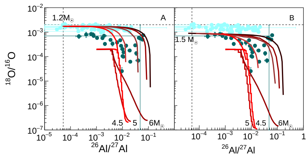
Figure 5. The ^{18}\text{O}/^{16}\text{O} isotopic ratio as a function of the ^{26}\text{Al}/^{27}\text{Al} one for the same models and grain data as in Figure 3. Horizontal and vertical dashed lines represent the solar values for the ^{18}\text{O}/^{16}\text{O} and the ^{26}\text{Al}/^{27}\text{Al} isotopic ratios. Panel (A) refers to calculations run with reaction rates of set A and Panel (B) to calculations run with the set B.
