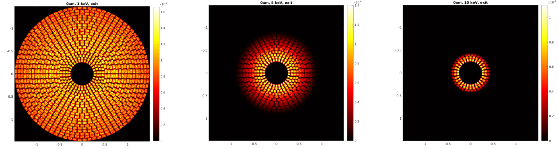
Figure 4. ATHENA optics through McXtrace ray-tracing. Example of simulated photons at exit of the optics for on-axis exposure with photon energies of 1 keV (left), 5 keV (center) and 10 keV (right).
