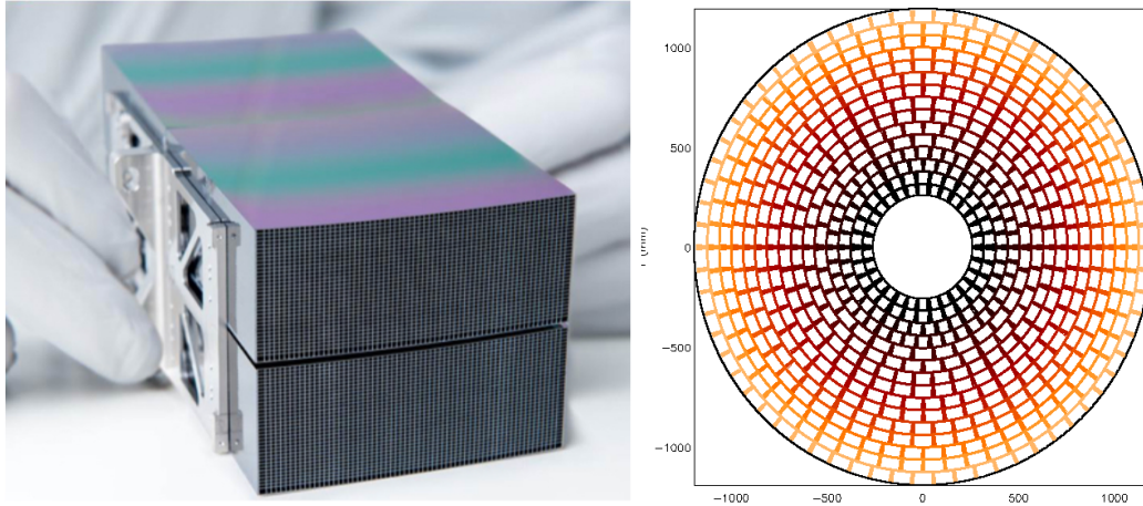
Figure 1. Left: A Wolter I SPOs mirror module (image credits ESA). The MM is realized as a double stack of 34 plates assembled in Wolter I configuration. Right: Graphic representation of the MMs positions in the ATHENA telescope. The MMs are organized in 15 rows with hexagonal symmetry.
