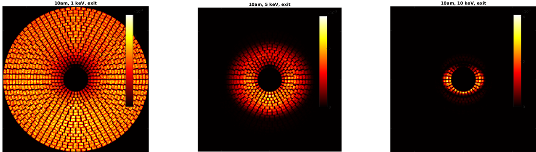
Figure 5. ATHENA optics through McXtrace ray-tracing. Example of simulated photons at exit of the optics for 10 arcmin off-axis exposure with photon energies of 1 keV (left), 5 keV (center) and 10 keV (right).
