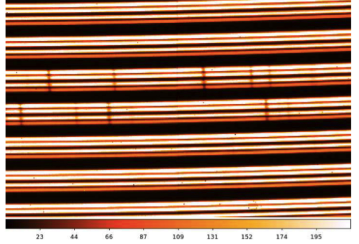
Fig. B.1. Zoom-in on a GIANO image of a continuum lamp. Note that each order is split in four parallel tracks due to the insertion of an image slider that divides the image of the two fibres.
