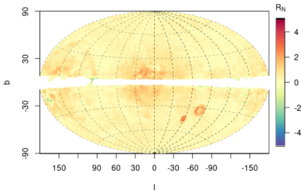
Fig. 31. Comparison of the total galactic extinction map ( a0 ) with Planck E(B - V) normalised by the error R_N = (a0 - E(B - V)) \times 3.1 / (a0\_uncertainty \times \sqrt{\text{num\_tracers\_used}}) . The white area corresponds to locations with status > 0 .
