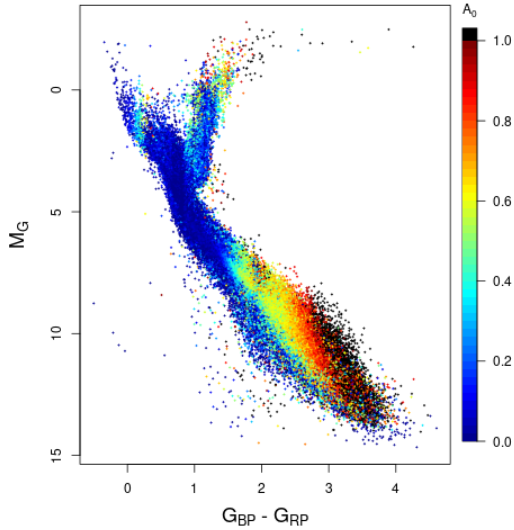
Fig. 30. Hertzsprung-Russell diagram of low-extinction stars ( A_0 < 0.05 mag according to Lallment et al. 2019) with a parallax relative precision lower than 10%, colour-coded with the mean extinction azero\_gspphot . The colour is saturated as black for values higher than 1 mag. In this low extinction sample, M_G is simply G + 5 + 5 \log(\varpi/1000) .
