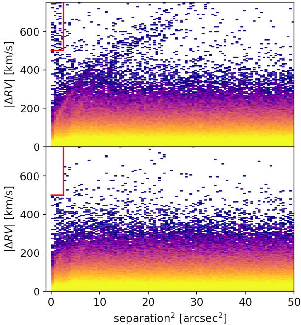
Fig. 1. Differences in radial velocities of the members of close pairs of sources as a function of the square of the angular separation in \text{arcsec}^2 (top) and after filtering (bottom). The red lines enclose one of the criteria that were used to filter the problematic cases.
