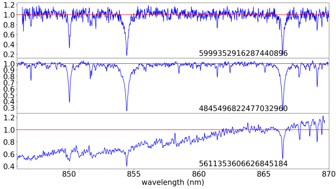
Fig. 13. Three example spectra with three different continuum levels.
