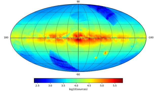
Fig. 14. Density of Gaia DR3 sources in the sky with available xp_continuous_mean_spectrum in Galactic coordinates.
