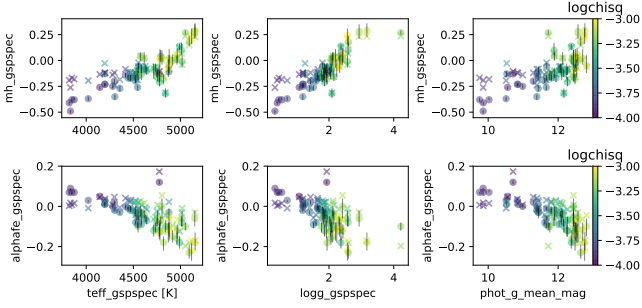
Fig. 36. Abundance trends for mh_gspspec (top) and alphafe_gspspec (bottom) as a function of teff_gspspec (left column), logg_gspspec (middle column), and phot_g_mean_mag (right column) for the stellar members of NGC 7789. The symbols are colour-coded as a function of logchisq_gspspec . Circles indicate the uncorrected alphafe_gspspec values, and crosses represent the calibrated mh_gspspec and alphafe_gspspec values. The parameters have been filtered with flags_gspspec[1:7,9:13]=0 and flags_gspspec[8]<=2 .
