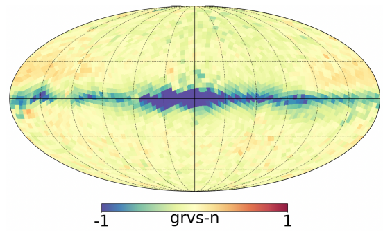
Fig. 11. Relative difference of the number of stars with a G_{\text{RVS}} value between DR3 and GOG20 ( \text{DR3-GOG20}/\text{DR3} ) in the magnitude range 12 < G < 13 in Galactic coordinates. -1 ( +1 ) corresponds to a deficit (an excess) of 100% in DR3 data with regard to the GOG20 model.
