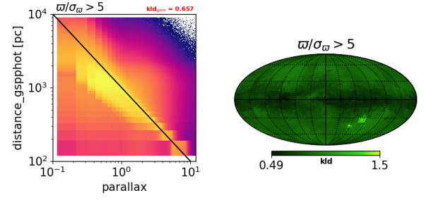
Fig. 37. Global distribution of distance_gspphot against parallax for sources with \varpi/\sigma_\varpi > 5 . The solid black line represents the 1/\text{parallax} relation. The map ( l, b ) on the right shows the sky distribution of the clustering between the two parameters.
