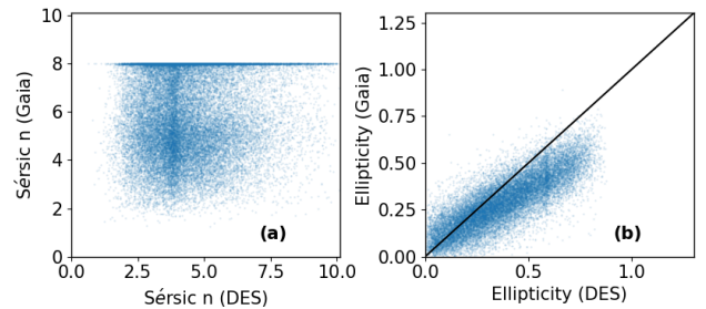
Fig. 45. Comparison of Sérsic index (panel a), and ellipticity (panel b) from DES with the Gaia measurements.
