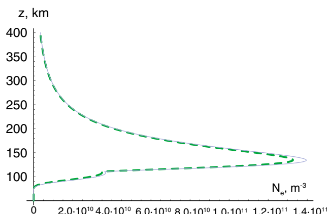
Figure 6. NeMars model ionospheric plasma density profiles for the ending points of satellite orbit portion. Solid line, SZA = 61.293, LAT = 20.658°N; dashed line, SZA = 64.95, LAT = 26.554°N.
