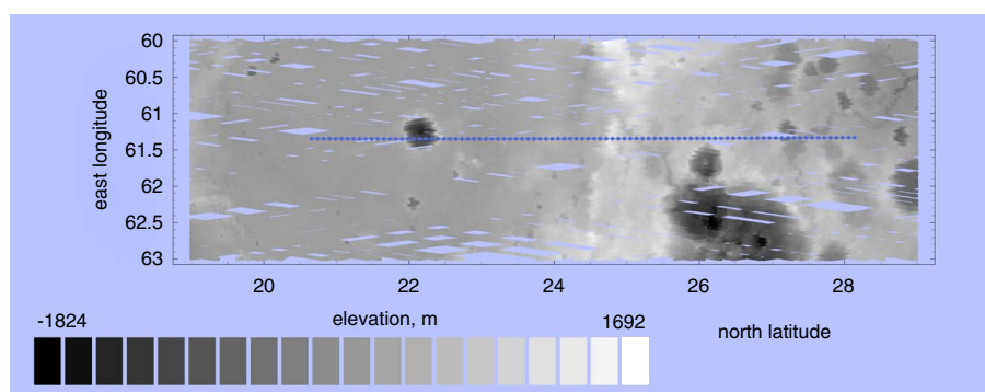
Figure 7. MOLA topography of the Martian underlying surface landscape. Blue dotted line, the southmost part of the MEX orbit 9466 subsatellite track.
