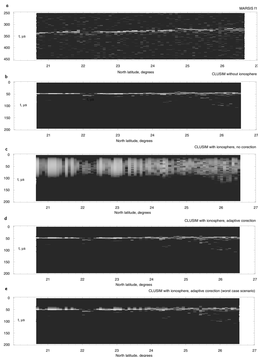
Figure 9. MARSIS radargrams of 9466 MEX orbit. MARSIS Band 4 (4.5–5.5 MHz). (a) Experimental MARSIS radargram, doppler filter 0, working frequency f = 5 MHz (MARSIS band IV), (b) Simulated MARSIS radargram (CLUSIM) without any ionospheric phase shifts, (c) Simulated MARSIS radargram (CLUSIM) with ionospheric phase distortions and no correction, (d) Simulated MARSIS radargram (CLUSIM) with ionospheric phase distortions superimposed and corrected by the maximal contrast adjustment, (e) Simulated MARSIS radargram (CLUSIM) (the same as Figure 9e for the hypothetical “worst case” scenario).
