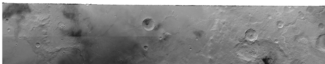
Figure 8. Mosaic of HRSC images H5191_0000_ND3 and H7357_0000_ND3 (Neukum & Jaumann, 2004) depicting the subsatellite landscape of the portion of MEX orbit 9466 under investigation. North is the right of the image.
