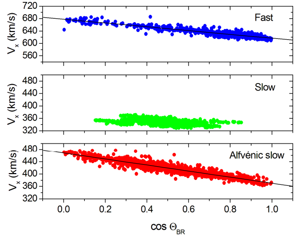
Figure 5. Relationship between \theta_{BR} and V_{sw} for fast and Alfvénic slow solar wind.
