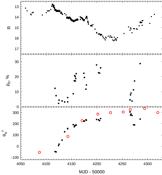
Fig. 9. Optical polarimetric data for 3C 279 obtained during the 2007 campaign. EVPA data for the 43 GHz core are marked with red (open) symbols in the bottom panel. The \pm 180^\circ ambiguity in the EVPAs is resolved by requiring the change across contiguous epochs to be < 90^\circ . No Faraday rotation correction has been applied to the 43 GHz data; see the text.
