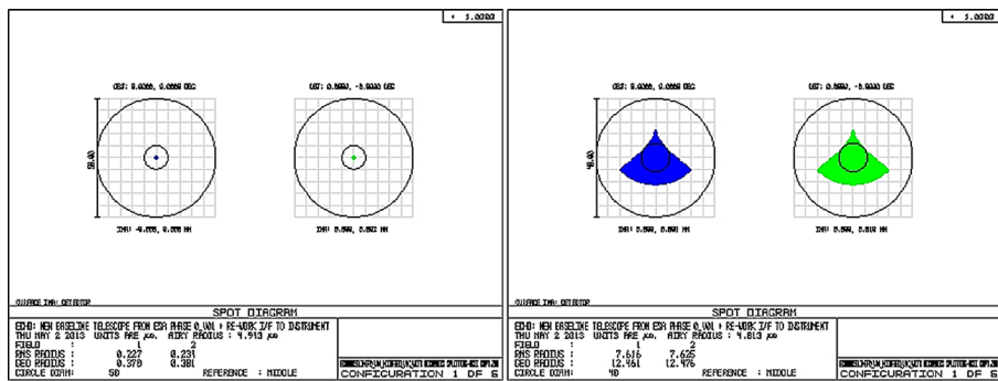
Fig. 9 Spot diagram of focused system in 50 \mu\text{m} at central field 0.0^\circ in blue and marginal field 0.00000278^\circ in green colour (on left side) and Spot diagram of defocused system in 50 \mu\text{m} at central field 0.0^\circ in blue and marginal field 0.00000278^\circ in green colour (right side)
