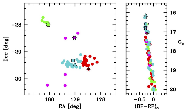
Figure 6. Positions of the spectroscopic targets in the sky map (left panel) and in the CMD (right panel) of PW 1. The targets are plotted with the same empty symbols in both panels. In both panels the filled circles representing the stars of PW 1 are coloured according to the sub-system they belong to: aE (cyan), aW (red), b (green). The stars that are likely members of the system but cannot be attributed to any of these pieces are plotted in magenta.
