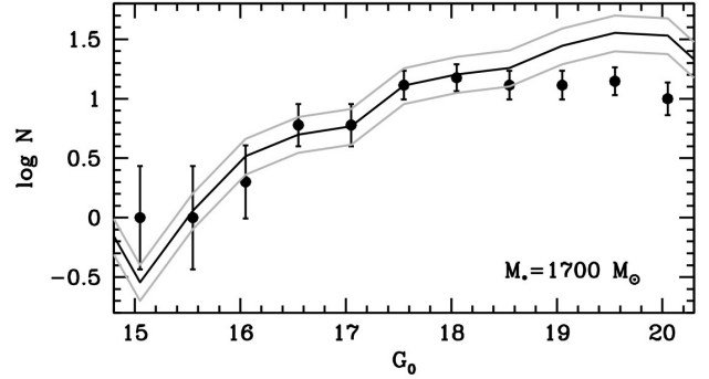
Figure 10. Luminosity Function (LF) of all the PM-selected, parallax-selected and color-selected possible members of PW 1 shown in Fig. 4. The black-line is the theoretical LF from an age = 100 Myr, [M/H] = -1.1 PARSEC model that best-fits the observations in the range G_0 < 18.5 , corresponding to M_* \approx 1700 M_\odot . The grey curves are the theoretical LF adopting different normalisation factors, corresponding to M_* = 2000 M_\odot (upper curve) and to M_* = 1000 M_\odot (lower curve).
