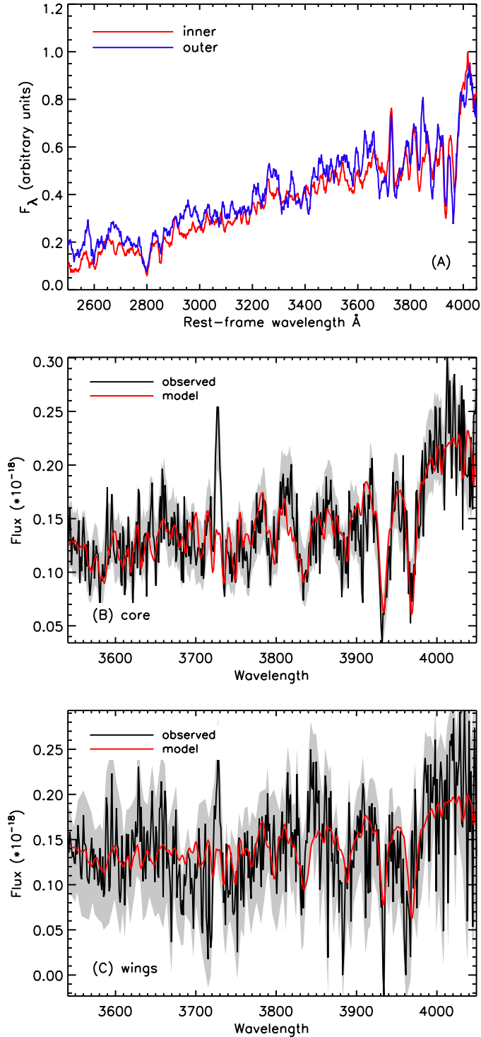
Fig. 7. A) : extracted inner (red) and outer (blue) spectra rebinned to a 10 pixel width. B) and C) : unbinned core and wings spectra, respectively, decomposed according to Eq. (1) (black), with associated uncertainties (gray) and best-fit combination of SSP templates (red).
