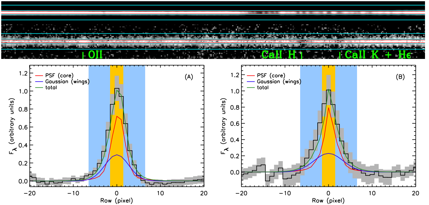
Fig. 5. Top: median 2D spectra of stars (top row) and pBzKs in the range z = 1.2-1.5 (bottom row), in the same wavelength range and using the same relative flux scale. Prominent features in the stacked galaxy spectrum are indicated in green. The red and cyan lines show the inner and outer extraction apertures, respectively. Bottom: cross-dispersion profile of the stacked pBzK spectrum at 3650–4050 Å rest-frame (dark histogram with gray errors), fit with a combination of a point-source (red) and a Gaussian (blue) profile. The inner and outer extraction apertures are indicated by the orange and light blue shaded regions, respectively. Panels A) and B) show, respectively, the cross-dispersion profiles before and after correcting for galaxy morphology. Only the profile shown in panel A) was used for the decomposition and analysis described in Sect. 3.1 and below.
