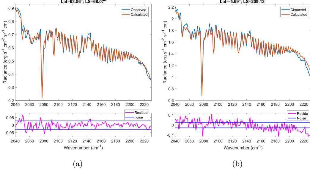
Figure 4: Example fits among the 16 PFS spectra analysed. For the case (a) with the lowest RMS of the residual ( 1.9 \times 10^{-2} \text{ erg s}^{-1} \text{ sr}^{-1} \text{ cm}^{-2} \text{ cm} ) and, (b) the largest RMS ( 4.6 \times 10^{-2} \text{ erg s}^{-1} \text{ sr}^{-1} \text{ cm}^{-2} \text{ cm} ).
