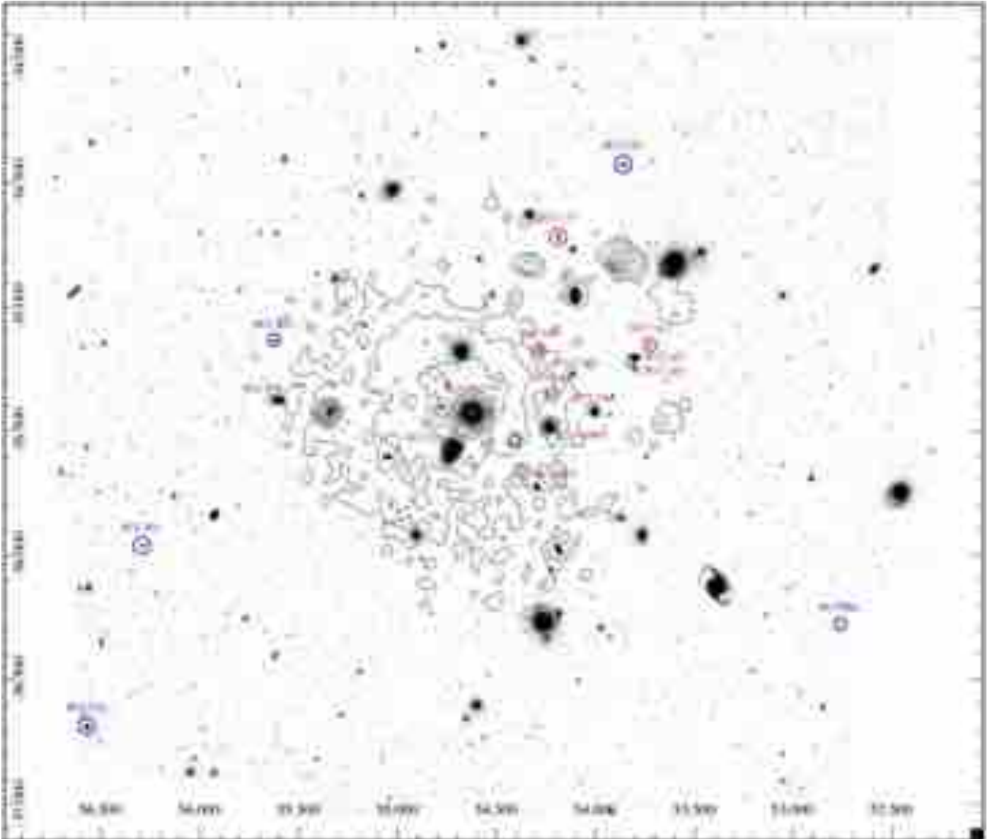
Fig. 2. VST mosaic in the g band of the Fornax cluster inside the virial radius (see Fig. 1). The image size is about 9 square degrees. Black contours are the X-Ray emission from ROSAT (Paolillo et al. 2002). The X-ray contours are spaced by a factor of 1.3, with the lowest level at 3.0 \times 10^{-3} counts arcmin ^{-2} s ^{-1} . All ETGs studied in the present work (see Table 2) are labelled on the image. Galaxies marked with blue symbols have g-i \leq 0.8 mag and g-r \leq 0.4 mag (see Sect. 4 for details). North is up and east is on the left.
