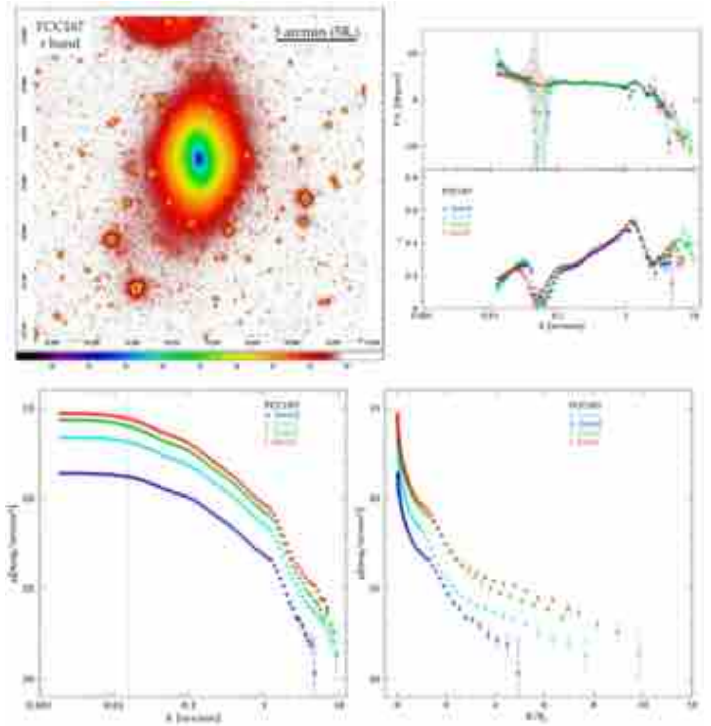
Fig. B.7. Surface photometry for FCC 167.
