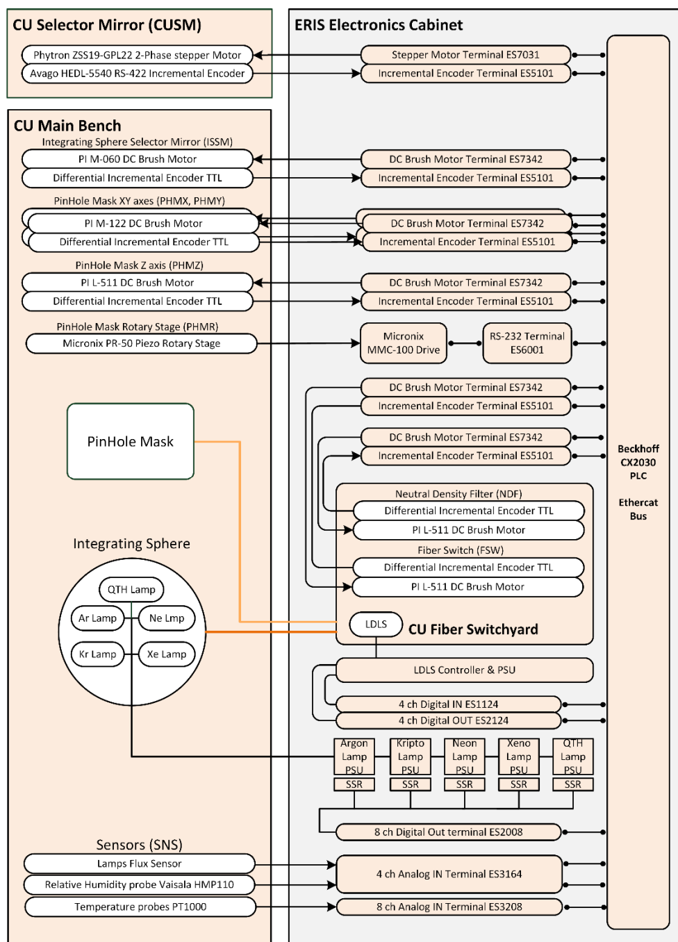
Figure 10. Schematic view of the electronics architecture of the CU. For each component of the instrument electronics (left part of the figure) the corresponding control electronics and connections are shown (right part of the figure).
