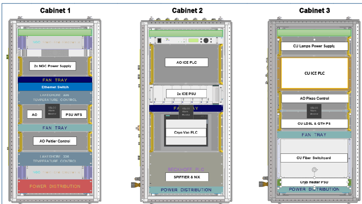
Figure 8. The three moving cabinets mounted on the telescope structure hosting the ERIS Electronics.
