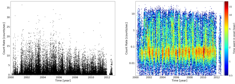
Fig. 5 inFOV-outFOV MOS2 light curves for 13 years of XMM-Newton mission, from 2000 to 2012. (Left) Linear scale on count rate axis shows evidence for evolution of the SP flaring background through the mission. (Right) Logarithmic scale on count rate axis focuses on the low-intensity background component (located in the denser region).
