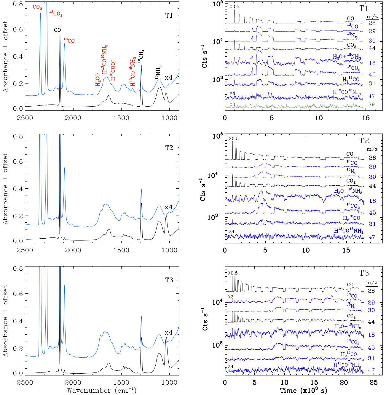
Figure 1. Left panels: infrared spectra of the ices for the experiments T1 (top), T2 (middle), and T3 (bottom), before (black lines) and after irradiation (blue lines, multiplied by 4). Right panels: main photodesorbing fragments detected by the QMS during soft X-ray irradiation for the three experiments. CO ( m/z = 28 ) and \text{CO}_2 ( m/z = 44 ) (black curves) come from the top layer. ^{13}\text{CO} ( m/z = 29 ), ^{13}\text{CO}_2 ( m/z = 45 ), ^{15}\text{N}_2 ( m/z = 30 ), \text{H}_2^{13}\text{CO} ( m/z = 31 ), \text{H}_2\text{O} and ^{15}\text{NH}_3 ( m/z = 18 ), and \text{H}^{13}\text{CO}^{15}\text{NH}_2 and possibly \text{H}^{13}\text{COOH} ( m/z = 47 ) come from the bottom layer. For comparison with m/z = 47 , the top panel shows the spectrum of m/z = 79 (green line), a value at which no species are expected.
