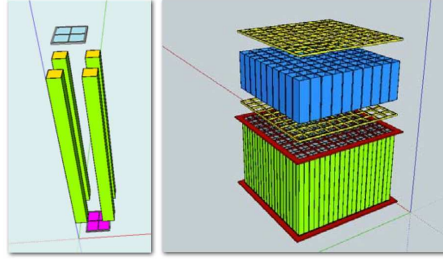
Fig. 2. The XGS concept. Left panel: basic unit of the module, composed by 4 CsI(Tl) bars and two 2x2 single-cell SDD arrays. Right panel: the complete XGS module, showing also a field of view collimator for X-rays.
