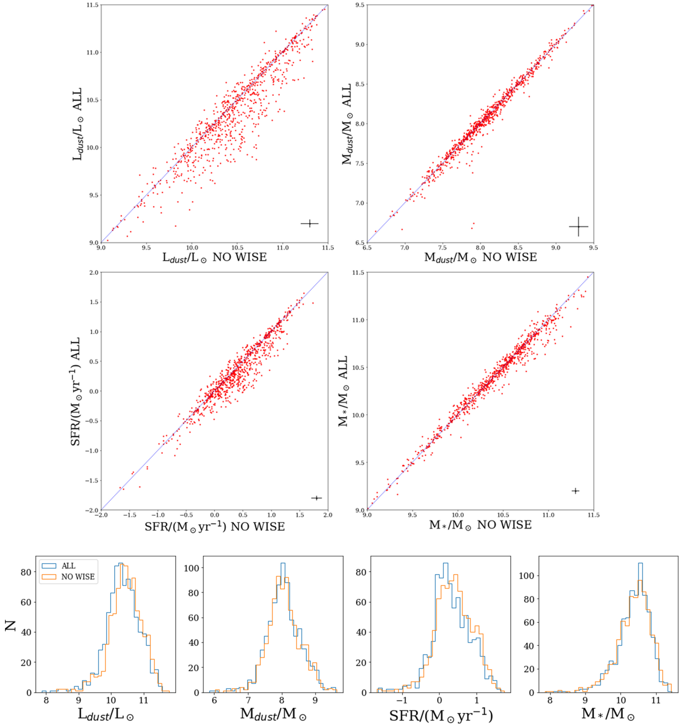
Fig. 1. Top panels: dust luminosity ( L_d , top left), dust mass ( M_d , top right), SFR (bottom left), and stellar mass ( M_{\star} , bottom right) obtained with CIGALE (Noll et al. 2009; Boquien et al. 2019) from the sample defined in Sect. 2 using the full photometric coverage (ordinate) or removing WISE data (abscissa). The blue dashed line shows a linear relation between the two quantities and the black cross in the bottom right corner shows the average errors in the fits. Bottom panels: histograms of the same quantities.
