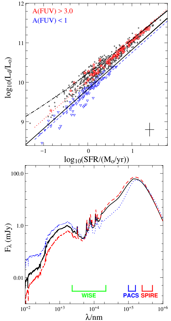
Fig. 8. Top panel: dust luminosity ( L_d ) as a function of the SFR obtained with CIGALE (Noll et al. 2009) using the full photometric coverage. Red stars and blue triangles identify galaxies with A(\text{FUV}) > 3.0 and A(\text{FUV}) < 1 , with their best fit shown as red dotted and blue dashed lines, respectively. Red dotted and blue dashed lines show the best fit for the galaxies showing high and low levels of extinction, respectively. The solid and dot-dashed black lines show the SFR as derived from Eqs. (1) (Kennicutt 1998) and (2) (Clemens et al. 2013), respectively. Bottom panel: median SED obtained using the full photometric coverage (black solid line), considering the galaxies with A(\text{FUV}) > 3.0 (red dashed line) and A(\text{FUV}) < 1 (blue dotted line). The photometric coverage of WISE, PACS, and SPIRE bands is shown at the bottom.
