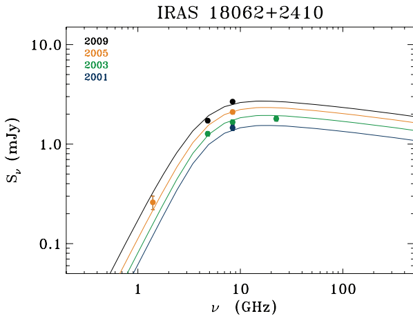
Figure 3. Radio continuum spectra of IRAS 18062+2410 obtained at different epochs. The correspondent spectra model curves are shown in the same colour as the data points.
