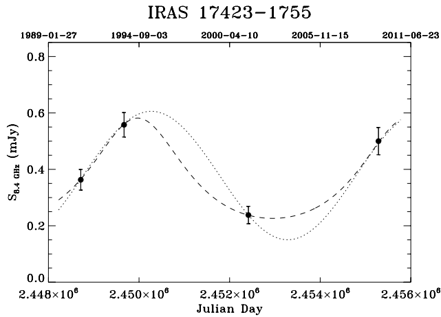
Figure 2. VLA observations at 8.4 GHz of IRAS 17423–1755 over 16 yr. The point in 1991 is from the VLA project AK247 (PI: Knapp), while that in 1993 is from AZ63 (PI: Zijlstra).
