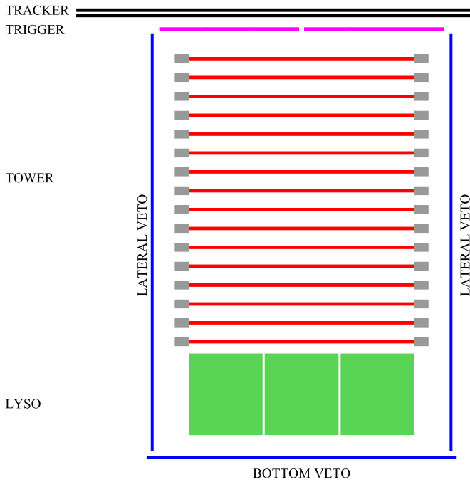
Figure 1. Schematic view of the HEPD apparatus: in the picture, the lateral veto plane located in the front has been removed for the purpose of visualization.
