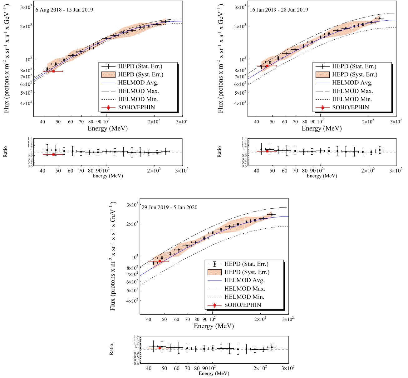
Figure 6. Large panel: galactic proton spectra as a function of energy measured by HEPD in the three intervals described in the text (from 2018 August 6 to 2019 January 15, from 2019 January 16 to 2019 June 28, and from 2019 June 29 to 2020 January 5, respectively). Systematic uncertainties are also present as a yellow shaded area. The continuous curves represent, respectively, the HelMod theoretical spectrum averaged over the period under study (blue solid line), the maximum (dashed line) and minimum (dotted line) expected deviation from the model itself. The red square represents data obtained from the SOHO/EPHIN spacecraft. Narrow panel: ratio between HEPD data and HelMod model, as a function of energy; errors on HEPD data are a sum of statistical and systematic uncertainties.
