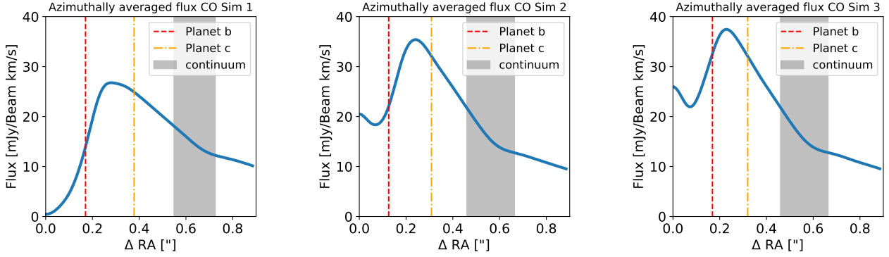
Figure 8. Azimuthally averaged ^{12}\text{CO} moment zero maps (continuum subtracted) for all the simulations (left: Sim 1, middle: Sim 2, right: Sim 3) for the t = 500 T_{\text{orb}} snapshot. The position of Planet b and c is shown as the red and orange vertical line respectively, while the grey region shows the extent of the continuum ring.
