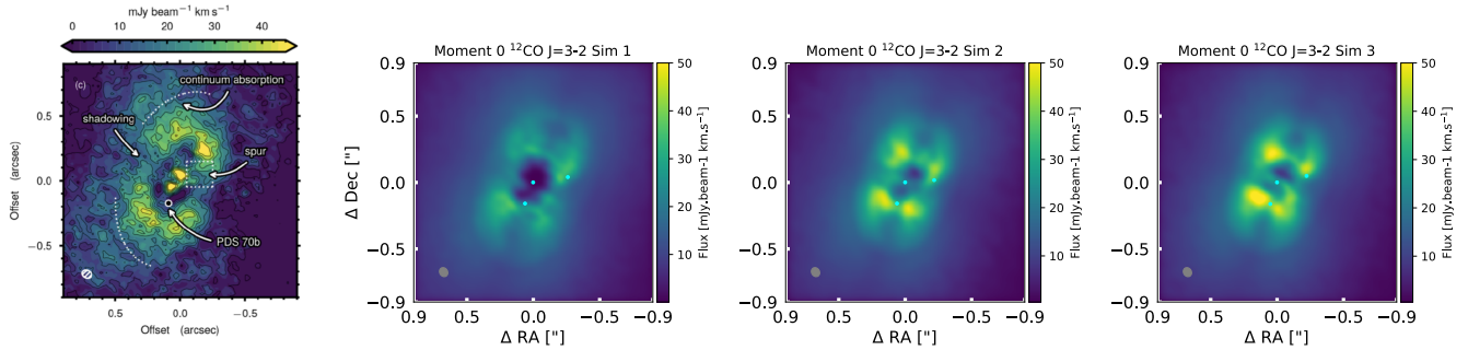
Figure 7. CO J=3-2 integrated intensity (moment 0, continuum subtracted) for all the simulations for the t = 500 T_{\text{orb}} snapshot and, as a reference, the observed image of Keppler et al. (2019) (left). The position of the star and the planets is shown as cyan dots. The image is convolved with a Gaussian 76 \times 61 mas beam with PA of 63 degrees as in Keppler et al. (2019) observations.
