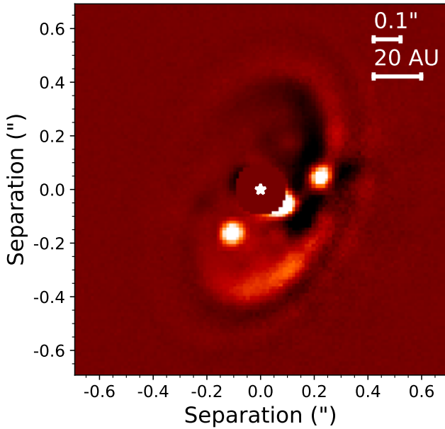
Figure A1. Differential image obtained by subtracting the predicted scattered light image at 2.11/2.25 \mu\text{m} when the location of planet c is 180 degrees from the observed one to the predicted image where the planets are at their observed position. This highlights the faint spiral accretion stream induced by planet c.
