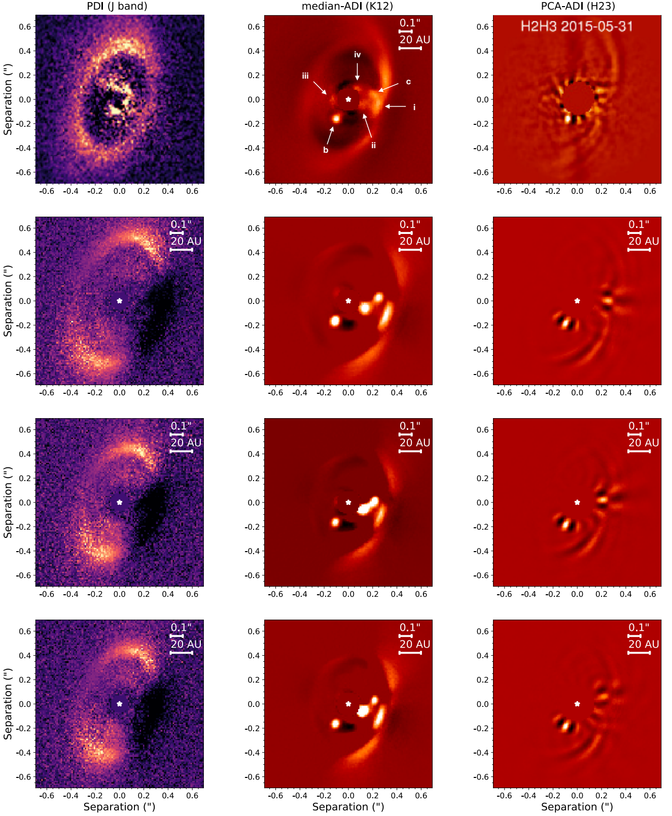
Figure B1. Near infrared observations of PDS 70 (top row) compared to the processed IR predictions obtained from simulations 1, 2 and 3 (second, third and last row, respectively). Left column: Polarimetric Differential Imaging predictions in J band ( 1.25\ \mu\text{m} ). Middle column: average median-ADI images over the K1 and K2 bands ( 2.11/2.25\ \mu\text{m} ). Right column: average PCA-ADI images over the H2 and H3 bands ( 1.59/1.67\ \mu\text{m} ), obtained with 5 principal components subtracted.
