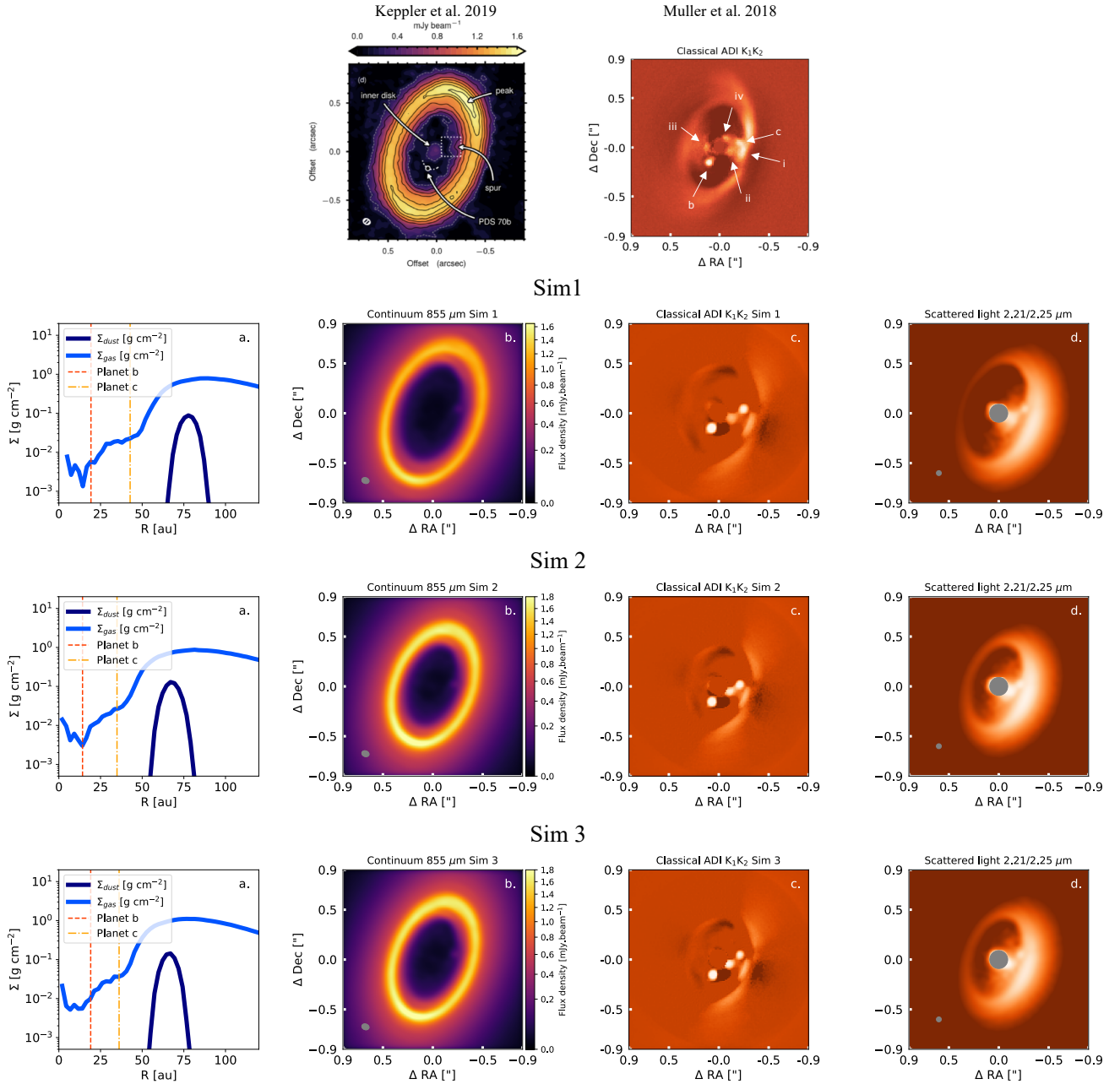
Figure 3. Comparison between our three simulations (bottom three rows) and observations from Keppler et al. (2019) and Müller et al. (2018) (top row). Panels a show the surface density profile of gas (light blue) and dust (blue) plotted as a function of radius for the t = 500 T_{\text{orb}} snapshot for the three simulations (1 to 3 from top to bottom), in units \text{g cm}^{-2} and au respectively. Instantaneous planets positions are also plotted as red and orange vertical lines. Panels b show the corresponding simulated continuum image at 855 \mu\text{m} , with fluxes in \text{Jy beam}^{-1} . The image has been smoothed with a 74 \times 53 mas Gaussian beam to match the beam size of ( Keppler et al. 2019 ). Panels c and d show the average between the 2.11/2.15 \mu\text{m} scattered light images with and without median-ADI processing, respectively. In panels c the flux of the planets were injected in the ADI cube before processing, while panels d do not include emission/heating from the planets. The flux density is in \text{Jy/arcsec}^{-2} and the image has been convolved with a psf of 0.05 mas.
