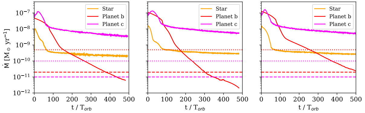
Figure 9. Accretion rates (in M_{\odot} \text{ yr}^{-1} ) onto the sinks for all the simulations (left: Sim 1, middle: Sim 2, right: Sim 3) as a function of the normalized time. Orange lines are the star accretion rate and red and pink lines are Planet b and Planet c accretion rates respectively. Horizontal red and pink dashed lines show the inferred values from Planet b and c respectively from Haffert et al. (2019) , while the horizontal red and pink dotted lines show the inferred values from Planet b and c from Hashimoto et al. (2020) .
