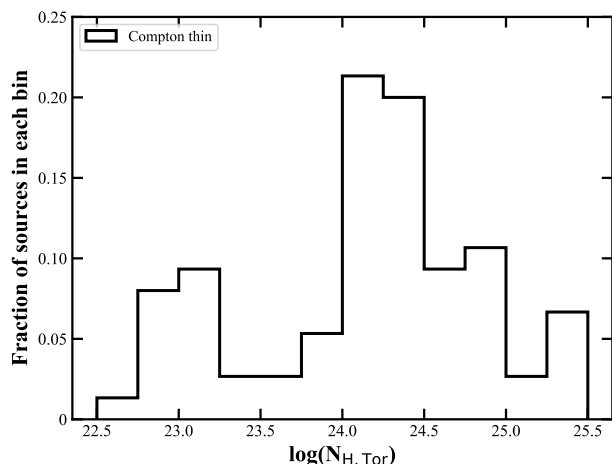
Fig. 3. Torus average column density distribution of the sources in our unbiased Compton thin AGN sample. The histogram describes the same sample as in the upper right panel of Fig. 1 but with different grouping bins.
