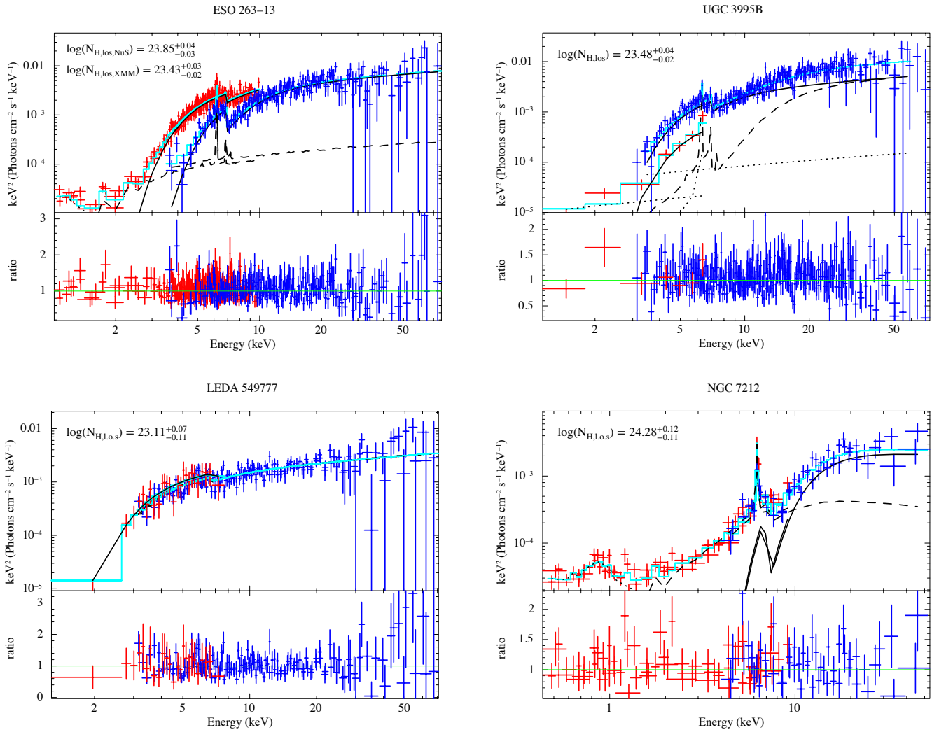
Fig. A.1. Spectra and ratio (between the data and model predictions) of ESO 263-13 (XMM-Newton+NuSTAR), UCG 3995B (Chandra+NuSTAR), LEDA 549777 (Swift-XRT+NuSTAR) and NGC 7212 (in M19 sample). NuSTAR and soft X-ray data are plotted in blue and red, respectively. The total best-fit model predictions and different components of the models of are plotted in cyan black, respectively. The reprocessed component, line-of-sight component, and scattered (& Mekeal) component are plotted in dashed, solid, and dot lines, respectively. Significant flux variabilities are found in ESO 263-13 and UCG 3995B.
