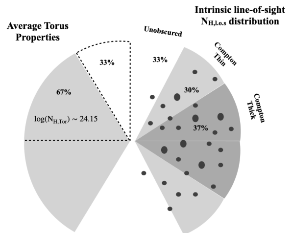
Fig. 5. The left part of the figure presents that the average torus properties of our unbiased Compton thin sample; The right part of the figure illustrates the intrinsic line-of-sight column density distribution derived from our new developed method.
