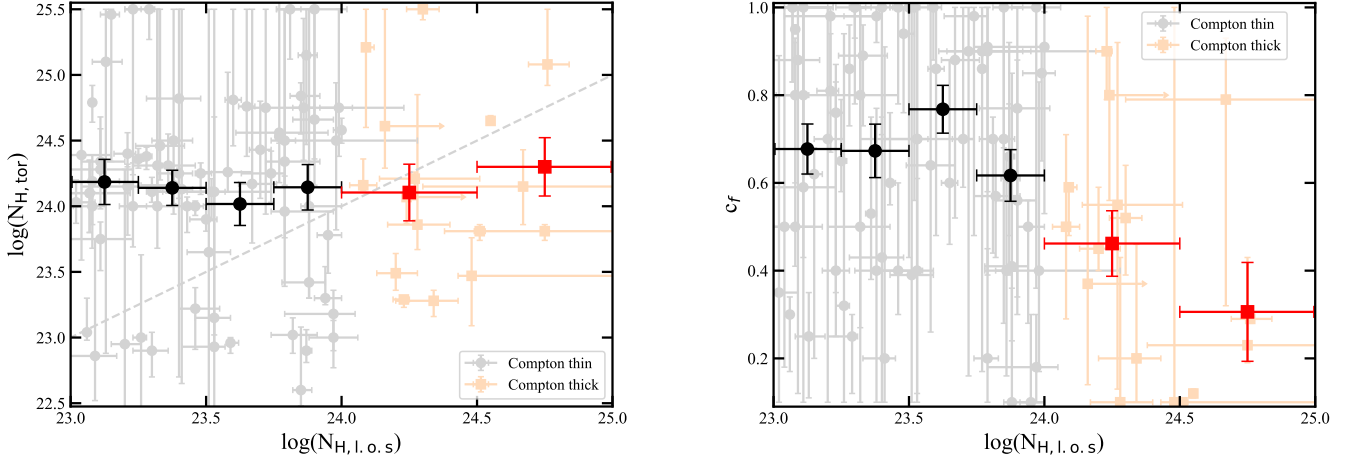
Fig. 2. Torus column density \log(N_{H,\text{tor}}) (left) and torus covering factor c_f (right) as a function of line-of-sight column density, \log(N_{H,\text{l.o.s}}) . Compton thin sources are plotted in light grey points, while CT sources are plotted in light red squares. The average and 1\sigma standard error of the torus column densities and torus covering factors in different line-of-sight column density bins are plotted in black points for Compton thin sources and red squares for CT sources, respectively. In the left panel, N_{H,\text{tor}} = N_{H,\text{l.o.s}} is plotted as a light grey dashed line. The low covering factors of the CT sources are due to the bias explained in Sec. 3.
