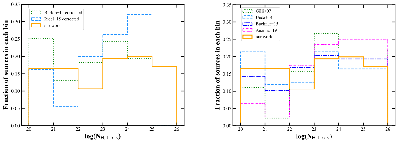
Fig. 4. Comparison between the intrinsic line-of-sight column density distribution derived from our new developed method with previous observational results (left) and those used in different population synthesis models (right). The extremely obscured sources with \log(N_{\text{H}, \text{l.o.s}}) > 26 are included in the 25 < \log(N_{\text{H}, \text{l.o.s}}) < 26 bin.
