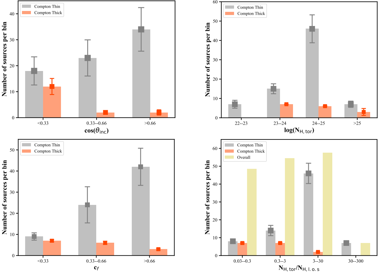
Fig. 1. The figures from left to right in the first row and second row are the number of sources with a specific range of the inclination angles, \cos(\theta_{\text{inc}}) , torus column densities, \log(N_{\text{H,tor}}) , torus covering factors, c_f , and the torus column density contrast ratio, N_{\text{H,tor}}/N_{\text{H,l.o.s}} , of Compton thin sources in our sample (grey histogram) and CT sources from M19 (orange histogram), respectively. \cos(\theta_{\text{inc}}) \sim 0.05 is when the AGN is observed in ‘edge-on’ direction and \cos(\theta_{\text{inc}}) \sim 0.95 is when the AGN is observed ‘face-on’. The error bar is at 90% confidence level. The overall distribution of torus column density contrast ratio after rescaling is plotted in yellow. We do not include the 15 sources fitted with only a line-of-sight component and a scattered component here.
