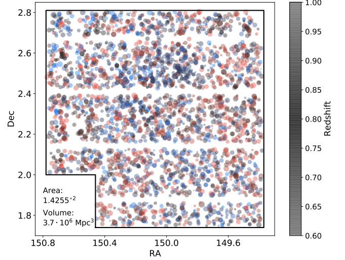
Figure 2. Survey footprint and source distribution in the COSMOS field. Symbol size reflects the stellar velocity dispersion (Section 3.2) in order to emphasize the more massive galaxies.
