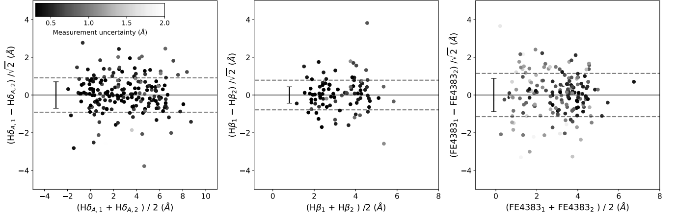
Figure C2. Comparison of duplicate measurements of 3 absorption line indices (LICK.H \delta _A, LICK.H \beta , LICK.FE4383). See Fig. C1 caption and text for details.
