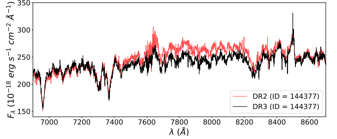
Figure 3. Example comparison of DR2 (red) and DR3 (black) versions of the same spectrum, illustrating the improvements and changes to the data processing techniques. The overall normalization is affected (on the level of a few percent) by the zero point changes in the photometry used for the flux calibration (Appendix B). The shape of the continuum is affected by the changes in the photometric SED fit (2.2.3). The improved telluric absorption correction (2.2.2) is most clearly seen in the wavelength range 7600 - 7700 \text{ \AA} , where the systematic residual in the form of high-frequency ‘beating’ is reduced in the DR3 version of the spectrum.
