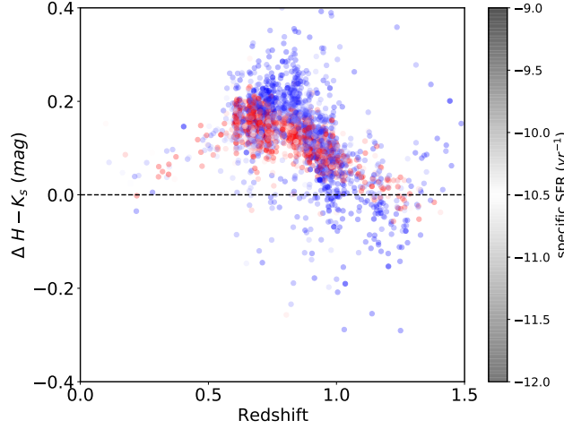
Figure B4. Difference between observed H - K_s color and inferred H - K_s based on fits to the BVrizYJ photometry. Color coding is with specific star formation rate: red colors indicate passive galaxies; blue colors indicate high star-formation activity. The strong redshift dependence indicates the offsets are not due to a simple calibration error in the photometry (which would lead to a redshift-independent offset). The small difference between young (star-forming) and old (quiescent) galaxies that the offsets are not strongly age dependent.
