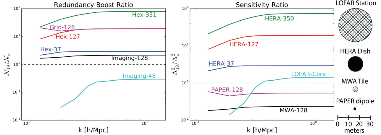
Figure 12. Left: Representative boost factors ( \mathcal{N} in Eq. 4) normalized to a 19-element hexagonal configuration spaced at 14.6 m. For a given element count, one can get about an order of magnitude improvement in delay-spectrum sensitivity. Alternatively, for the same sensitivity one can build roughly 1/3 the antennas. Right: Power spectrum sensitivities for various arrays normalized to HERA-19. The element sizes are indicated at the far right with appropriately sized circles. Cross-hatching denotes phased tiles.
