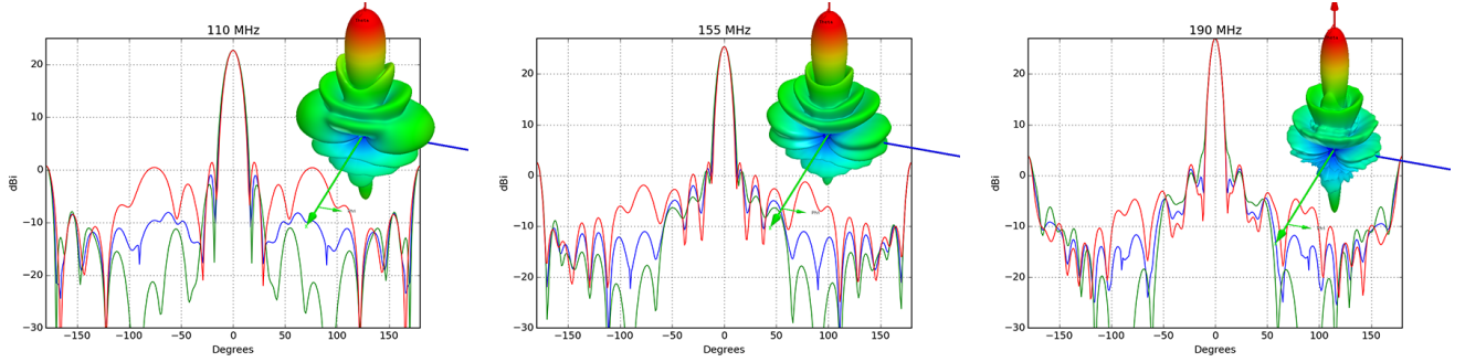
Figure 19. Antenna patterns at 110 MHz, 155 MHz and 190 MHz calculated with HFSS and the adopted design. Red curves are E-plane, green are H-plane at blue at 45°. Inset is the full 3D pattern.
