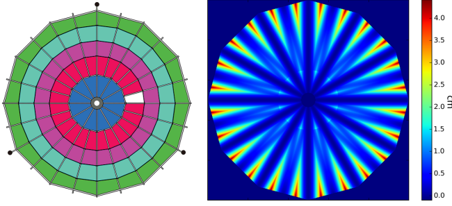
Figure 17. Element panel plan (left) and residual from a true paraboloid (right). The white panel denotes the location of the door.
