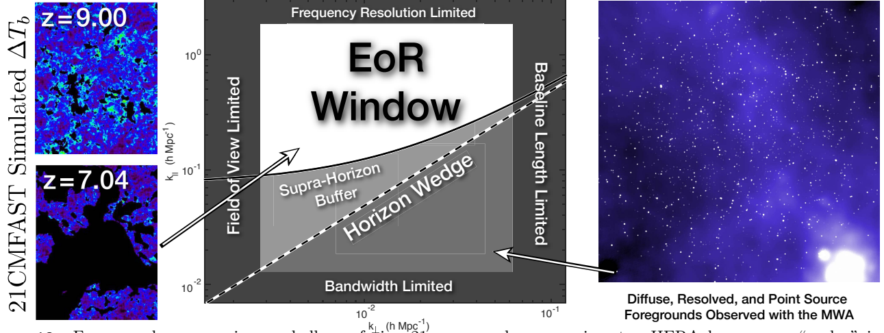
Figure 10. Foregrounds are a primary challenge facing 21 cm cosmology experiments. HERA leverages a “wedge” in the cylindrically-averaged ( \mathbf{k} is broken into k_{\parallel} and k_{\perp} ) power spectrum (center panel). Smooth-spectrum foregrounds (right panel) \sim 3 - 5 orders of magnitude brighter than fiducial EoR models (left panel; Mesinger et al. 2011 ) create the “wedge” when they interact with the interferometer’s chromatic response. Flat spectrum foregrounds cannot contaminate the EoR window beyond the horizon wedge, though intrinsic or imperfectly calibrated chromaticity can push it slightly beyond the horizon. By avoiding foregrounds, PAPER has placed limits within an order of magnitude (in mK) of these models ( Ali et al. 2015 ) and shown the “EoR Window” to be foreground-free. HERA’s dish and compact configuration optimize wedge/window isolation and direct sensitivity to low- k_{\perp} modes where the EoR is brightest relative to the foreground wedge.
