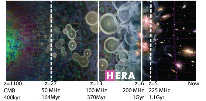
Figure 2. Rendering of cosmic evolution from just after the Big Bang to today (background image credit Loeb/ Scientific American ). The labels show the redshift and the frequency of the red-shifted hydrogen line (rest frequency 1420 MHz) at different ages of the Universe. The solid white lines bracket the HERA EOR band and the dashed ones bracket the extended frequency goal. CMB observations observe the afterglow of the Big Bang (far left) and Baryonic Acoustic Oscillation (BAO) surveys proposed target z \approx 0.8 -2.5. Limited surveys span back to about z \approx 7 .
