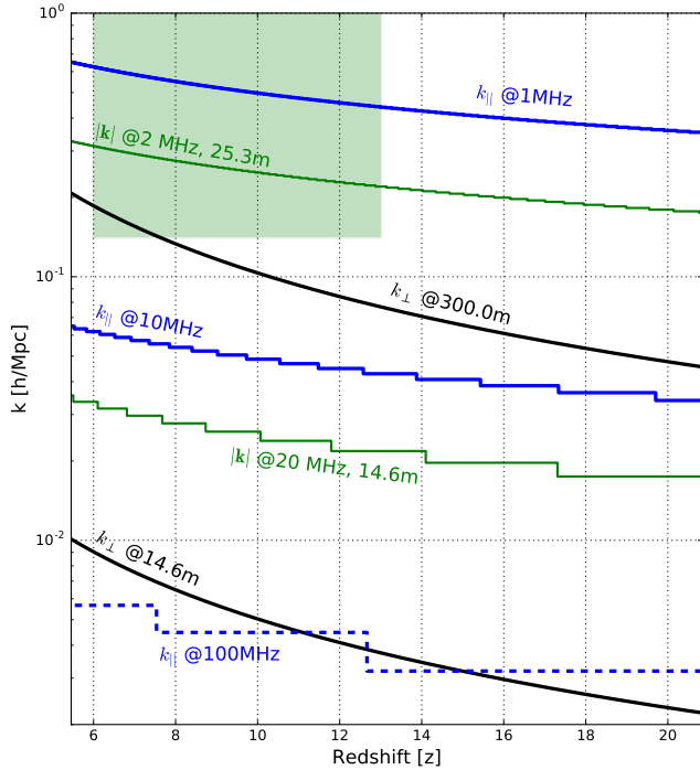
Figure 11. |\mathbf{k}|, k_{\parallel}, k_{\perp} wavenumber plots at various bandwidths ( k_{\parallel} ; blue), baselines ( k_{\perp} ; black), and total ( |\mathbf{k}| , green) as a function of redshift. The stepped profiles for k_{\parallel} and |\mathbf{k}| are the line-of-sight redshift ranges for that bandwidth (too small to see at 1 MHz). See text for discussion. The full redshift range is the HERA extended goal. The initial HERA delay-spectrum power spectrum goal is the light green square region in the upper left.
