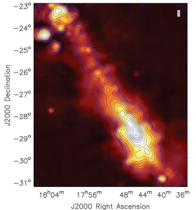
Figure 8. The color-scale shows an input model image of the Galactic center region based on the Effelsberg 21cm continuum survey (Reich et al. 1990). The contours show the mock HERA-350 observation at 130MHz with a resolution of 12' . Contour levels are a geometric progression in square root 2, starting at 5 \text{ Jy beam}^{-1} . The peak surface brightness on the HERA image is 2330 \text{ Jy beam}^{-1} .
