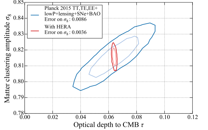
Figure 6. Likelihood contours (68% and 95%) for \sigma_8 and \tau using Planck constraints (blue) and adding HERA data (red). The 21 cm constraints break the CMB degeneracy between the amplitude of density fluctuations and the optical depth, improving constraints on both.
