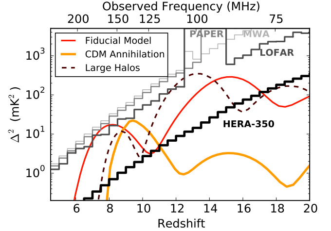
Figure 4. 1\sigma thermal noise errors on \Delta^2(k) , the 21 cm power spectrum, at k = 0.2 h \text{ Mpc}^{-1} (the dominant error at that k ) with 1080 hours of integration (black) compared with various heating and reionization models (colored). Sensitivity analysis is per Table 1 and associated text.
