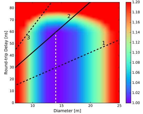
Figure 13. The background coloring with colorbar shows the relative cost/performance for delay and cost at a fixed performance as a function of element diameter. See §4.3, §4.4 and DeBoer & Parsons (2015) for details. A diameter of 14-m (vertical dashed line) is near the cost minimum and consistent with assumptions for the delay specification.
