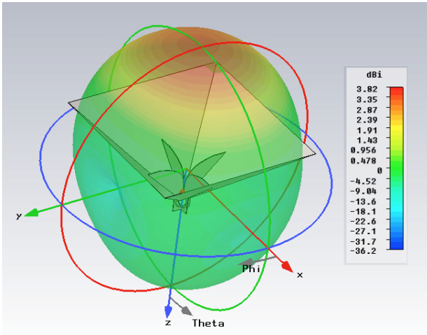
Figure 20. Future potential HERA feed showing its directive beam pointed towards the dish. It is based on a modified ridge TEM horn and is currently under investigation at Cambridge University.
