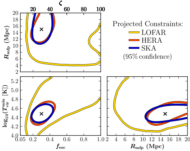
Figure 5. Projected likelihood contours from an MCMC analysis for astrophysical parameters of reionization. Model parameters are T_{\text{vir}}^{\text{min}} (minimum virial temperature of ionizing galaxies); R_{\text{mfp}} (mean free path of ionizing photons in HII regions); and \zeta_0 (ionizing efficiency of galaxies). Also shown are constraints on the derived ionizing escape fraction, f_{\text{esc}} . Adapted from Greig & Mesinger (2015).
