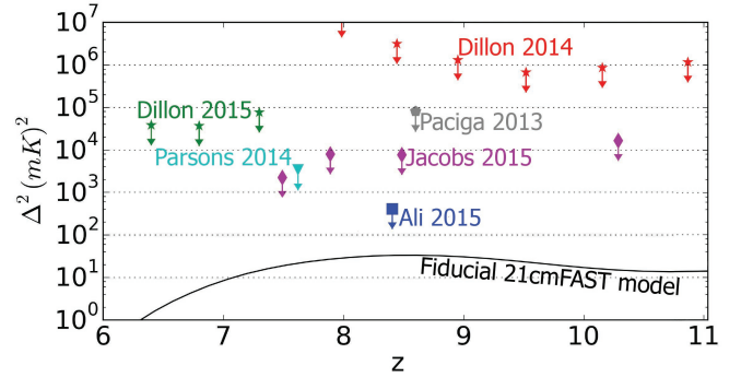
Figure 9. The current best published 2\sigma upper limits on the 21cm power spectrum, \Delta^2(k) , compared to a 21cmFAST-generated model at k = 0.2 h \text{ Mpc}^{-1} . Analysis is still underway on PAPER and MWA observations that approach their projected full sensitivities; HERA can deliver sub-mK 2 sensitivities.
