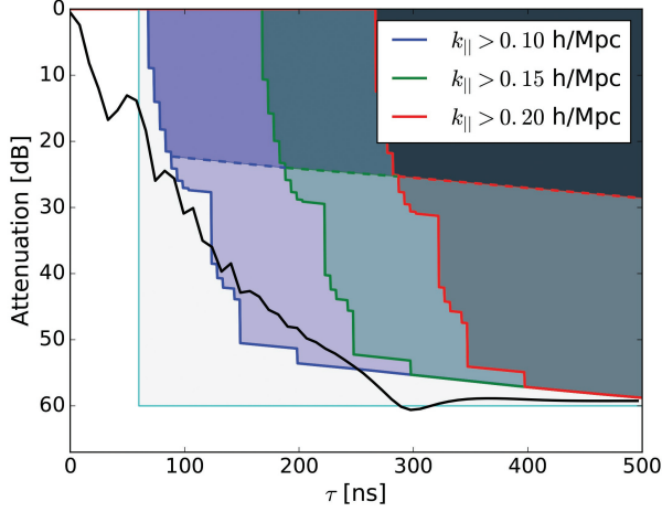
Figure 14. Antenna delay attenuation specification with realistic foregrounds from Thyagarajan et al. (2016) . The blue, green and red lines show the maximum attenuation needed at a given delay for the foregrounds to be below the expected EOR signal level for different k_{||} . The lower lines are for the worst case with no additional processing, while the dashed line assumes inverse covariance weighting. The teal line is the 60 dB by 60 ns initial conservative specification. HFSS calculations (black line) for the expected attenuation show the HERA dish meeting the more sophisticated specification for k_{||} \gtrsim 0.15 \text{ h Mpc}^{-1} .
