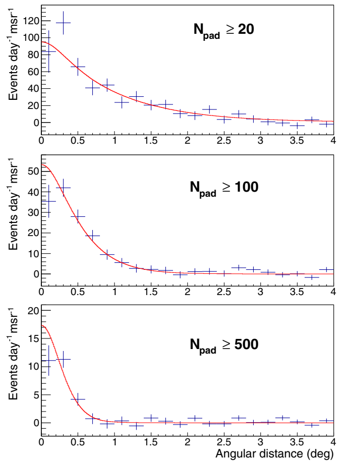
Figure 5. Comparison of experimental and simulated PSFs: event rate per solid angle as a function of the angular distance from the source position, for events with N_{\text{pad}} \geq 20, 100 , and 500 . The solid lines are the results of the simulation.
