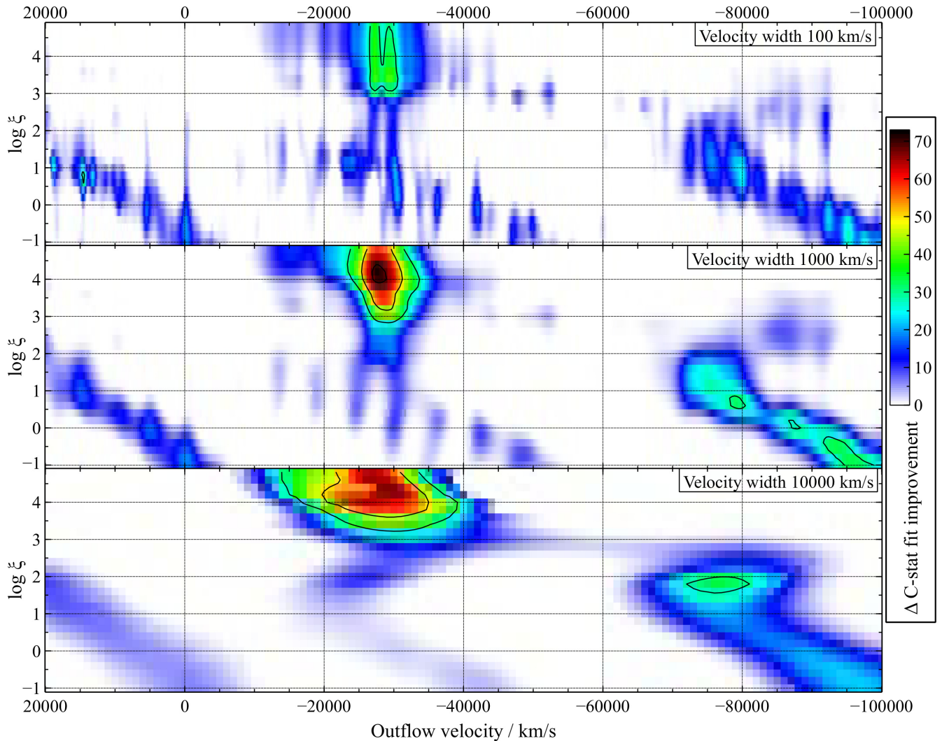
Figure 5. Systematic scan for ionized outflow features in the spectrum of PG 1448+273. The spectrum is scanned with ionized absorption model grids with systematic velocities between +20 000 and −100 000 km s −1 (on the X-axis), ionization parameters log \xi between −1.0 and +4.8 (on the Y-axis), with turbulent velocities of 100 km s −1 (top subplot), 1000 km s −1 (middle subplot), and 10 000 km s −1 (bottom subplot). The colour shows the \Delta C-stat fit improvement upon adding the absorption grid to the baseline continuum model (according to the colour bar on the right), and the black contours show \Delta C-stat fit improvement of 30, 50, and 70, respectively.
