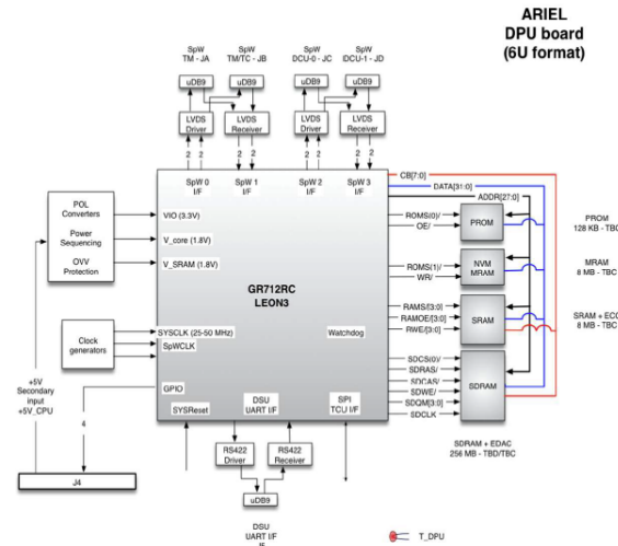
Figure 1: a possible configuration of the CDPU, hosting the GR712RC Leon 3 dual-core processor and different kinds of memories.
