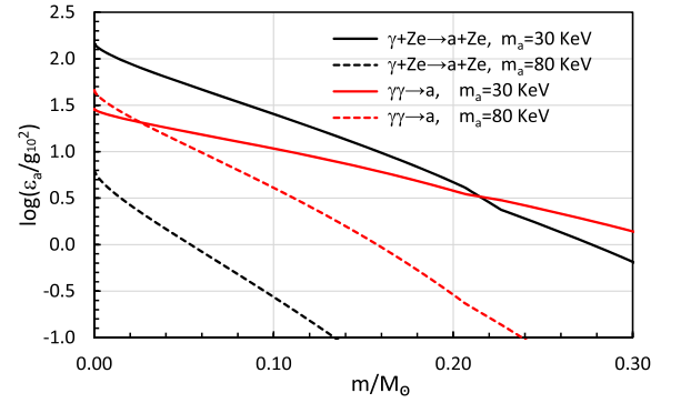
Fig. 2. Energy-loss rates (in units of \text{erg g}^{-1} \text{s}^{-1} and normalized for g_{10} = 1 ) for Primakoff ( \gamma + Ze \rightarrow a + Ze ) and photon coalescence ( \gamma\gamma \rightarrow a ) within the core of a typical HB star. The most internal 0.3 M_\odot is shown. This is the same model used for Fig. 1. Results for two different axion mass, m_a = 30 keV and m_a = 80 keV, are shown.
