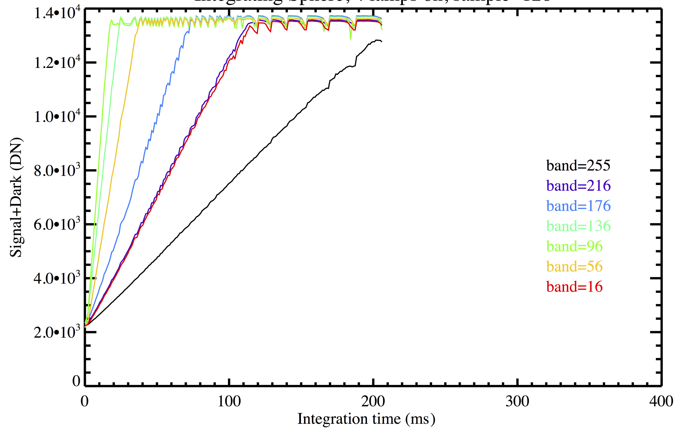
Integrating Sphere, 2 lamps on, sample=128
