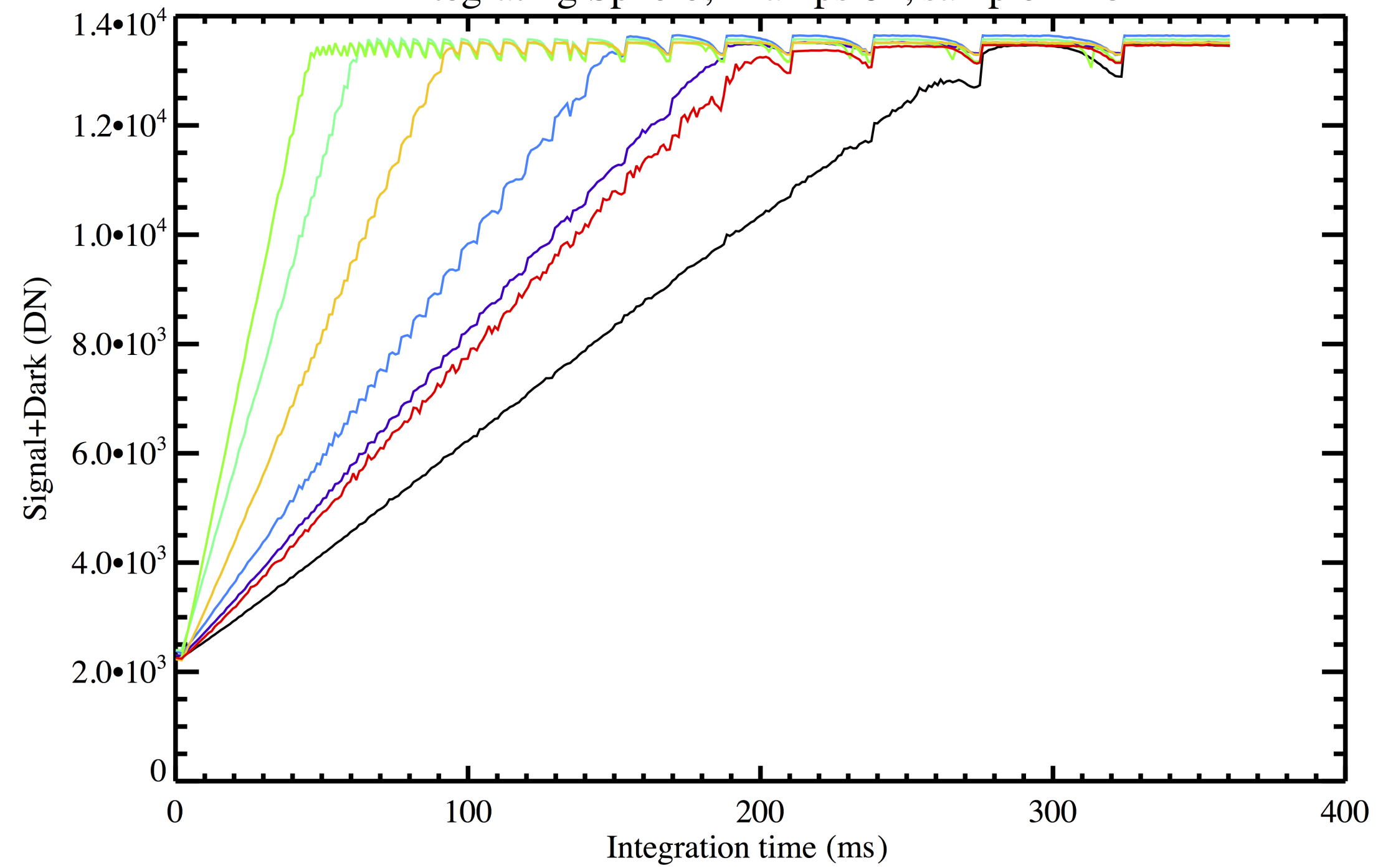
Integrating Sphere, 1 lamps on, sample=128
