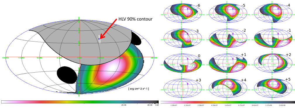
Fig. 5 Left panel: the GRID 2\sigma UL map (in 30 MeV – 10 GeV) on 4 s integration around the GW170817 T_0 , showing the LR occulted by the Earth. Maps are in Galactic coordinates; the 90% c.l. LR of GW170817 is marked in white color; the sky region occulted by the Earth is shown in gray color while the Sun inaccessible region is in black. Right panel: the 150 s exposure UL map scan preceding and following T_0 evaluated at the optical transient position. Maps are in Galactic coordinates; the GW170817 90% c.l. LR is marked in magenta color.
