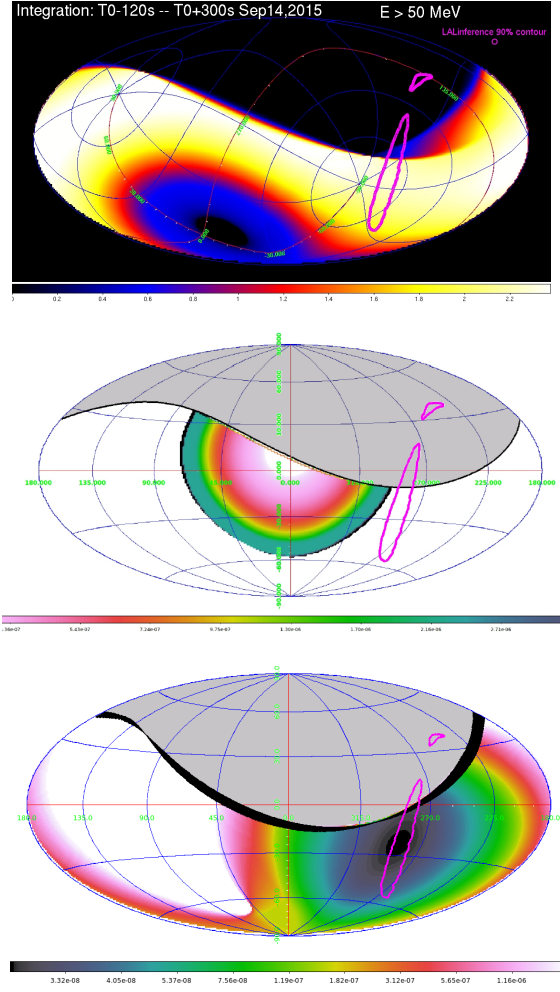
Fig. 1 The AGILE-GRID observations of the first announced GW event, GW150914. Maps are in Galactic coordinates; the 90% confidence level localization region (LR) of GW150914 is marked in magenta color; the sky region occulted by the Earth is shown in gray color. Top panel: Aitoff exposure map in the 50 MeV – 10 GeV energy band for a 7-minute integration from -120 s to +300 s (with respect to T_0 ). Middle panel: Aitoff map of GRID upper limits (ULs) obtained with a 4 s integration near the GW150914 T_0 . The AGILE GRID just missed exposing the GW event LR in this case. Bottom panel: Aitoff map of the GRID ULs map obtained for the first available coverage of a substantial fraction of the GW event LR, which occurred at +330 s after T_0 .
