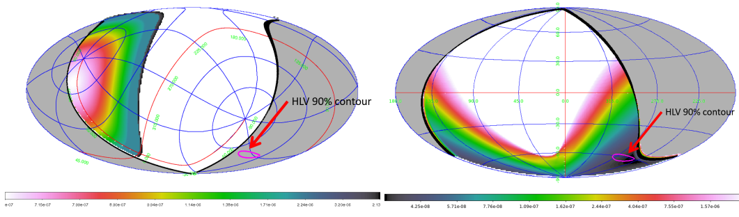
Fig. 4 Left panel: the GRID 3\sigma UL map (in 50 MeV – 10 GeV) on 4 s integration around the GW170814 T_0 showing Earth occultation of the event LR. Right panel: the 100 s best exposure of the LR at +550 s after T_0 , with a complete coverage. Maps are in Galactic coordinates; the 90% c.l. LR of GW170814 is marked in magenta color; the sky region occulted by the Earth is shown in gray color.
