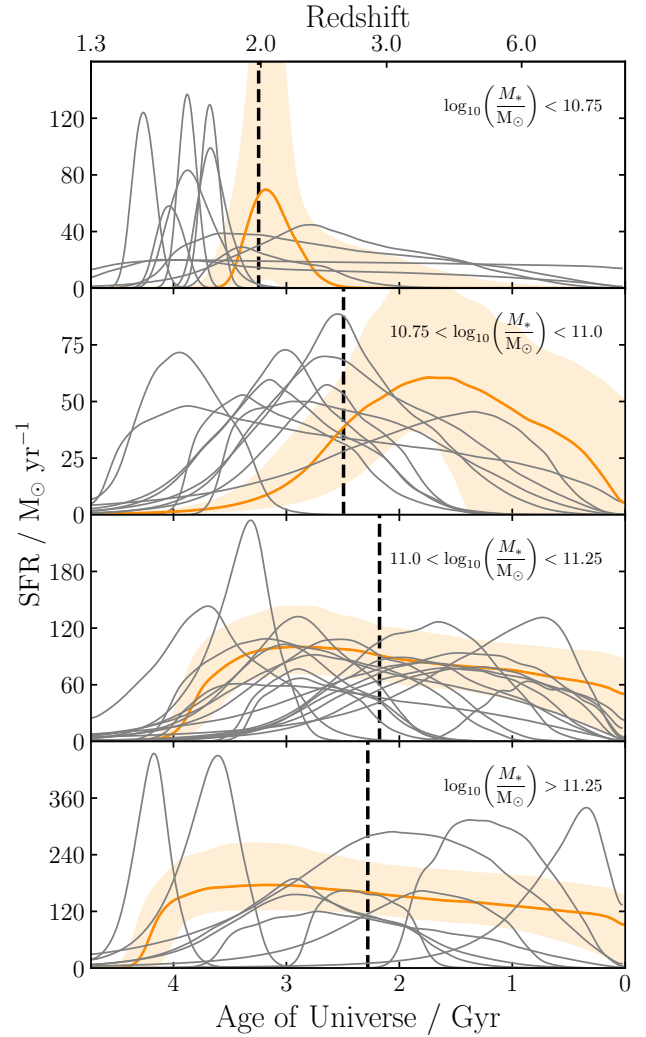
Figure 13. Posterior median SFHs for our quiescent sub-sample, divided into four bins in stellar mass. In each bin, a randomly selected SFH is highlighted, and the 16 th –84 th percentiles of the posterior are shaded to demonstrate the typical uncertainties. The dashed vertical lines show the mean formation times for galaxies in each bin, as described in Section 5.2 and shown in Fig. 3.
