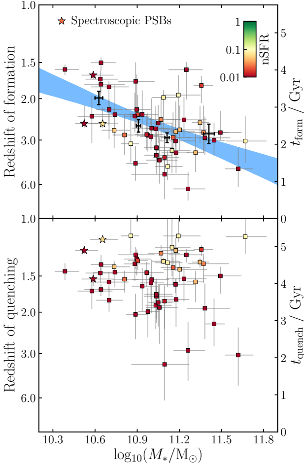
Figure 3. Redshifts of formation (top panel) and quenching (bottom panel) for our quiescent sub-sample. In the top panel the black errorbars show the mean time of formation in four stellar mass bins. The posterior distribution given in Equation 9 for the mean formation time as a function of stellar mass is shown in blue. Individual SFHs for these objects are shown in Fig. 13.
