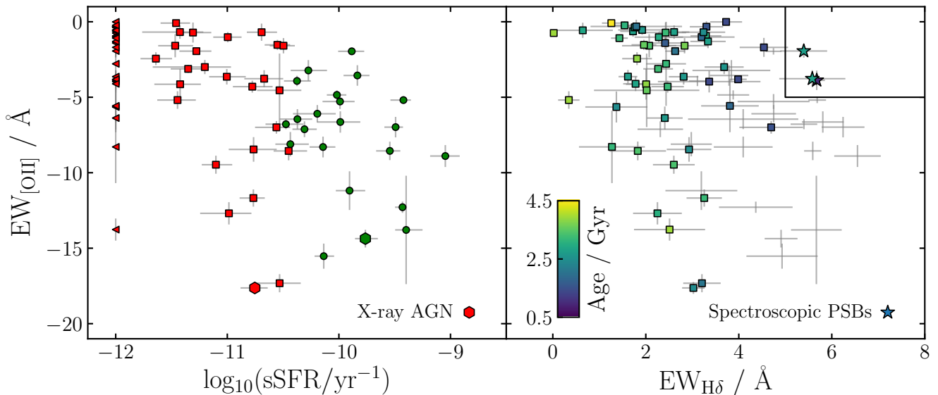
Figure 6. The distribution of [O II] emission in our sample. The left panel shows EW_{[O II]} vs sSFR: symbols and colours are as defined in Fig. 4, except for galaxies with \log_{10}(sSFR/\text{yr}^{-1}) < -12 , which are shown as triangles, indicating an upper limit. Additionally, objects detected in the Chandra seven megasecond catalogue of Luo et al. (2017) are shown as hexagons (see Section 5.7). The right panel shows the EW_{H\delta} vs EW_{[O II]} parameter space typically used to select post-starburst galaxies. Quiescent galaxies are coloured by mass-weighted age, green-valley galaxies are shown with gray errorbars. Commonly used spectroscopic PSB selection criteria are shown with solid lines (e.g. Tran et al. 2003; Maltby et al. 2016). Galaxies which meet these criteria are shown as stars (see Section 5.6).
