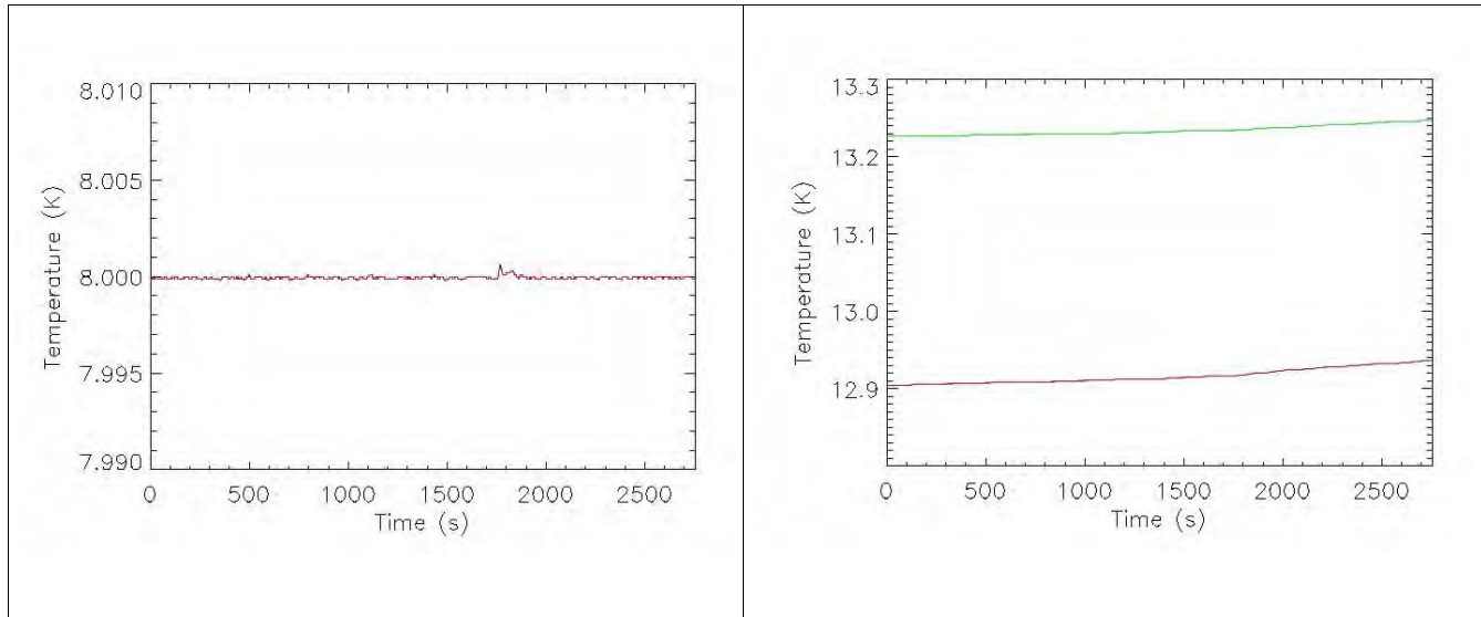
Figure -9: Left – Reference Load temperature behaviour during the RCA_THF test; right – SKY_TEMP probe (red) and SMON_TMP probe (green)
