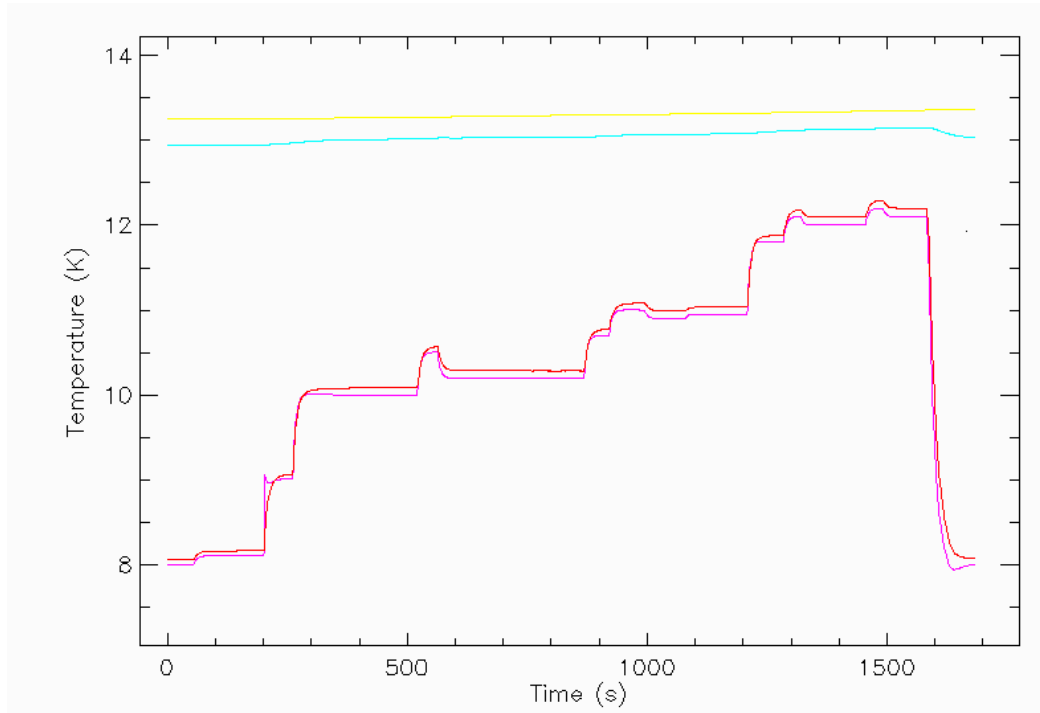
Figure 6-2: Temperature sensor output: yellow: SMON (sky Load Eccosorb pyramid tip); light blue: Tsky (Sky load control temperature); violet: RMON (Reference Load case); red Tref (Reference Load control).
