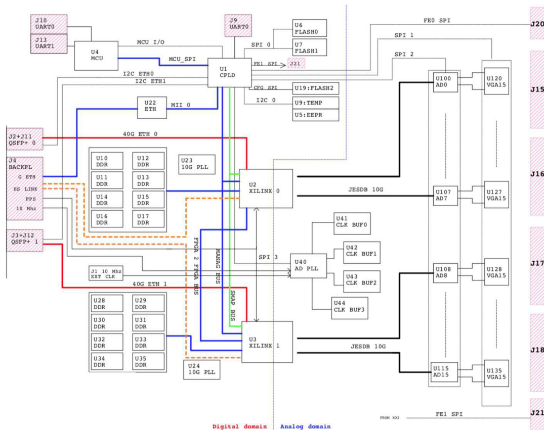
Figure 5. ITPM 1.6 ADU Schematic view, data processing flow reading from left to right.
