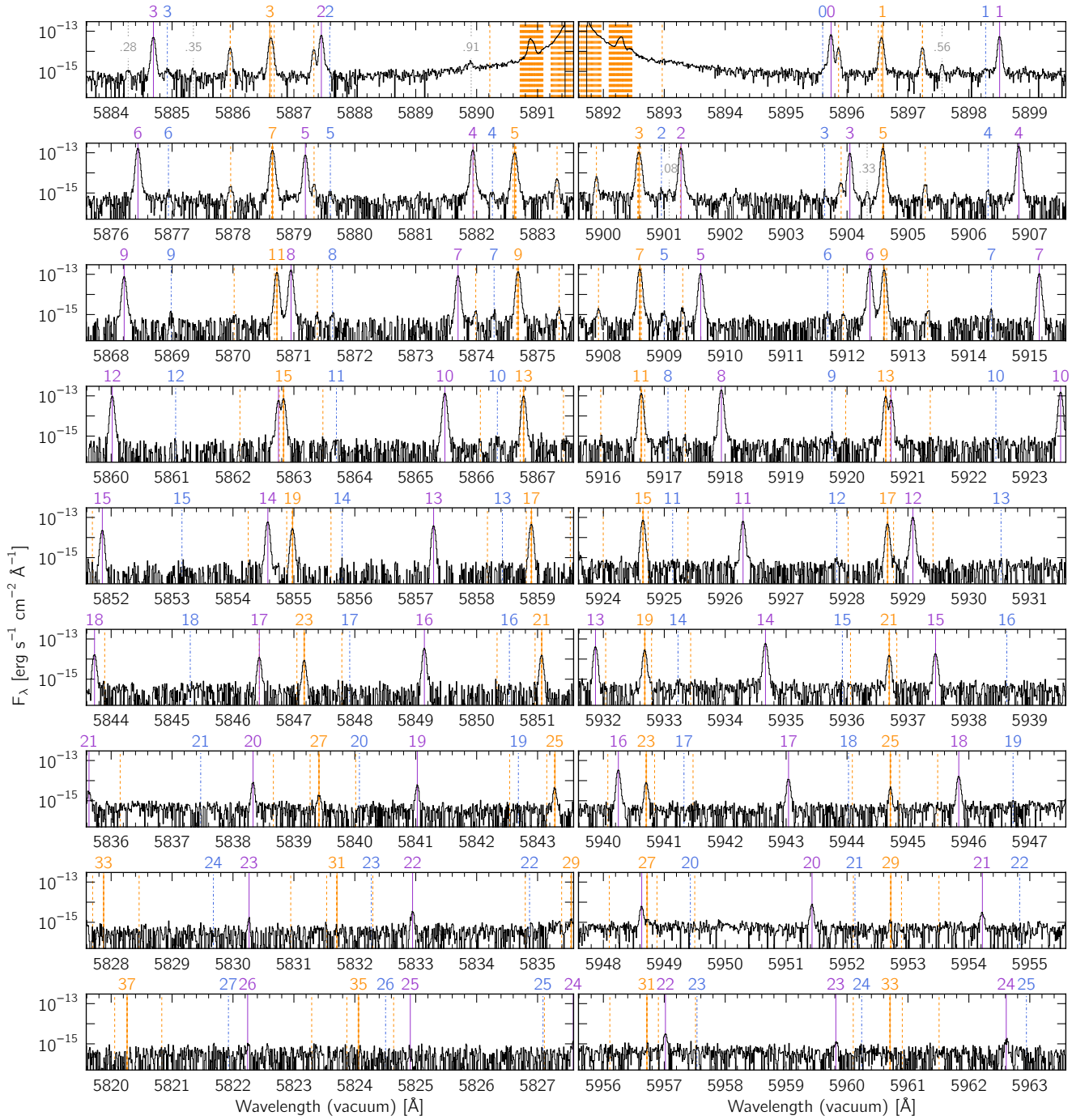
Figure 3. ESPRESSO spectrum of one 4LGSF up-link laser beam, focusing on the spectral regions containing pure rotational Raman lines. Each panel is 8 Å wide. For a given row, the left and right panels are equidistant from the main laser line at 5891.5912 Å (which is saturated). Pure rotational Raman lines, associated with the Stokes (right column) and anti-Stokes (left column) branches, are detected up to J = 27 for ^{16}\text{O}_2 , J = 24 for ^{14}\text{N}_2 , and J = 9 for ^{14}\text{N}^{15}\text{N} . Solid orange, solid purple, and dash-dotted blue vertical lines mark the theoretical position of the pure rotational Raman lines of ^{16}\text{O}_2 , ^{14}\text{N}_2 , and ^{14}\text{N}^{15}\text{N} (respectively), when treated as non-rigid singlet diatomic rotators. The molecular rotational quantum number J associated with each of these lines is indicated above them (only the ^{14}\text{N}_2 J = 11 anti-Stokes and J = 9, 19 Stokes lines are not tagged because of crowding). Dashed orange vertical lines, derived using a numerical model of ^{16}\text{O}_2 accounting for the non-zero electronic spin of its ground state, highlight the fine-splitting of the pure rotational lines for this molecule. The nature of 6 lines (tagged with dotted grey vertical lines and the first two decimals of their wavelength in the top panels) remains unknown at this time.
