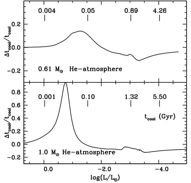
Figure 11. Same as Fig. 10 but for He-atmosphere models.
