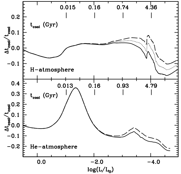
Figure 13. As Fig. 12, but for our new models calculated with Blouin et al. (2020) opacities.
