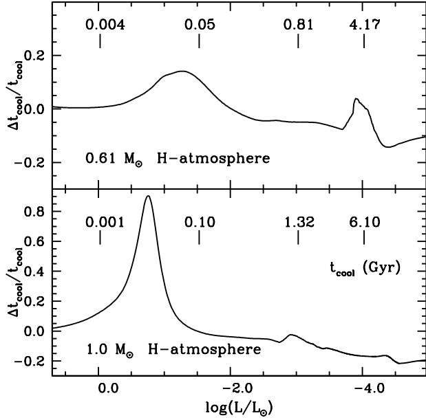
Figure 10. Relative difference of cooling times as a function of luminosity for our 0.61M_{\odot} and 1.0M_{\odot} H-atmosphere models with no Ne (corresponding to metal poor populations), calculated with Blouin et al. (2020) and Cassisi et al. (2007) opacities, respectively. A positive difference means that models computed with Blouin et al. (2020) opacities have longer cooling times. Some reference cooling ages from the calculations with Cassisi et al. (2007) opacities are marked.
