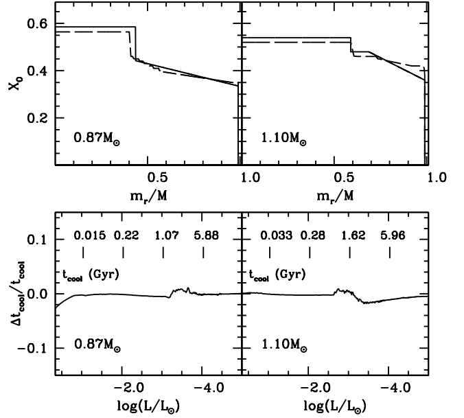
Figure 8. Upper panels: Pairs of oxygen abundance profiles (abundance in mass fraction) employed for the calculation of 0.87 and 1.1M_\odot H-atmosphere WD models. The dashed lines display our adopted reference profiles, whilst the solid lines correspond to the case of metal poor progenitors with Z=0.0002 (see text for details). Lower panels: Relative difference between the cooling times obtained using the CO stratification of the metal poor progenitor, and those obtained from the reference stratification, as a function of the luminosity. Selected cooling ages from the calculations with the reference profiles are marked.
