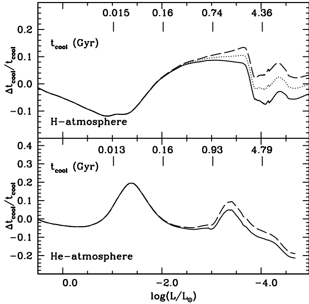
Figure 12. Relative difference of cooling times (in Gyr) as a function of luminosity with respect to the 0.61M_{\odot} H-atmosphere calculations from S10 of, respectively, our new 0.61M_{\odot} H-atmosphere calculations with Cassisi et al. (2007) opacities without Ne diffusion (solid line), with Ne diffusion and Z=0.017 Ne abundance (dotted line), with Ne diffusion and Z=0.04 Ne abundance (dashed line). Some reference ages from S10 calculations are marked.
