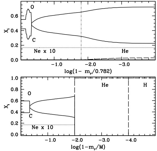
Figure 3. Upper panel: Stratification of the C, O, Ne, H and He abundances in the inner layers of a 3.1M_{\odot} asymptotic giant branch model with initial chemical composition about solar. Abundances are given in mass fractions (for the sake of clarity the Ne mass fraction is increased by a factor of 10) and m_r is the mass enclosed within a radial distance r from the centre of the model. The stratification is taken around the time the He-free core (whose boundary is marked by the thin dash-dotted vertical line) has reached 0.77M_{\odot} , the final WD mass prescribed by the Cummings et al. (2018) IFMR (see text for details). Lower panel: Initial chemical stratification adopted for the corresponding 0.77M_{\odot} H-atmosphere WD model ( M is the total mass of the model).
