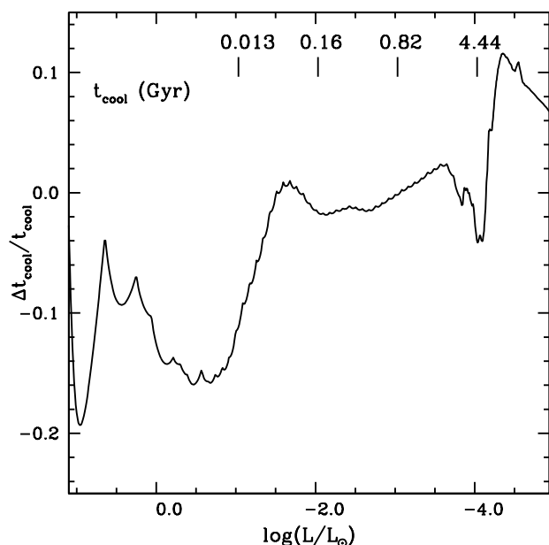
Figure 14. Relative difference of the cooling times (zeroed at \log(L/L_\odot)=1.1 ) as a function of luminosity between our 0.61M_\odot H-atmosphere cooling track with Ne abundance from a Z=0.017 progenitor, and a 0.6M_\odot H-atmosphere track with solar metallicity progenitor from Camisassa et al. (2016). Some reference cooling ages from Camisassa et al. (2016) calculations are marked.
