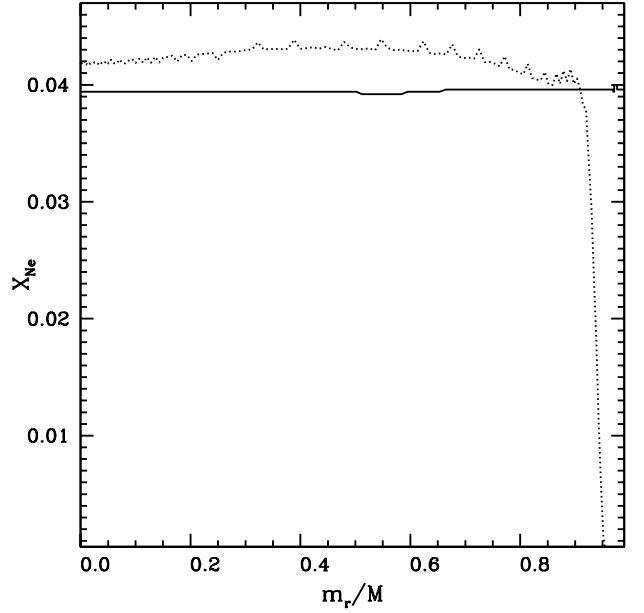
Figure 5. Initial (solid line) and final (dotted line) Ne abundance stratification (abundance in mass fraction) of a 0.61 M_{\odot} H-atmosphere model from a progenitor with Z=0.04 (see text for details).
