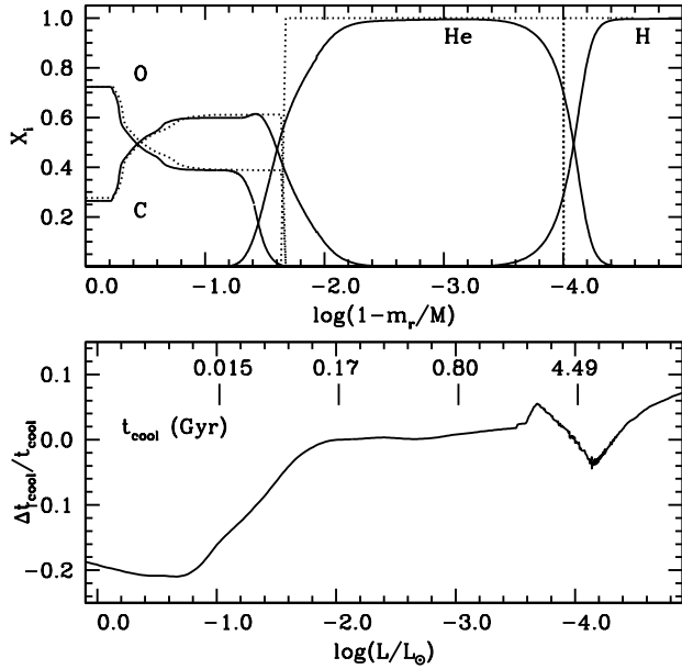
Figure 9. Upper panel: Solid lines display the C, O, He and H stratification (abundances in mass fraction) at the beginning of the cooling sequence of 0.61M_\odot H-atmosphere models by Renedo et al. (2010). The dotted lines display our adopted core stratification with CO profile determined as described in Sect. 2.2, plus stratified pure-H and He envelopes which match the total mass of H and He of Renedo et al. (2010) models. Lower panel: Relative difference of cooling times as a function of luminosity with respect to Renedo et al. (2010) calculations, of 0.61M_\odot models calculated using the stratification with pure-He and H envelopes shown in the upper panel (dotted line – see text for details). Some reference cooling ages from Renedo et al. (2010) calculations are marked.
