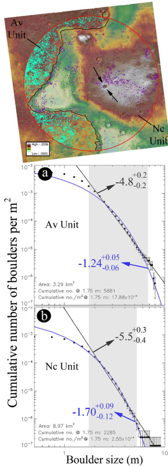
438 Fig. 8: Uppermost panel: HiRISE DTM showing the spatial distribution of all boulders detected, grouped according to 439 the geologic units. Those located on the Av unit are shown in light-blue, whilst those on the Nc unit are shown in 440 purple. Black arrows in the top panel show the location of the crater referred to in the text. The cumulative SFDs for 441 both regions are presented in a) and b). The data were fitted with a linear regression (solid black line) and with 442 an exponential curve (solid blue curve) performed on data between 1.75 and 6.75 m on the Av unit and between 443 1.75 and 5.25 on the Nc unit (the fitting ranges are highlighted in grey) as shown in Fig. 7. 444 445
