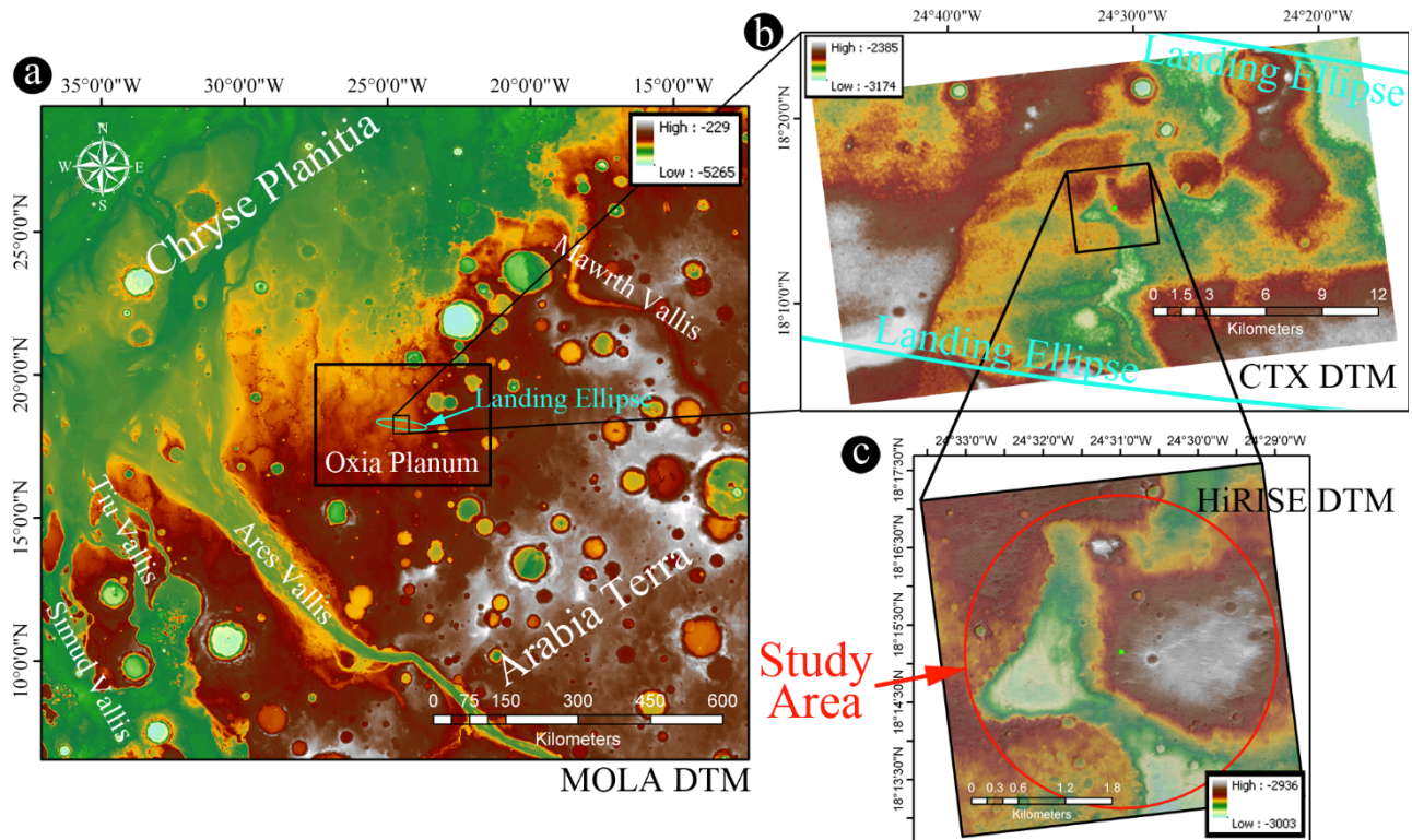
Fig. 1. (a) MOLA context map showing the location of the Oxa Planum region (black rectangle) and the landing ellipse for the ExoMars 2020 mission. The primary landing ellipse (light blue) is 104 \times 19 km wide, is oriented with an azimuth angle of 97^{\circ}30' and its center is located at -24^{\circ}30'59''E and 18^{\circ}15'9''N . (b) CTX DTM located at the center of the ExoMars landing ellipse (light blue) with a spatial scale of 22 m/pixel. (c) HiRISE DTM covering the center of the Oxa Planum proposed landing ellipse. The spatial scale is 1 m/pixel. The red circle indicated by a red arrow is the study area where the boulder identification was performed. In (b) and (c) the green dot represents the center of the proposed landing ellipse.
