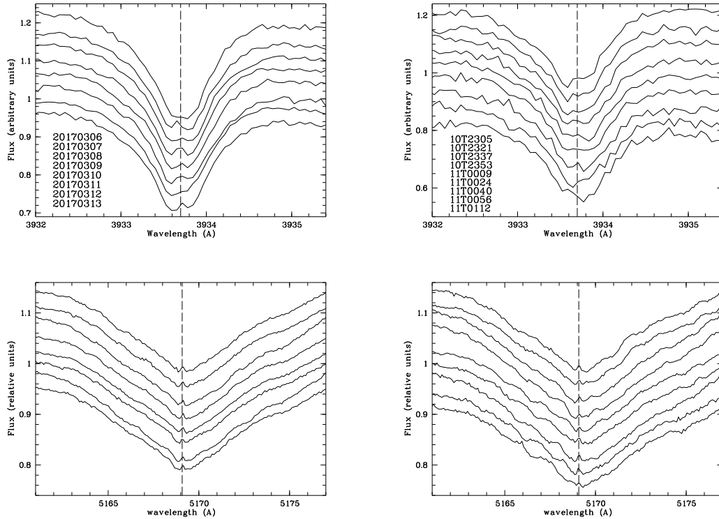
Fig. B.1. Left: Nightly median of Ca II K and Fe II 5169 Å. Dates are indicated in the labels. Right: Some consecutive spectra taken during the night 2017-03-10/11. Exposure time of each spectrum is 15 minutes. The resolution of the Ca II spectra is 0.0625 Å/pixel, while for Fe II is 0.0938 Å/pixel. Ca II K shows variability from night to night as well as irregular short timescale variability in individual nights. The central emission is seen in some of the nights, and both blue- and red-shifted minima change their relative strength. With respect to the Fe II line the central emission is present in all nights but the variability is less pronounced than the one in the K line and no correlation is seen.
