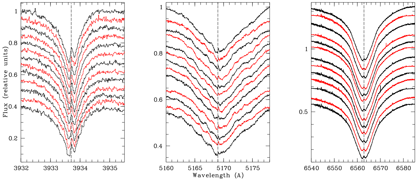
Fig. 10. Ca II K ( left panel , resolution 0.016 \text{ Å pixel}^{-1} ), Fe II 5169 Å ( middle , resolution 0.03 \text{ Å pixel}^{-1} ), H \alpha ( right , resolution 0.01 \text{ Å pixel}^{-1} ). Spectra were taken with HARPS-N during the night of 2019-01-29/30; each spectrum is 15 min apart starting 01h01m UT (first spectrum at the top) and finishing 04h07m UT (last spectrum at the bottom). The dashed line corresponds to a velocity of 3 \text{ km s}^{-1} .
