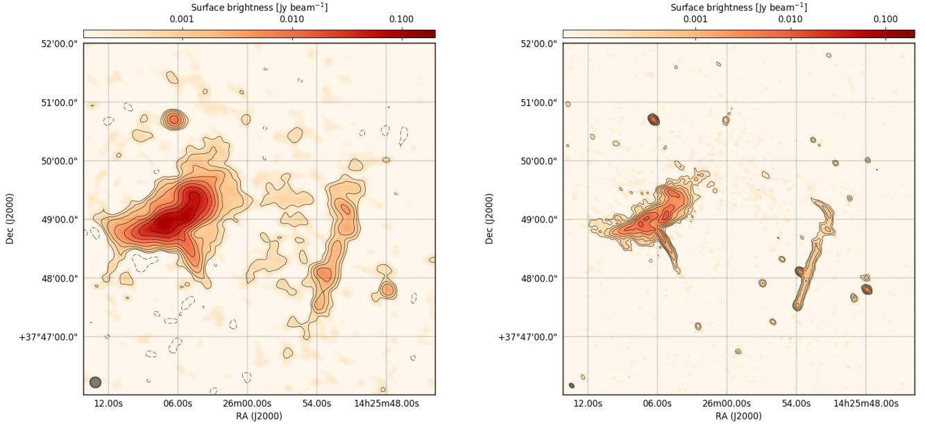
Fig. 3. Full-resolution GMRT images of Abell 1914 at 325 MHz ( left panel : 11'' \times 10'' ) and 610 MHz ( right panel : 5'' \times 4'' ). The black contours and dashed lines indicate the significance of the radio emission at (1, 2, 4, \dots) \times 3 \times \sigma_{\text{GMRT},325/610} and -3 \times \sigma_{\text{GMRT},325/610} levels, respectively, where \sigma_{\text{GMRT},325} = 130 \mu\text{Jy beam}^{-1} and \sigma_{\text{GMRT},610} = 40 \mu\text{Jy beam}^{-1} .
