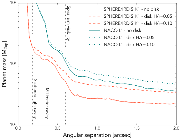
Fig. 14. Planet mass detection limits ( 5\sigma ) for the IRDIS K1-band and NaCo L'-band images, both with the effect of attenuation of a planet emitted flux by protoplanetary dust (dashed and dash-dotted curves, see text) compared to the case where the attenuation by protoplanetary dust is neglected (solid curves, see Fig. 12).
