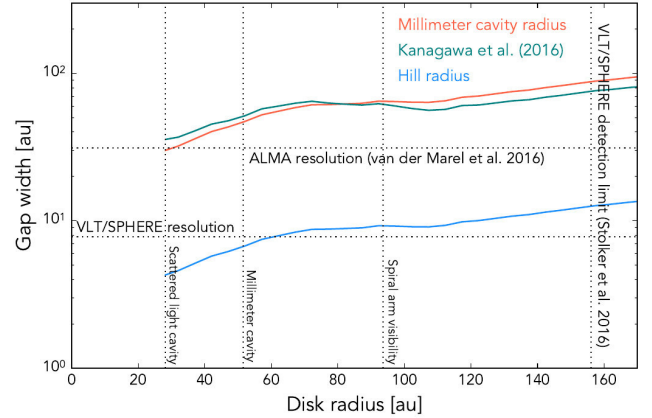
Fig. 15. Gap widths in the gas and large dust grains for the K1-band planet mass limits, corrected for the attenuation by the dust (see Fig. 14). The gas gap widths are assumed to be valid for the small dust grains, which are probed by the SPHERE data. The Hill radius gives a first-order estimate of a gap width in the gas (blue). We also considered the empirical relation from the hydrodynamical simulations of Kanagawa et al. (2016; green curve, see text for details). The cavity radius in the large dust grains (red) is assumed to be \sim 7 R_H following the work of Pinilla et al. (2012).
