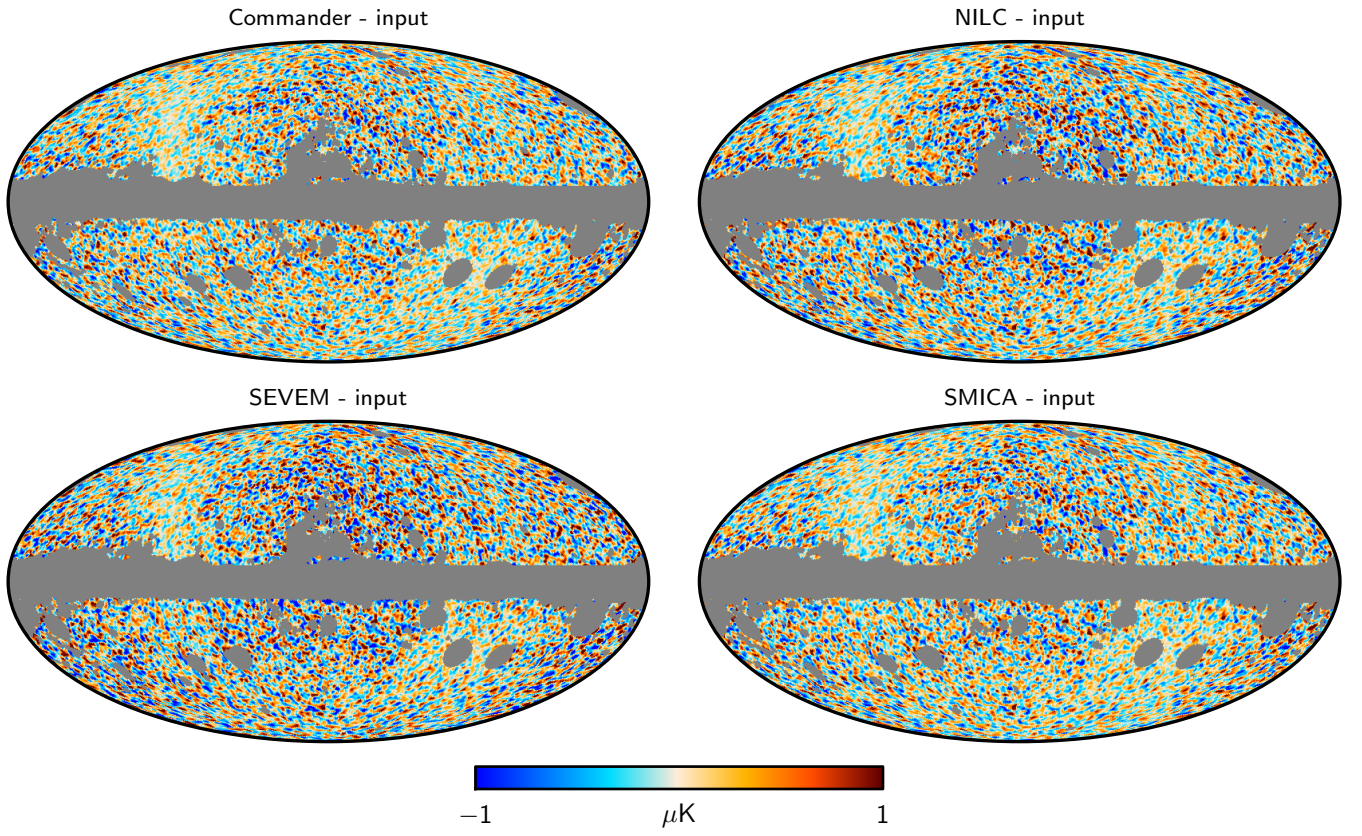
Fig. 11. Difference between output and input CMB Q maps from FFP8 simulations. Smoothing and downgrading as in Figs. 9 and 10.
