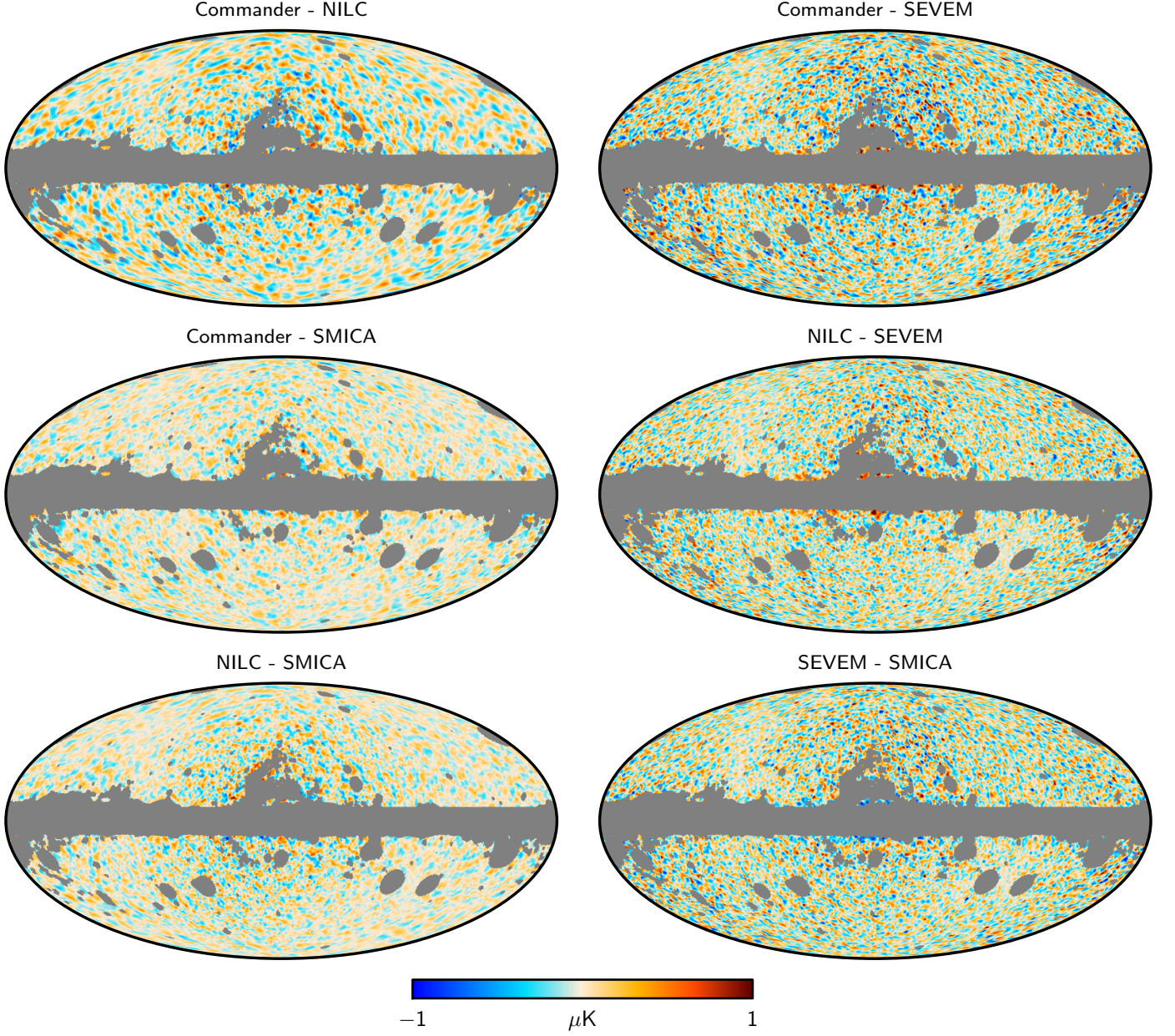
Fig. E.3. Pairwise difference maps between U maps obtained on FFP8 simulations. Smoothing and degrading as in Figs. 4,9.
