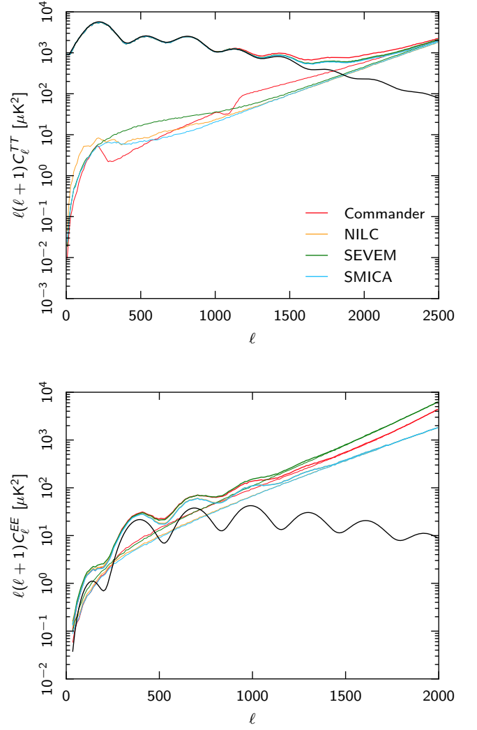
Fig. E.6. Power spectra of the foreground cleaned CMB maps from FFP8 simulations. Top: TT power spectra evaluated using the FFP8-UT74 mask. Bottom: EE power spectra evaluated using the FFP8-UP76 mask. Thick lines show the spectra of signal plus noise estimated from the half-mission half-sum maps; thin lines show the noise levels from half-mission half-difference maps. The black line shows the input spectrum.
