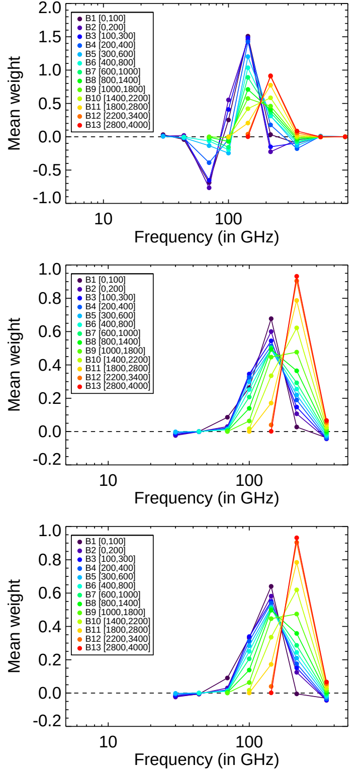
Fig. B.2. Full-sky average of needlet weights for different frequency channels and needlet bands. From top to bottom, the panels show results for temperature, E , and B modes.
