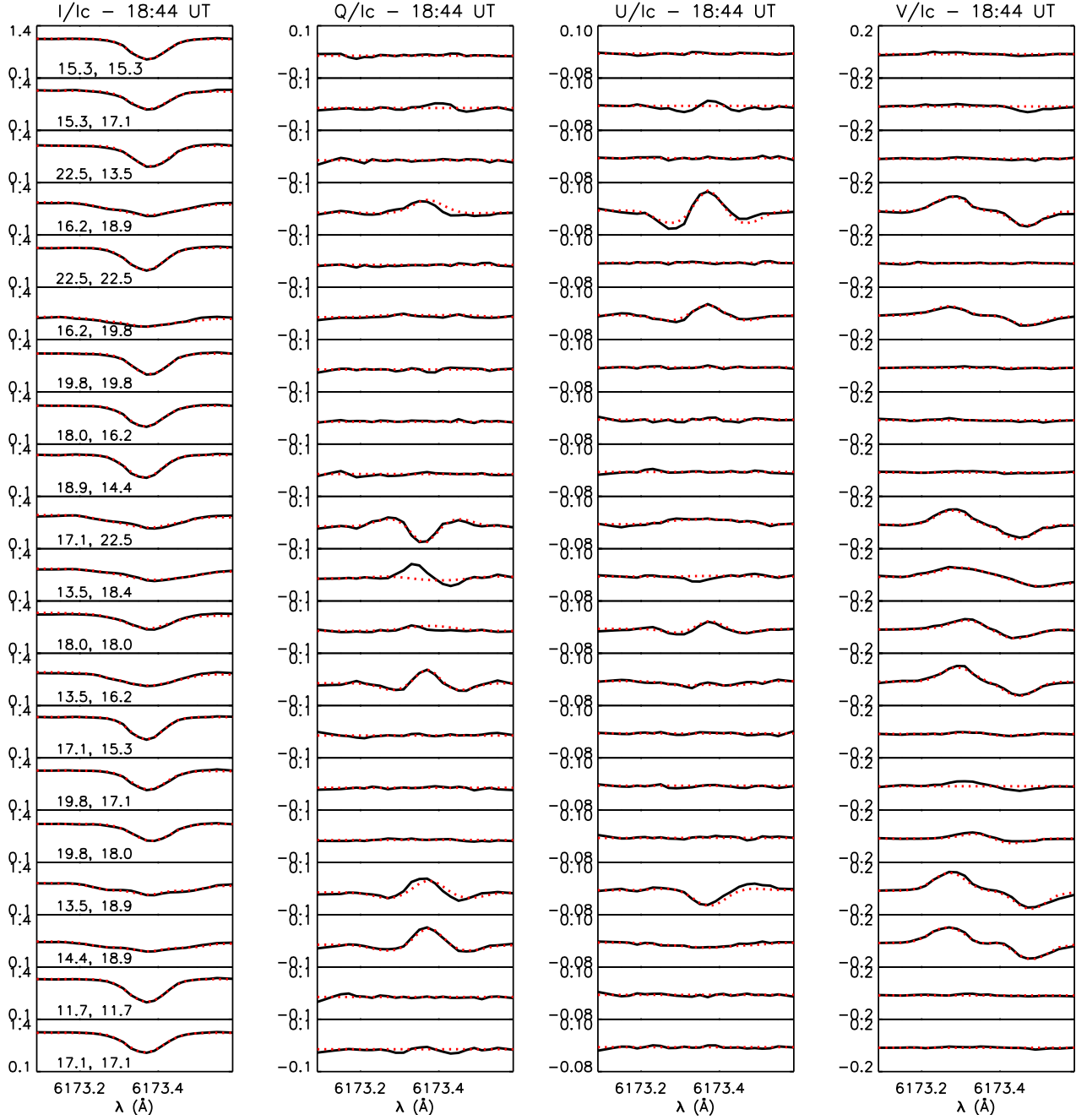
Fig. A.6. As in Fig. A.2 but for the data taken at 18:44 UT (stage (e) of the pore formation shown in Fig. A.1). Values of the stray-light fraction, LOS magnetic strength (kG), field inclination and azimuth (degree), and LOS velocity ( \text{km s}^{-1} ) derived from our data analysis (at optical depth \log \tau_{500} = 1 ) at the same positions of the shown profiles are listed in Table A.5; the values are cut at 2 decimal digits.
