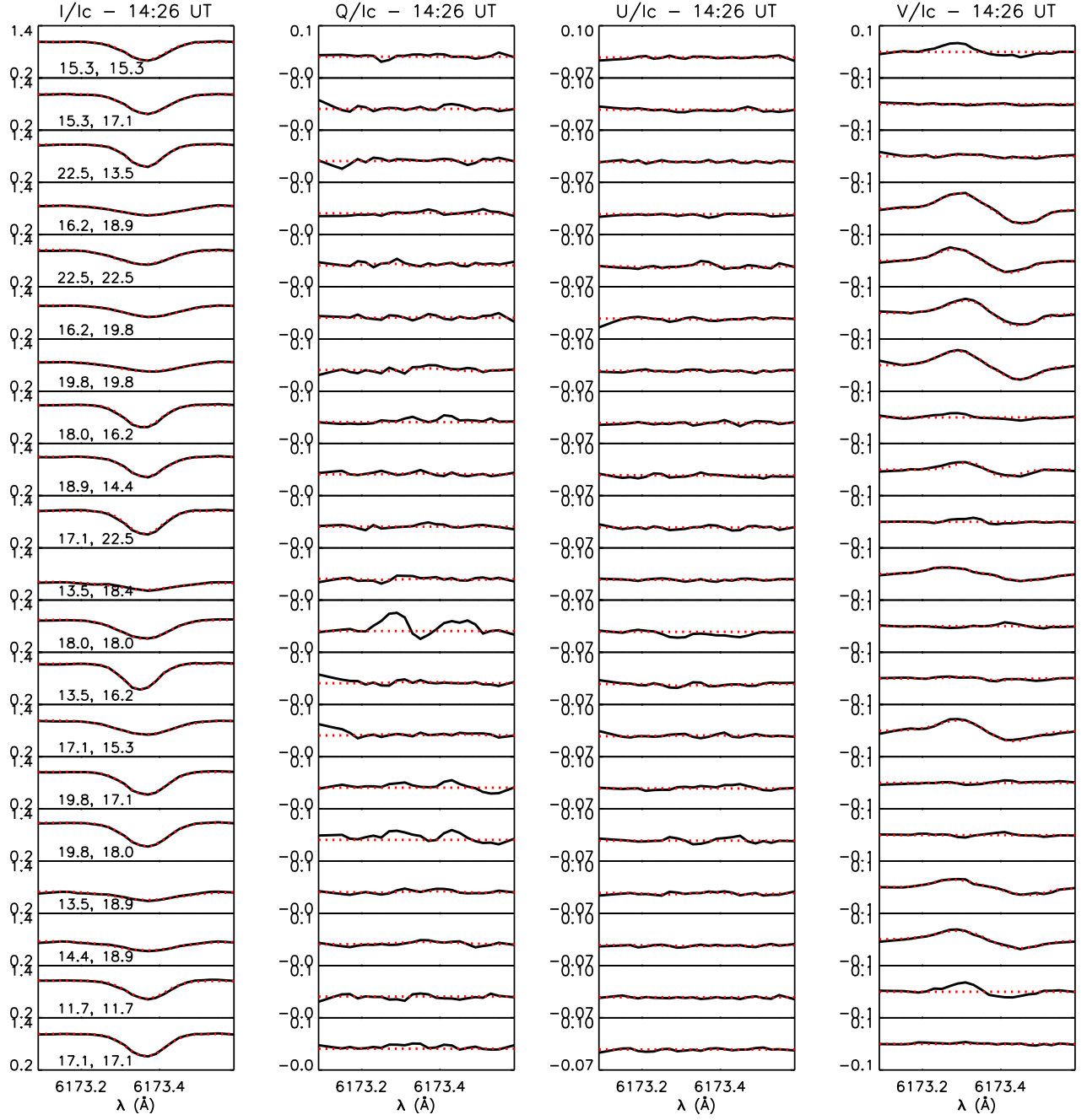
Fig. A.3. As in Fig. A.2 but for the data taken at 14:26 UT (stage (b) of the pore formation shown in Fig. A.1). Values of the stray-light fraction, LOS magnetic strength (kG), field inclination and azimuth (degree), and LOS velocity (km s -1 ) derived from our data analysis (at optical depth \log\tau_{500} = 1 ) at the same positions of the shown profiles are listed in Table A.2; the values are cut at 2 decimal digits.
