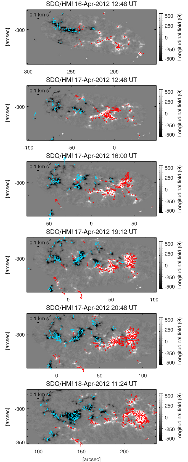
Fig. 4. Examples of the photospheric horizontal velocity maps derived from the SDO/HMI SHARP data taken from Apr. 16, 2012, 12:48 UT to Apr. 18, 2012, 11:24 UT, which is from 24 h before the start of the pore formation to several hour after. The arrows indicate the horizontal velocity; red (light blue) shows the leading (trailing), positive (negative) polarity. In all panels but the first , the studied pore coincides with the largest size structure in the leading region. The magnetic field in the background magnetogram is shown in the range of values specified in the colour bars. The full temporal evolution of all computed maps is shown in a movie available online .
