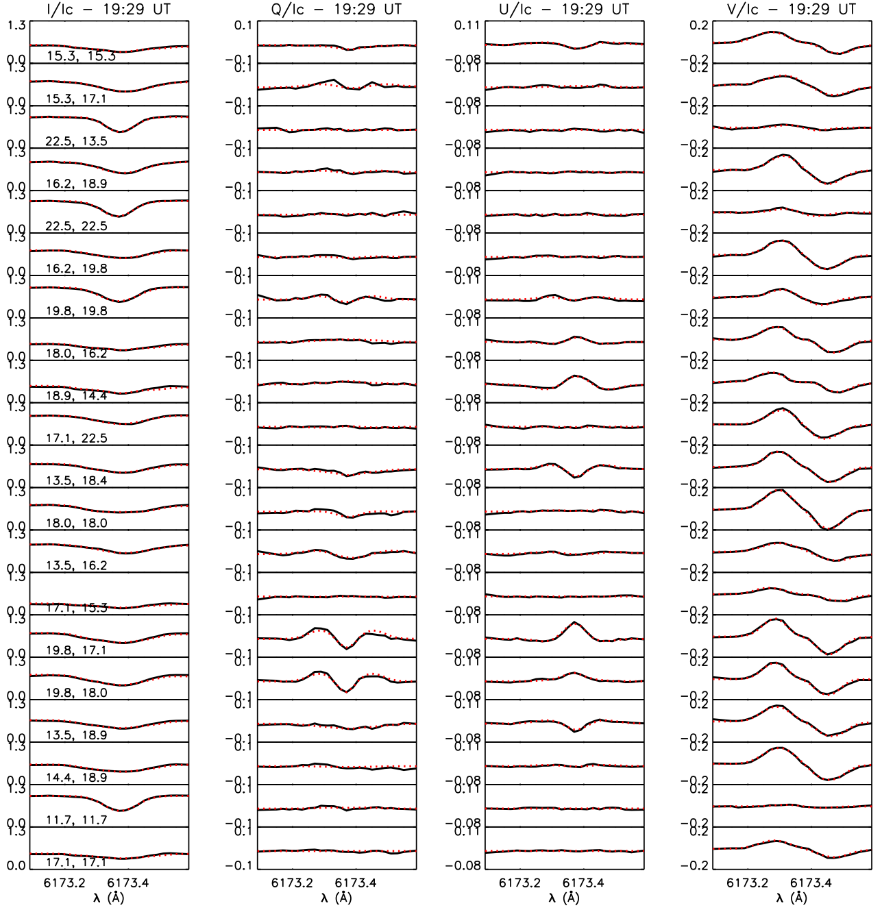
Fig. A.7. As in Fig. A.2 but for the data taken at 19:29 UT (stage (f) of the pore formation shown in Fig. A.1). Values of the stray-light fraction, LOS magnetic strength (kG), field inclination and azimuth (degree), and LOS velocity ( \text{km s}^{-1} ) derived from our data analysis (at optical depth \log \tau_{500} = 1 ) at the same positions of the shown profiles are listed in Table A.6; the values are cut at 2 decimal digits.
