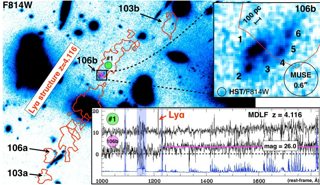
Fig. 7. Ly \alpha nebulae (red contours at 2\sigma level) including images 106(a,b) and 103(a,b), belonging to the same physical structure at z = 4.116 , are shown in the main panel (HST ACS/F814W band). In the top-right inset, the lensed galaxy 106b broken in six clumps is shown; the smaller ones (2–6) have intrinsic UV magnitude \approx 30.5\text{--}31 (corresponding to M_{\text{UV}} \approx -15 ) and intrinsic sizes of the order of (or smaller than) 100 pc along the tangential stretch, as indicated by the ruler. The bottom inset shows two one-dimensional spectra extracted from the MDLF. One is on galaxy 106b (within a circular aperture of 1.2'' diameter, see magenta circle). We note the ultraviolet continuum of 106b with F814W = 26.01 \pm 0.03 is well-detected (magenta line) above the zero level (black dashed line), and its continuum-break confirmed at z = 4.116 . The top spectrum is extracted from a nearby region showing Ly \alpha emission without HST counterpart (green circle with 1.2'' diameter, labeled as #1), vertically shifted at position 10 for illustrative purposes. The error spectrum is shown in blue at the bottom to highlight the location of the sky emission lines. The shaded band marks the wavelength region affected by the GLAO sodium-based laser.
