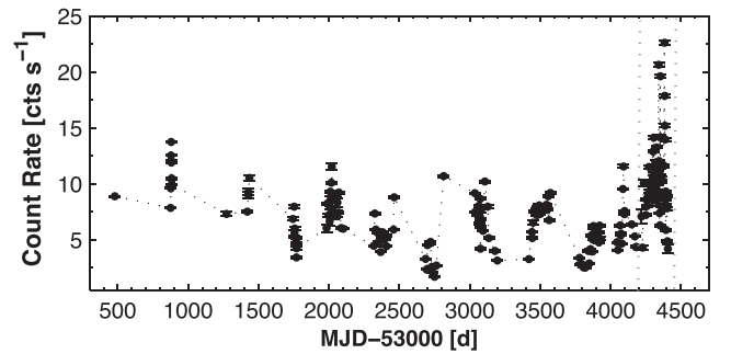
Figure 1. Long-term 0.3–10 keV light curve of 1ES 1959+650 from the Swift –XRT observations performed between 2005 April 19 and 2016 January 19. Its part, corresponding the campaign starting since 2015 August 1, is included within vertical dashed lines.
